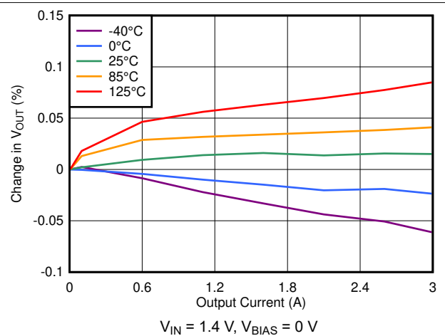
6-26. Load Regulation With Bias
