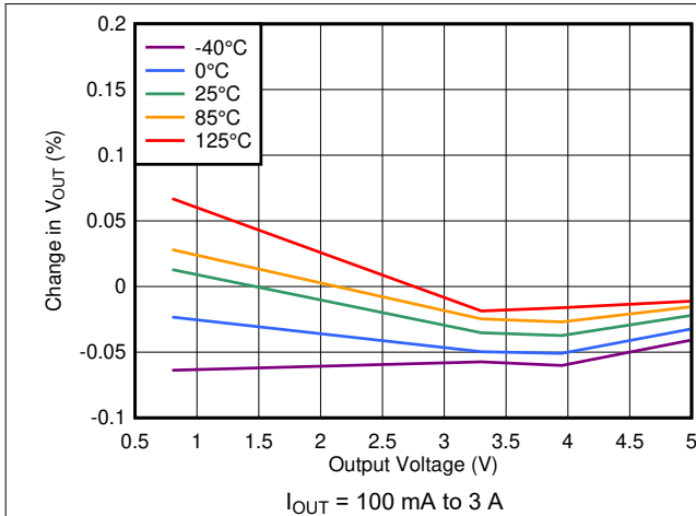
6-25. Load Regulation vs Output Voltage
