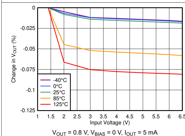
6-29. Line Regulation Without Bias
