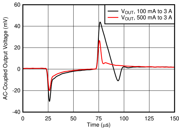
6-19. Load Transient vs Time and DC Load ( V_{OUT} = 0.9\text{ V} )
