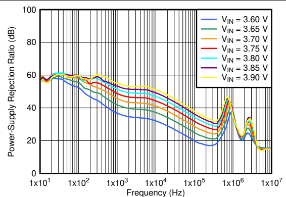
6-4. PSRR vs Frequency and V_{IN}
