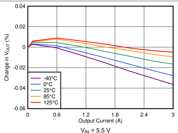
6-28. Load Regulation (5-V Output)
