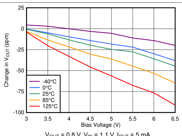
6-30. Line Regulation Without Bias
