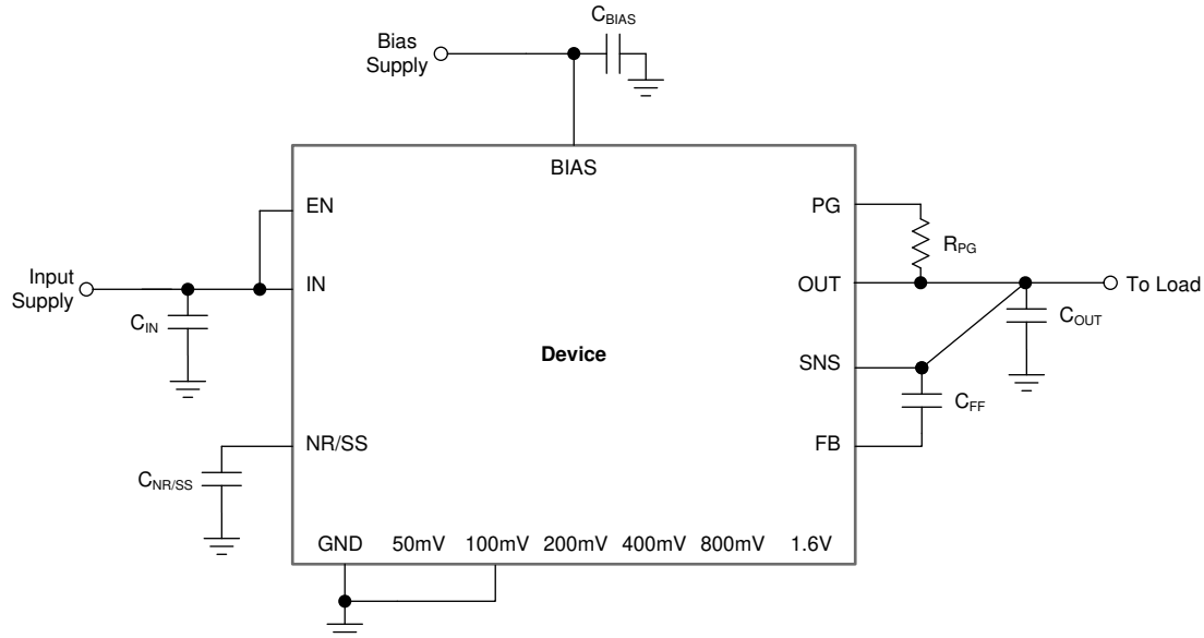
Figure 8-20. Typical Application
