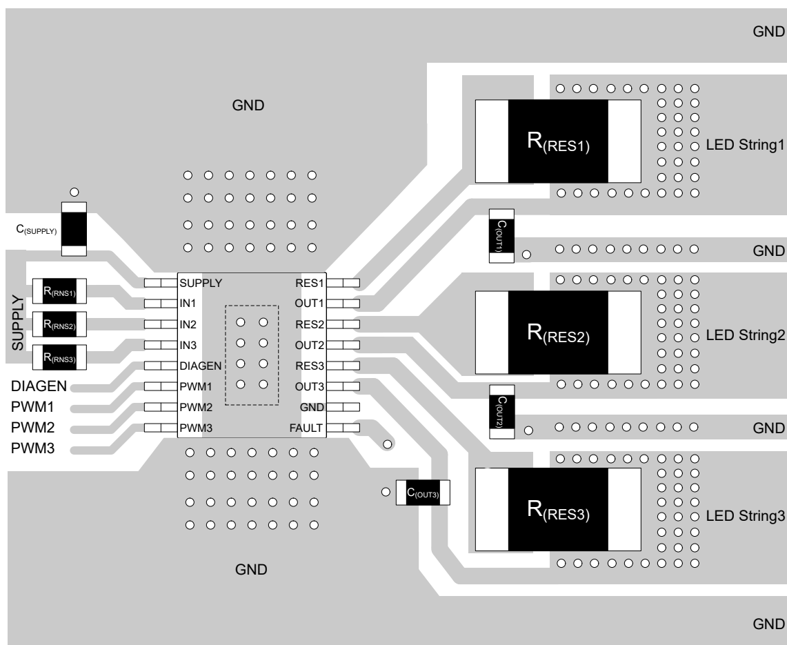
FIG 10-1. TPS92623-Q1 Example Layout Diagram
