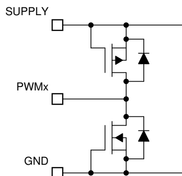
7-8. PWMx Pins
