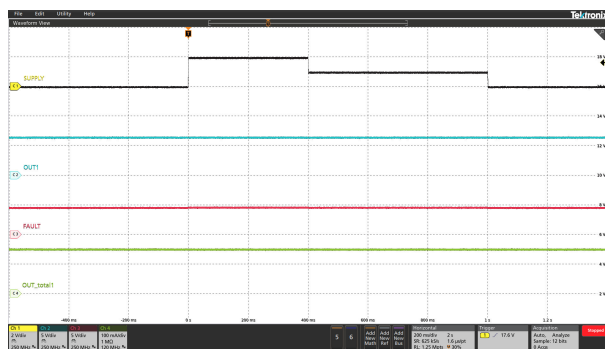
6-19. Transient Overvoltage
