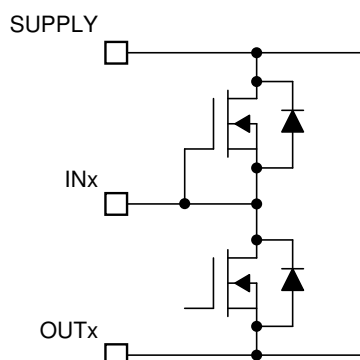
7-13. INx Pins
