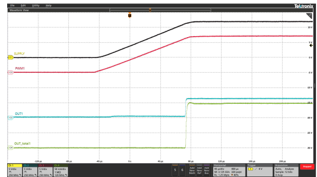
FIG 6-8. Output Current Distribution vs Supply Voltage
