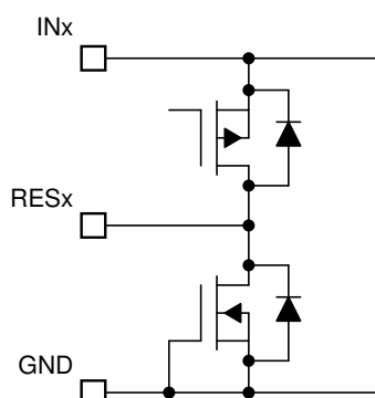
7-12. RESx Pins
