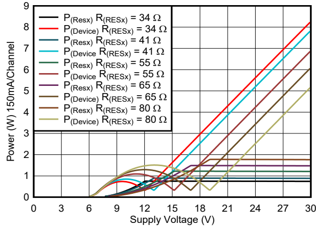
FIG 6-7. Power Dissipation vs Supply Voltage
