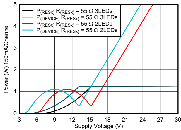
FIG 6-9. Power Dissipation vs Supply Voltage
