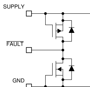
7-10. FAULT Pin
