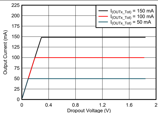
Figure 6-4. Output Current vs Dropout Voltage
