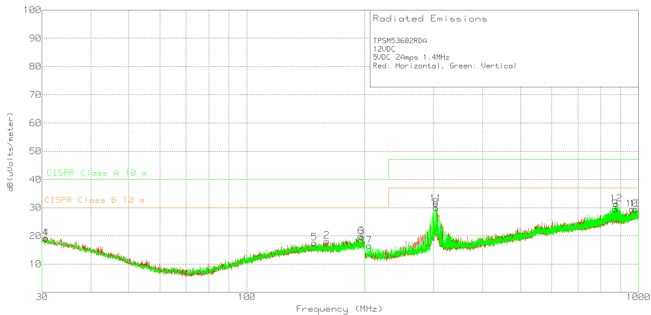
10-6. Radiated Emissions 12-V Input, 5-V Output, 2-A Load
