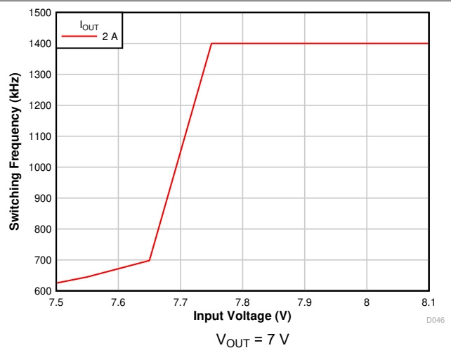
7-12. Frequency Foldback
