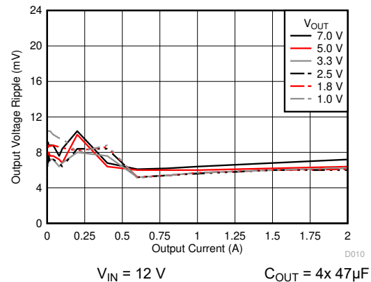
Figure 6-9. Voltage Ripple versus Output Current
