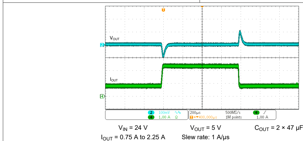
8-4. Transient Response
