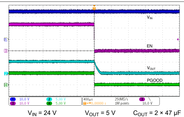
8-3. Enable Turn-OFF
