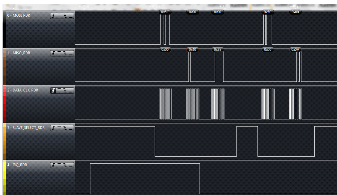
FIG 6-24. Read IRQ Status Register After Inventory Command
