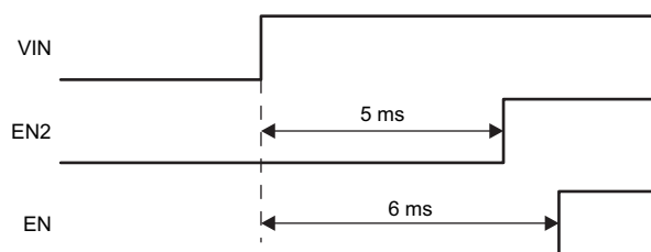
FIG 6-4. Nominal Start-up Sequence Using Parallel (MCU Controls EN2)
