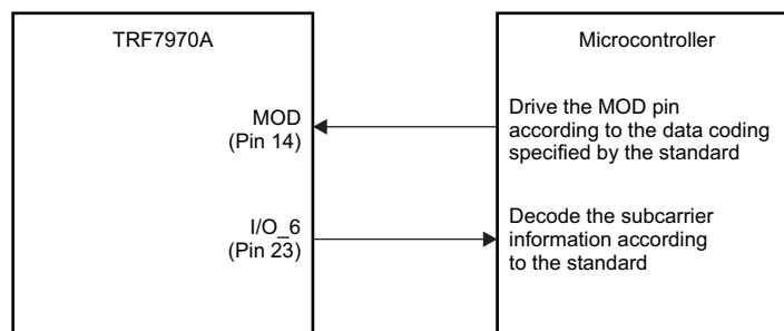
☒ 6-29. Direct Control Signals
