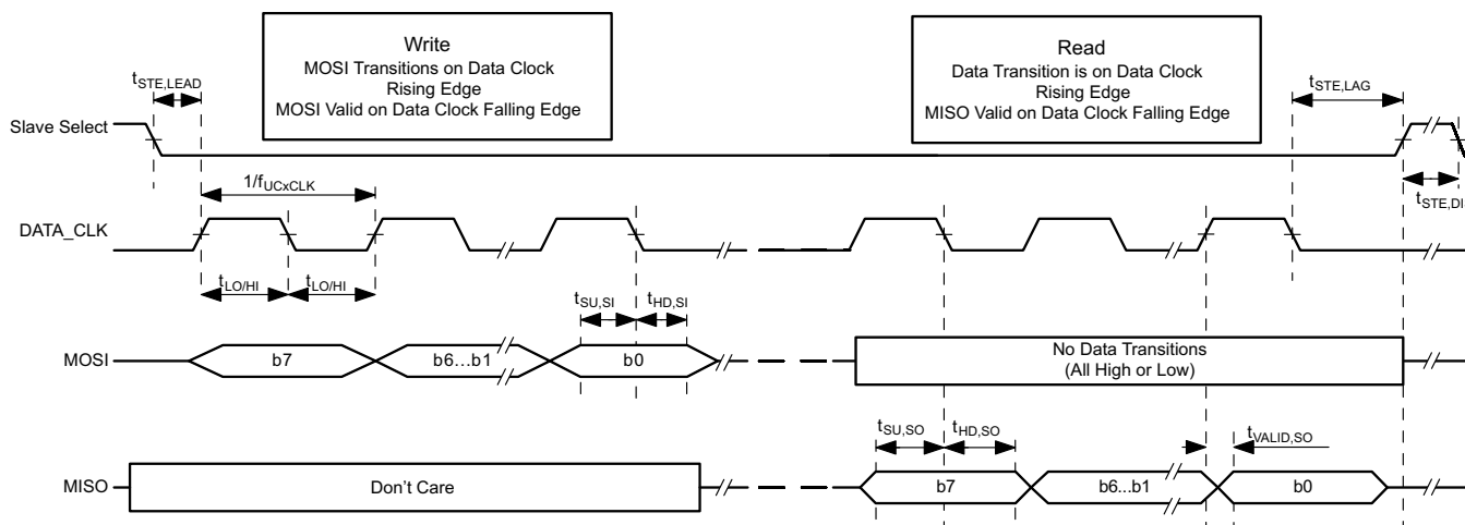
FIG 6-19. SPI With Slave Select Timing Diagram
