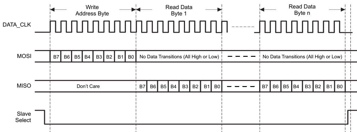
FIG 6-20. Continuous Read Operation Using SPI With Slave Select
