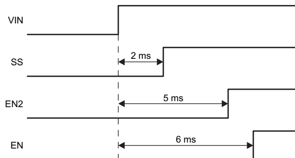
FIG 6-3. Nominal Start-up Sequence Using SPI With SS (MCU Controls EN2)
