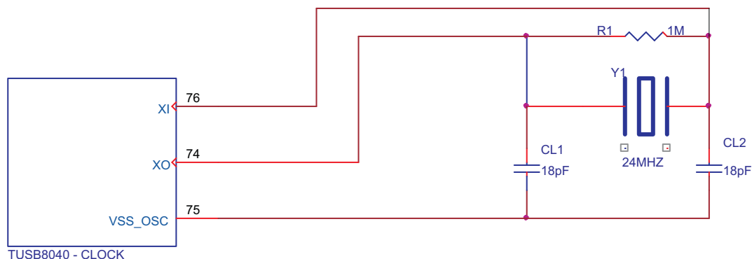
Figure 4-1. TUSB8040 Clock
