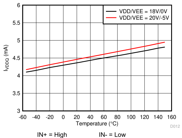
図 6-9. I_{VDDQ} Supply Current vs Temperature
