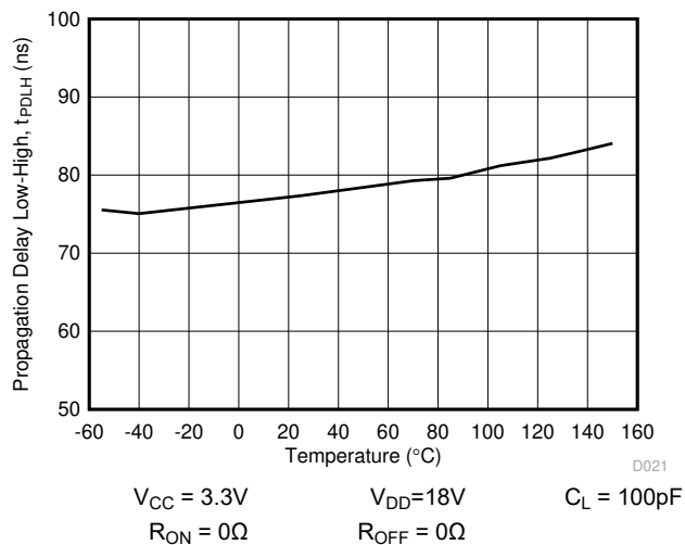
図 6-14. Propagation Delay t_{PDLH} vs Temperature
