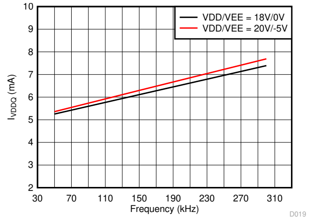
図 6-11. I_{VDDQ} Supply Current vs Input Frequency
