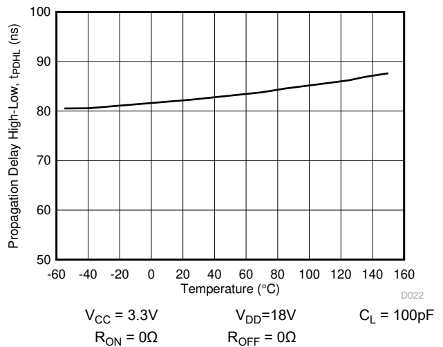
図 6-15. Propagation Delay t_{PDLH} vs Temperature
