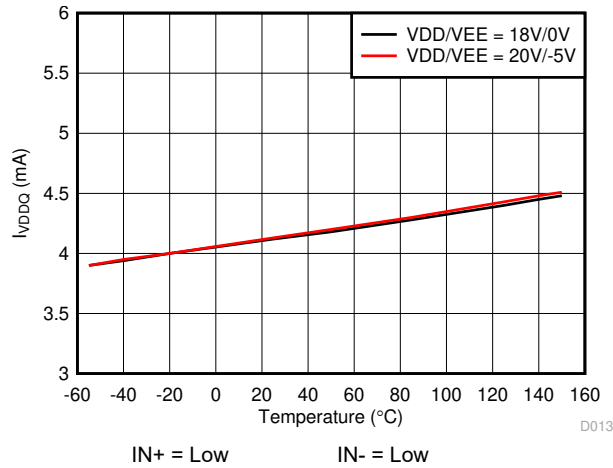
図 6-10. I_{VDDQ} Supply Current vs Temperature
