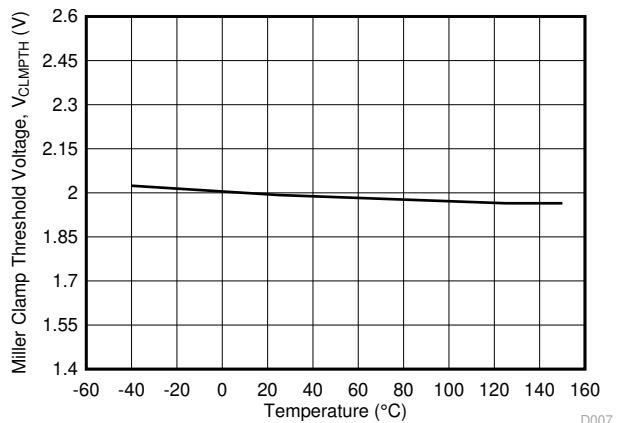
图 6-21. V_{CLMPH} Miller Clamp Threshold Voltage vs Temperature
