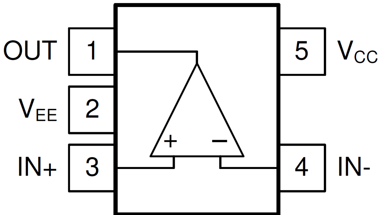
Figure 4-1. Pin Diagram (DCK and DBV) Package
