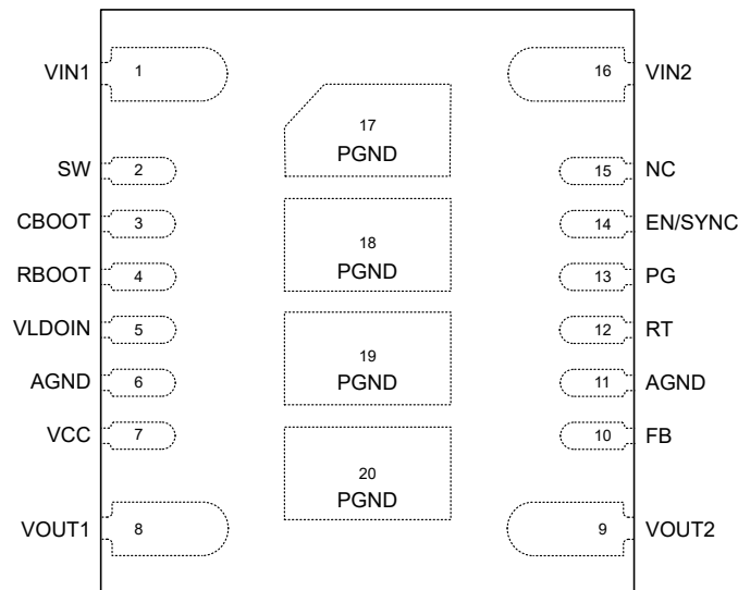
Figure 4-1. Pin Diagram
