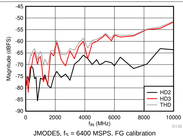
Figure 9. HD2, HD3, THD vs Input Frequency
