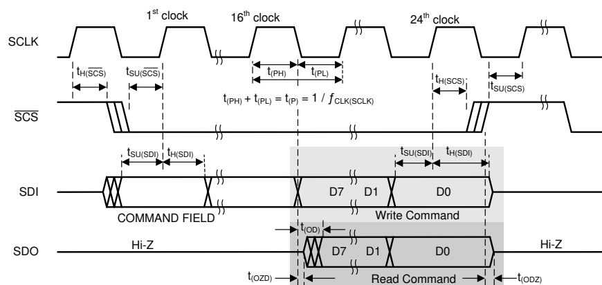
3. Serial Interface Timing
