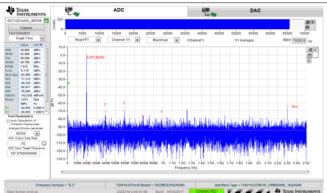
162. 200-MHz, Sine-Wave Frequency Domain (FFT) for 5-GSPS, Single-Channel Oscilloscope
