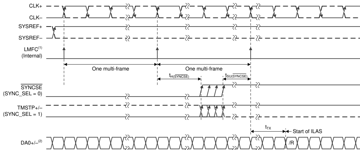
✎ 1. ADC Timing Diagram
