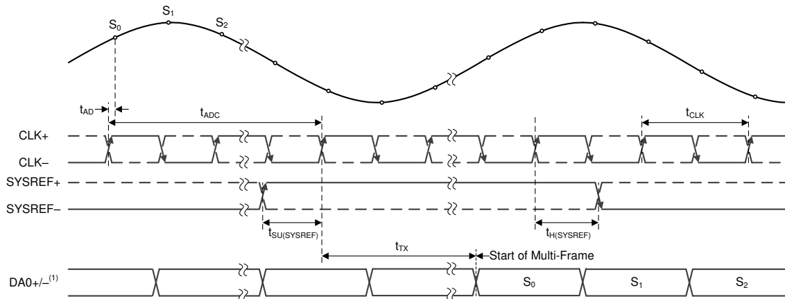
✎ 1. ADC Timing Diagram
