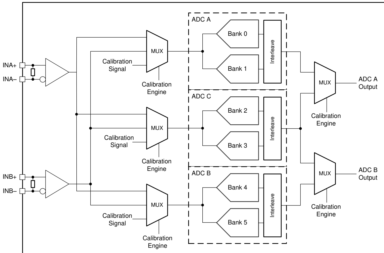
FIG 68. ADC08DJ3200 Calibration System Block Diagram
