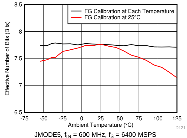
Figure 35. ENOB vs Temperature and Calibration Type
