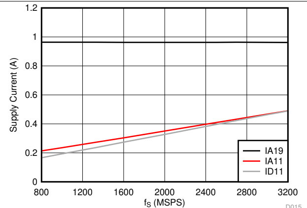
Figure 43. Supply Current vs Sampling Rate
