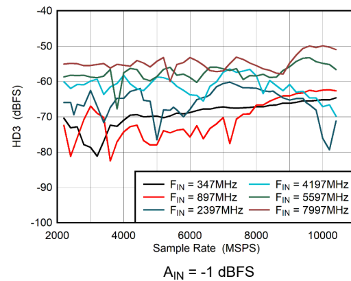
Figure 5-38. DES Mode: HD3 vs Sample Rate
