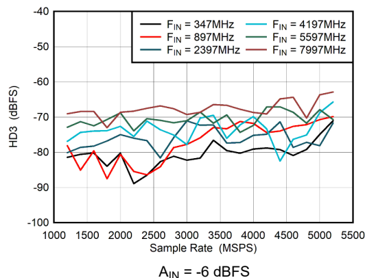
5-54. Dual Channel Mode: HD3 vs Sample Rate
