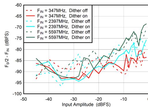
FIG 5-80. Dual Channel Mode: F_S/2 - F_{\text{IN}} vs Input Amplitude and Dither
