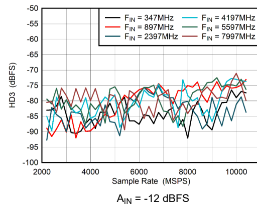
Figure 5-40. DES Mode: HD3 vs Sample Rate
