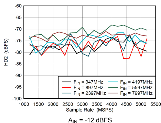
5-52. Dual Channel Mode: HD2 vs Sample Rate
