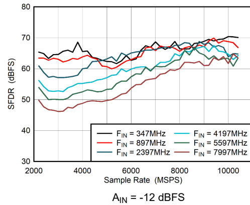
5-34. DES Mode: SFDR vs Sample Rate
