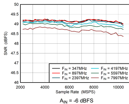
5-30. DES Mode: SNR vs Sample Rate
