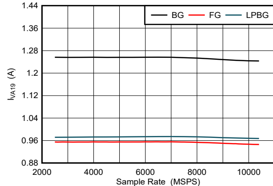
FIG 5-110. DES Mode: I_{VA19} vs Sample Rate
