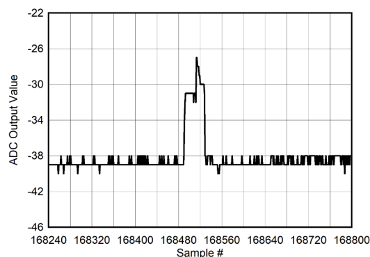
FIG 5-120. Background Calibration Core Transition (AC Signal Zoomed)
