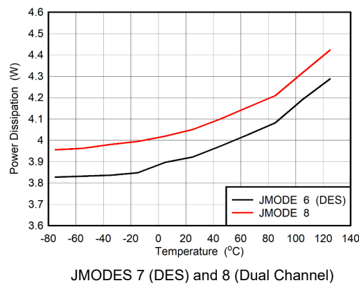
FIG 5-118. Power Dissipation vs Temperature
