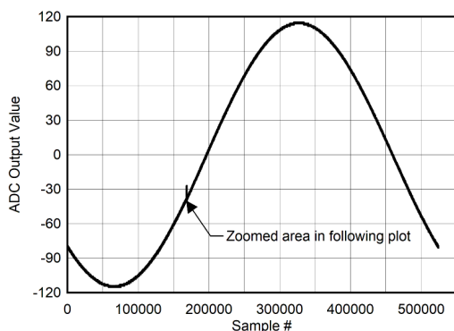
FIG 5-119. Background Calibration Core Transition (AC Signal)
