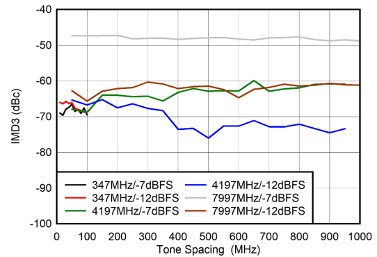
FIG 5-102. DES Mode: IMD3 vs Tone Spacing
