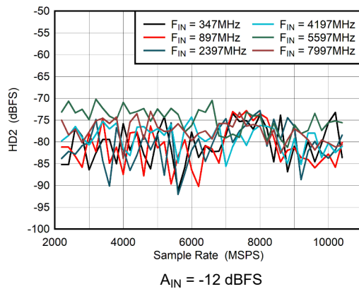
Figure 5-37. DES Mode: HD2 vs Sample Rate
