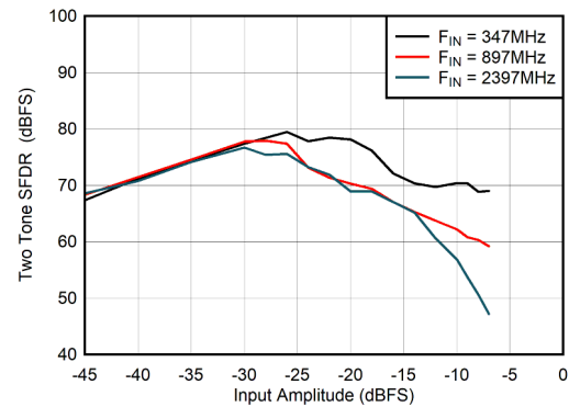
FIG 5-104. DES Mode: Two Tone SFDR vs Input Amplitude
