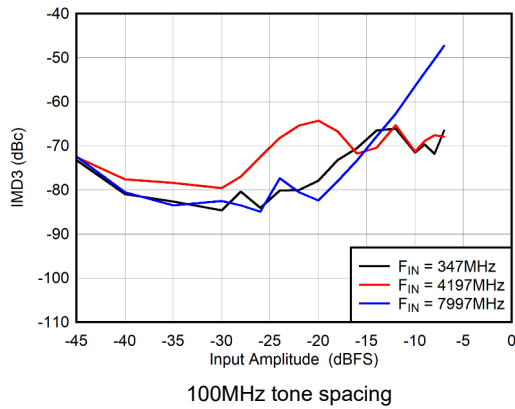
FIG 5-101. DES Mode: IMD3 vs Input Amplitude
