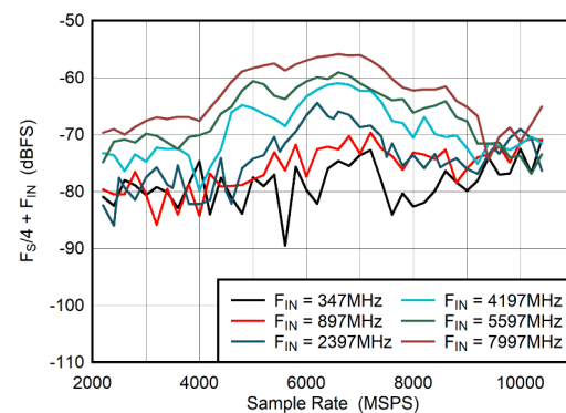
Figure 5-42. DES Mode: \text{FS}/4 + f_{\text{IN}} vs Sample Rate
