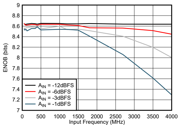
図 5-17. ENOB vs Input Frequency
