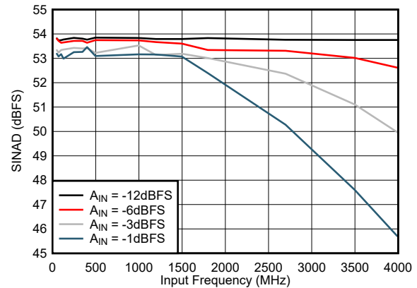
図 5-16. SINAD vs Input Frequency
