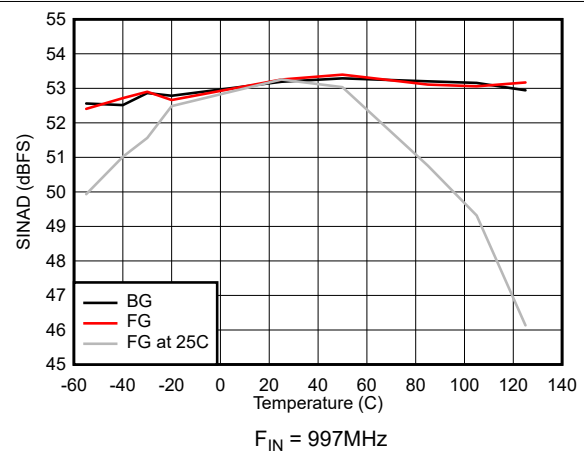
Figure 5-36. SINAD vs Temperature
