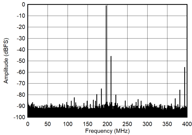
図 5-13. Single Tone FFT at 1797MHz and -1dBFS
