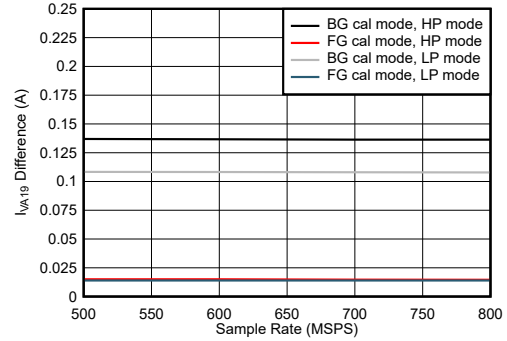
Figure 5-106. Single Channel, I_{VA19} Change with Calibration Mode
