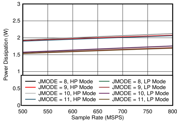
FIG 5-73. Quad Channel, Power Dissipation vs F_S for JMODES 8 - 11
