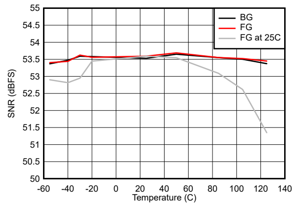
Figure 5-34. SNR vs Temperature
