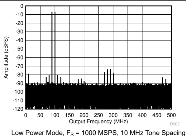
図 5-54. Two Tone FFT at 95.07 MHz Center
