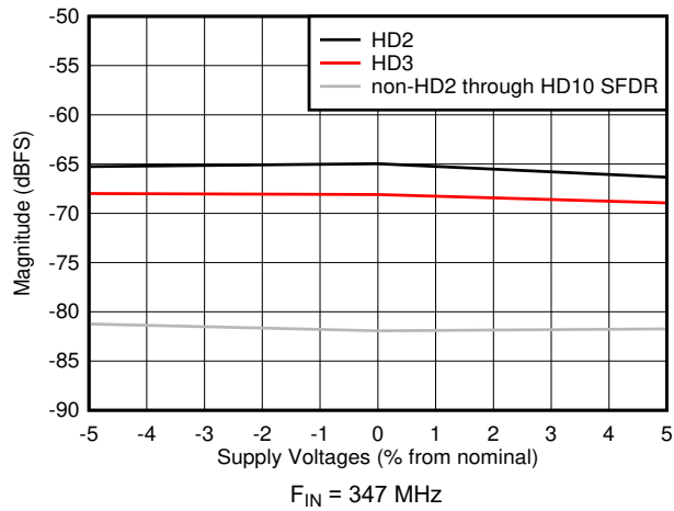
5-45. HD2, HD3 and Worst non-HD Spur vs Supply Voltage
