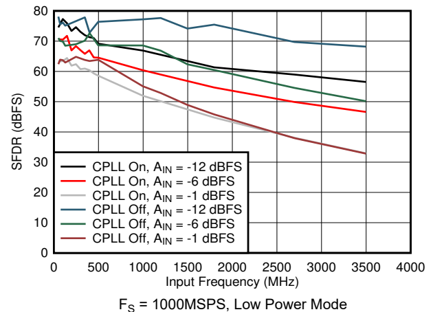
図 5-76. SFDR vs Input Frequency, CPLL and Input Amplitude
