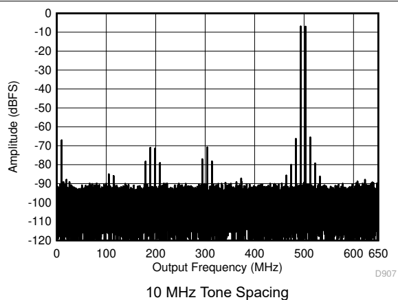
図 5-52. Two Tone FFT at 1798 MHz Center
