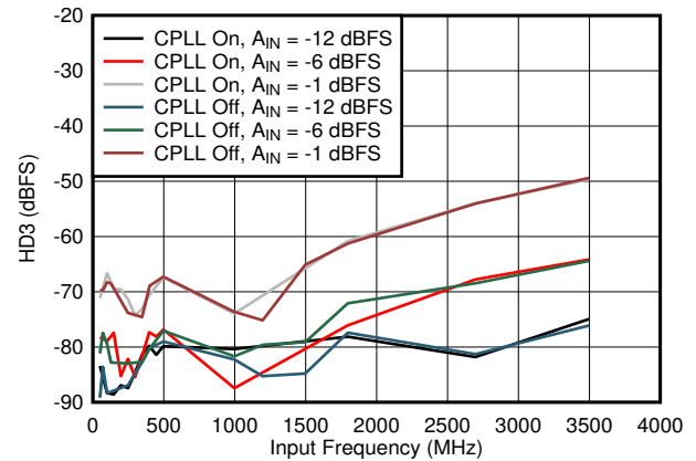
図 5-74. HD3 vs Input Frequency, CPLL and Input Amplitude
