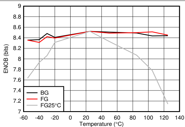
5-42. ENOB vs Temperature and Calibration Mode
