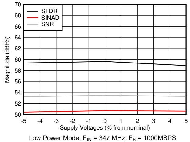
5-46. SNR, SFDR and SINAD vs Supply Voltage
