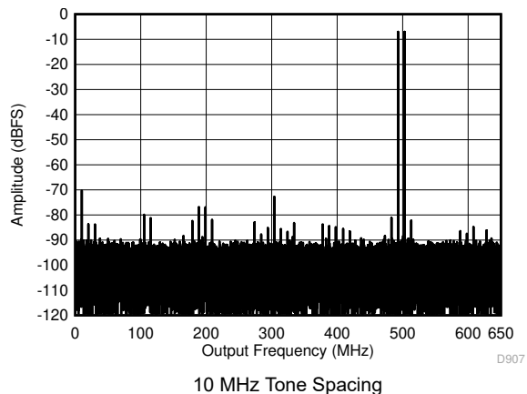
図 5-50. Two Tone FFT at 498 MHz Center
