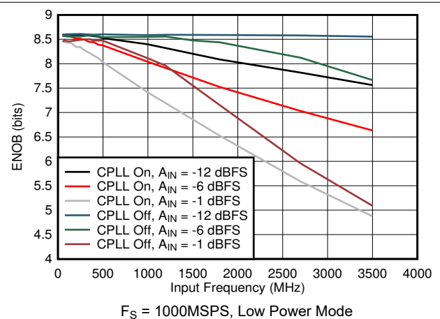
図 5-78. ENOB vs Input Frequency, CPLL and Input Amplitude
