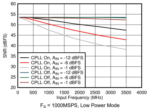
図 5-75. SNR vs Input Frequency, CPLL and Input Amplitude
