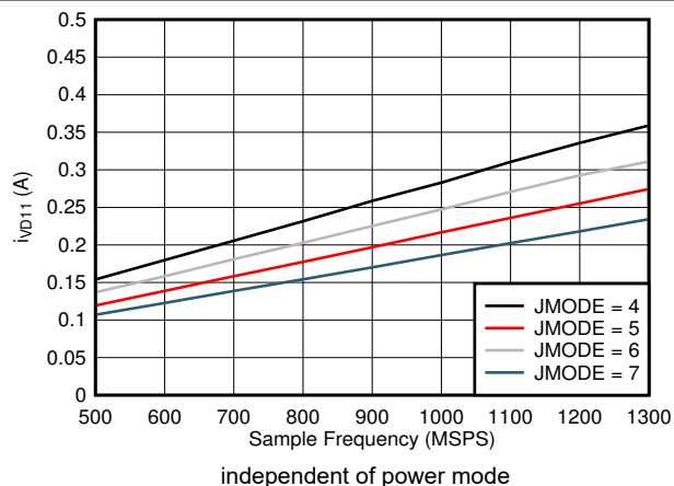
Figure 5-98. Dual Channel, I_{VD11} vs FS and JMODE 4 - 7
