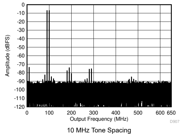
5-48. Two Tone FFT at 95.07 MHz Center
