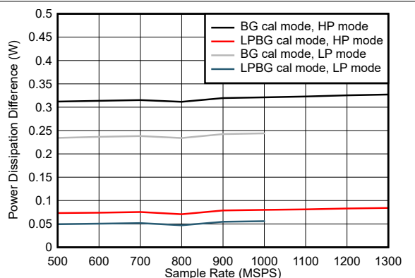
5-111. Quad Channel, Power Dissipation Change with Calibration Mode
