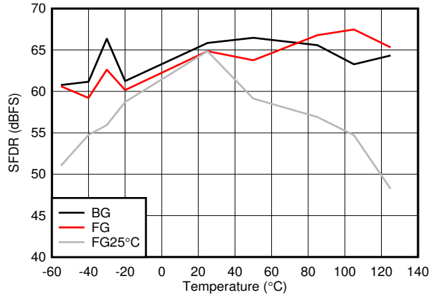
5-43. SFDR vs Temperature and Calibration Mode
