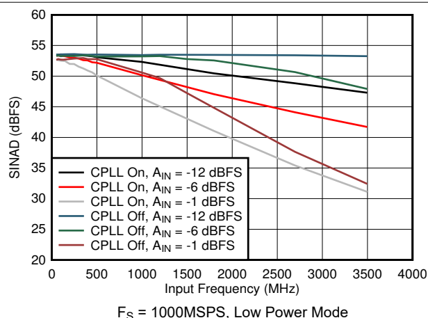
図 5-77. SINAD vs Input Frequency, CPLL and Input Amplitude
