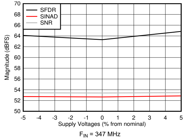
5-44. SNR, SFDR and SINAD vs Supply Voltage
