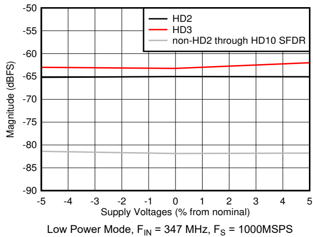
5-47. HD2, HD3 and Worst non-HD Spur vs Supply Voltage
