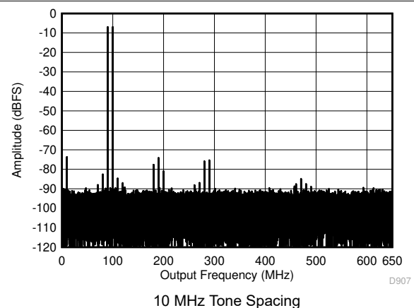
5-48. Two Tone FFT at 95.07 MHz Center
