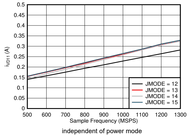
Figure 5-100. Dual Channel, I_{VD11} vs FS and JMODE 12 - 15
