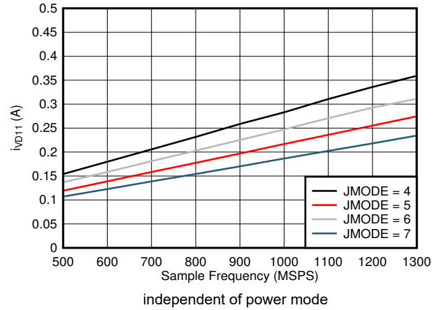
Figure 5-98. Dual Channel, I_{VD11} vs FS and JMODE 4 - 7
