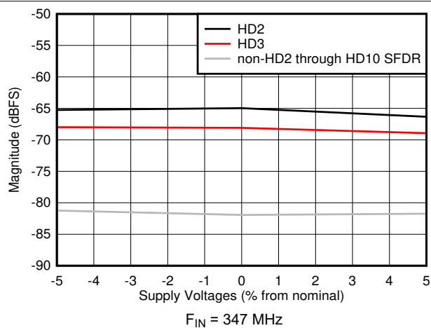
5-45. HD2, HD3 and Worst non-HD Spur vs Supply Voltage
