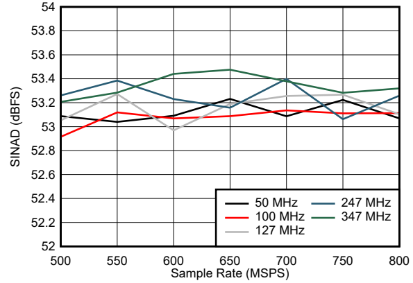
図 5-26. SINAD vs Sample Rate
