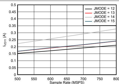
Figure 5-80. Quad Channel, I_{VD11} vs F_S for JMODES 12 - 15
