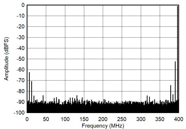
図 5-12. Single Tone FFT at 1197MHz and -1dBFS Low Power Mode
