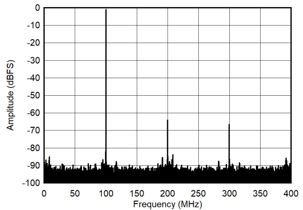
図 5-10. Single Tone FFT at 100MHz and -1dBFS Low Power Mode
