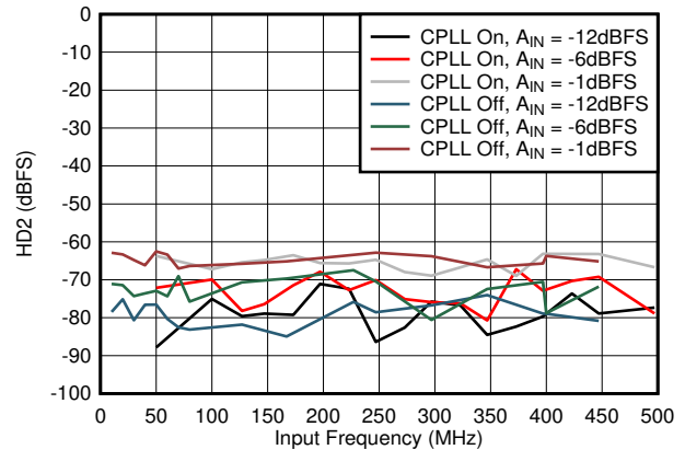
Figure 6-58. HD2 vs A_{IN} and C-PLL
