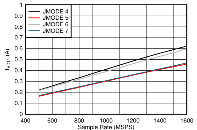
Figure 6-84. Quad Channel, I_{VDD11} vs F_S
