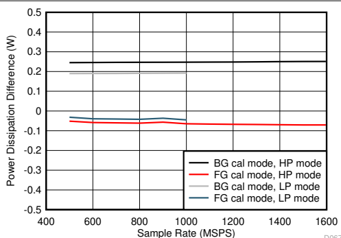
图 6-109. Quad Channel, Power Dissipation Change with Calibration Mode
