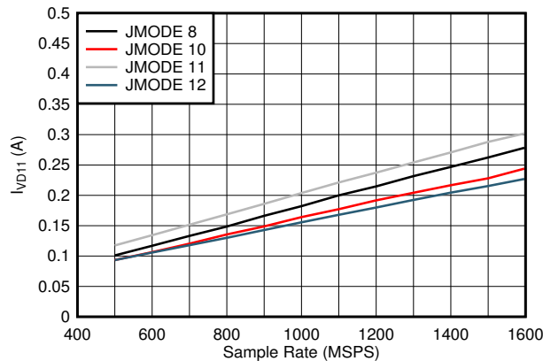
图 6-107. Single Channel, I_{VD11} vs F_S and JMODE 8 - 12
