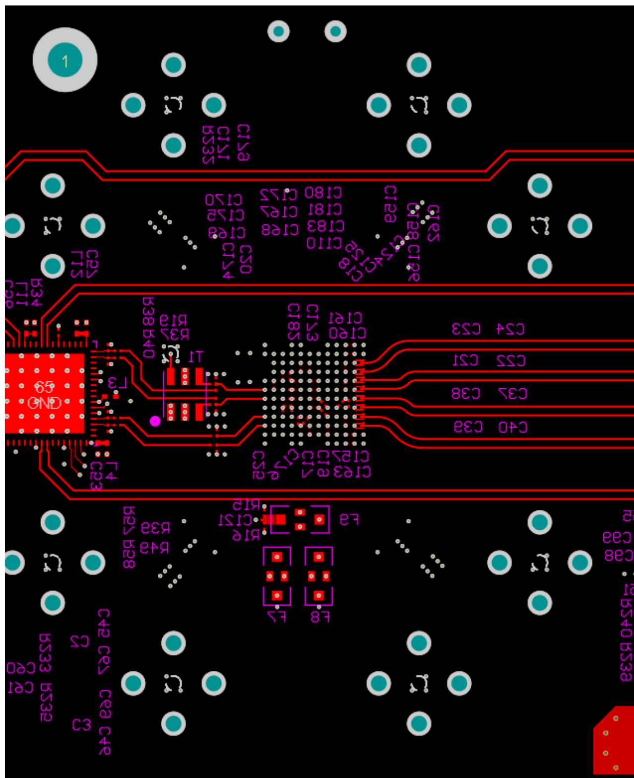
図 8-7. Bottom Layer Routing: CLK±, SYSREF and D[7:4]± Routing
