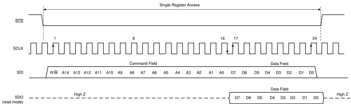
図 7-18. Serial Interface Protocol: Single Read/Write
