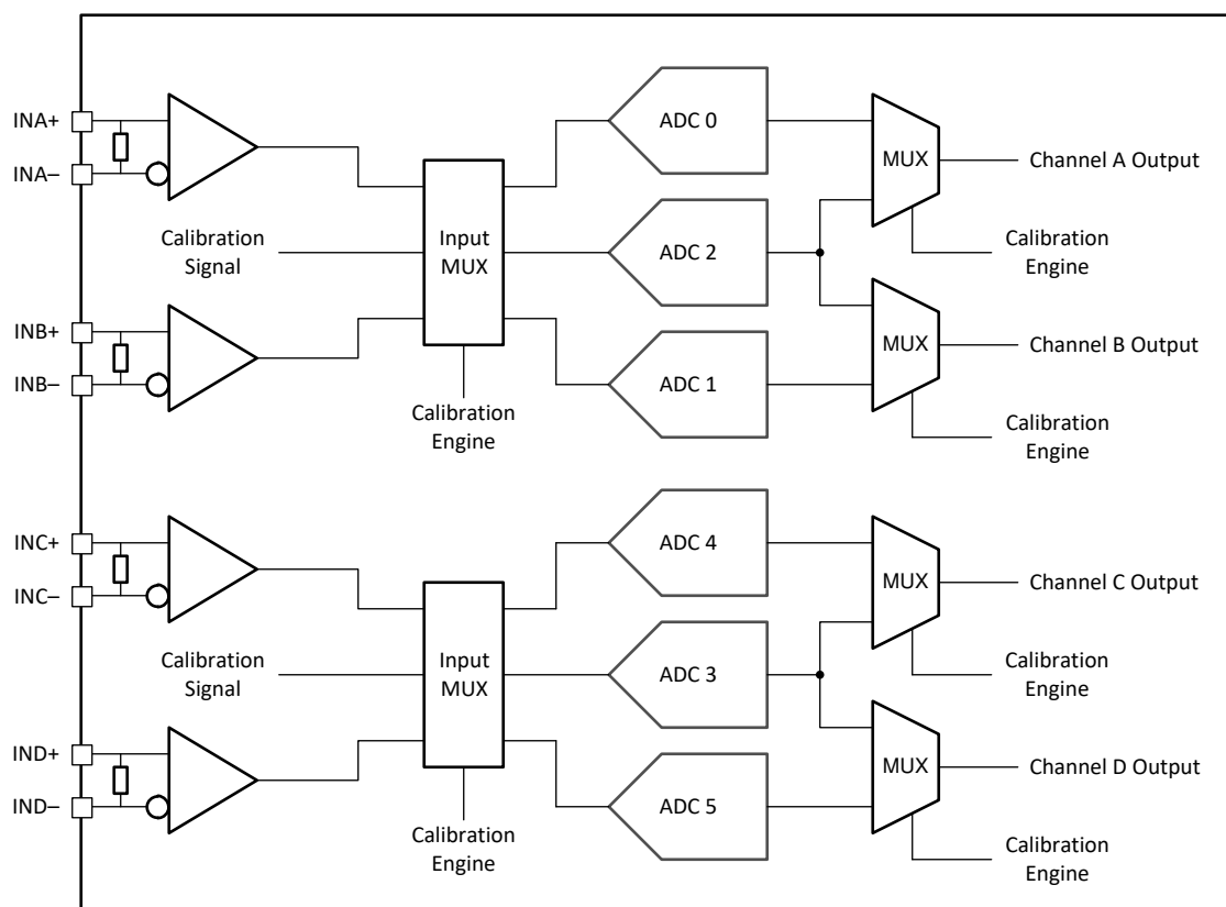
図 7-15. Quad Channel Calibration System Block Diagram
