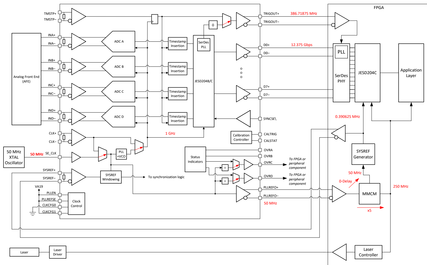
8-1. Typical Configuration for a LiDAR Digitizer
