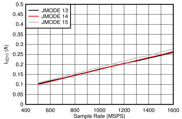
图 6-108. Single Channel, I_{VD11} vs F_S and JMODE 13 - 15
