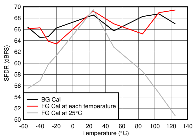
Figure 6-65. SFDR vs Temperature
