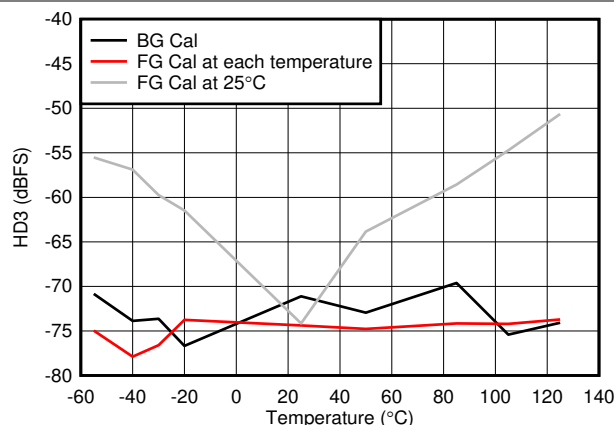
Figure 6-67. HD3 vs Temperature
