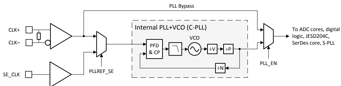
図 7-6. Converter PLL (C-PLL) Architecture
