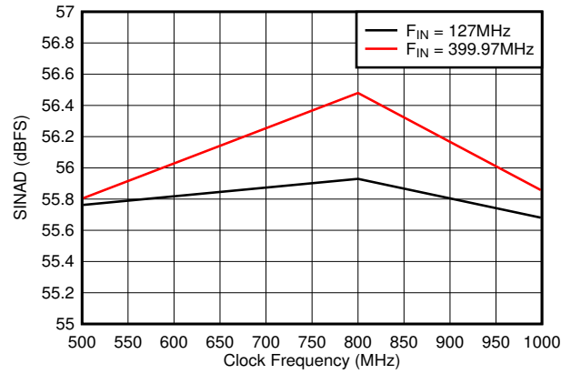
図 6-30. SINAD vs Sample Rate
