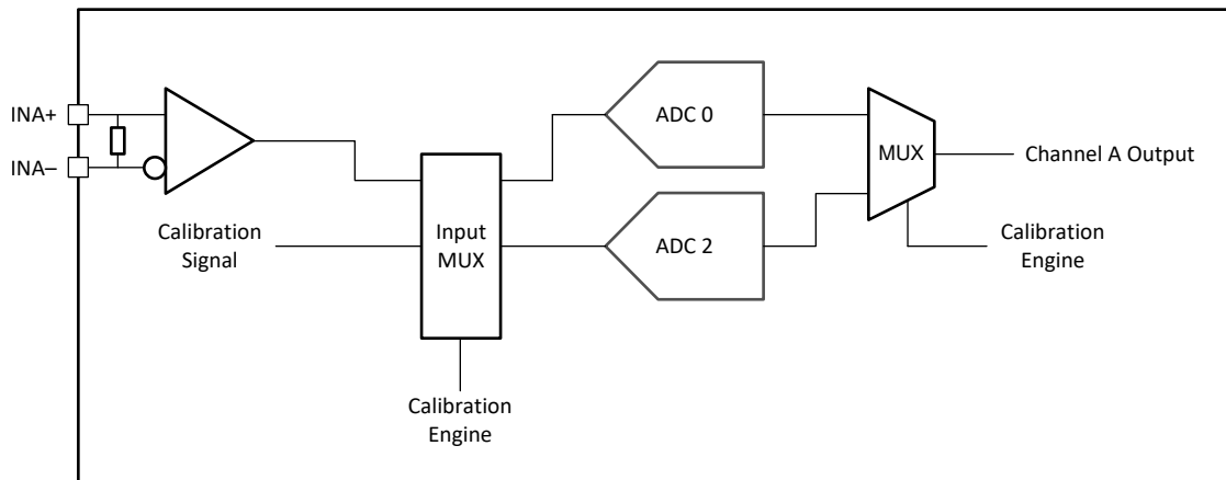
7-17. Single Channel Calibration System Block Diagram
