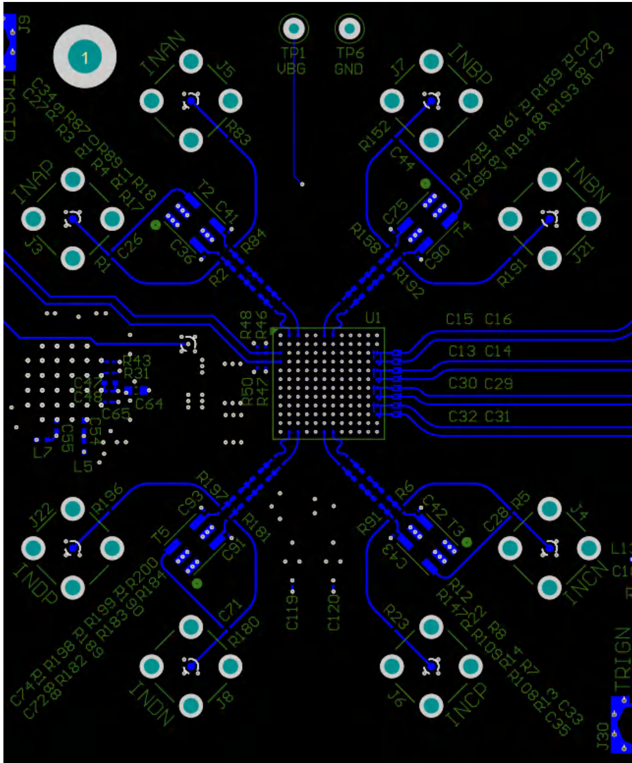
図 8-5. Top Layer Routing: Analog Inputs (INA±, INB±, INC±, IND±), TMSTP± and D[3:0]± Routing
