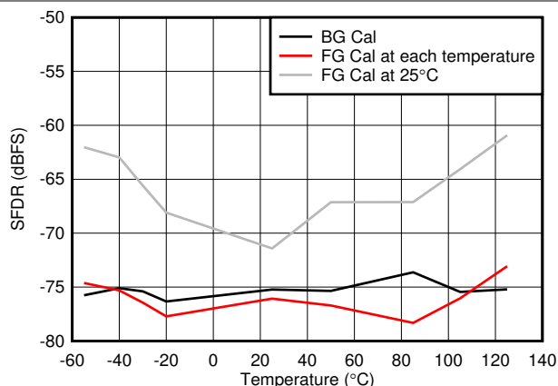
Figure 6-68. Worst Spur vs Temperature
