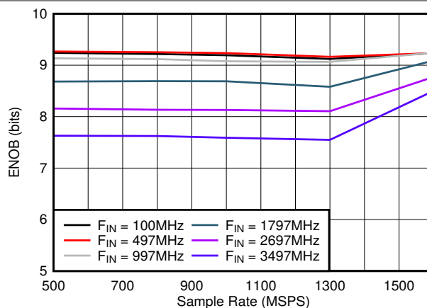
Figure 6-26. ENOB vs Sample Rate
