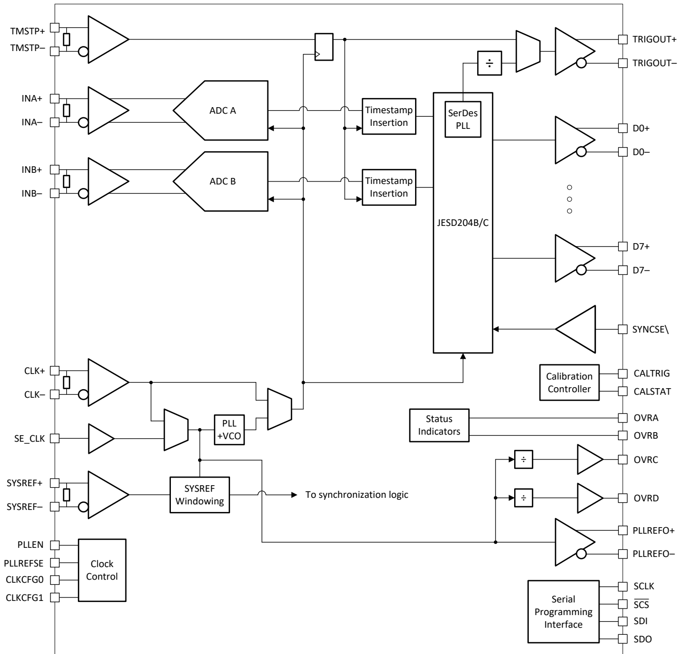
7-2. Dual Channel Functional Block Diagram
