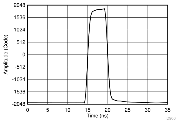
Figure 8-2. Measured Pulse using Sub-Sampling Technique for Equivalent 32 GSPS Measurement
