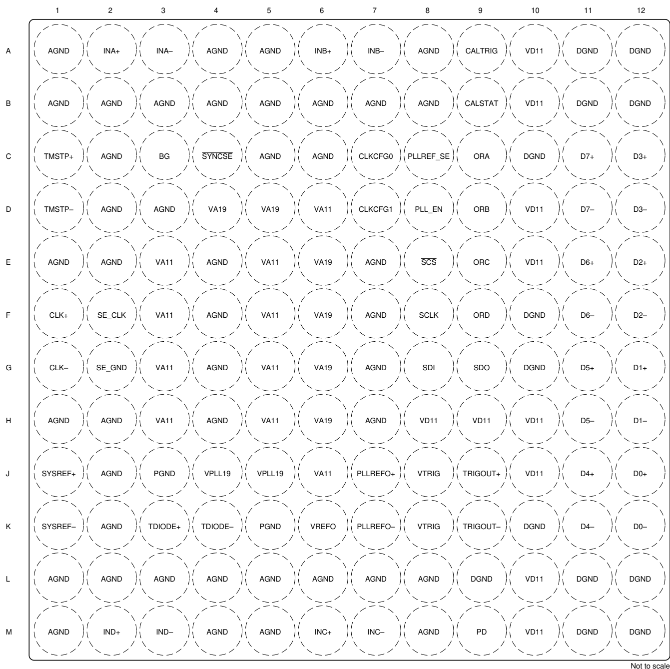
図 5-1. Quad Channel AAV Package, 144-Ball Flip Chip BGA (Top View)
