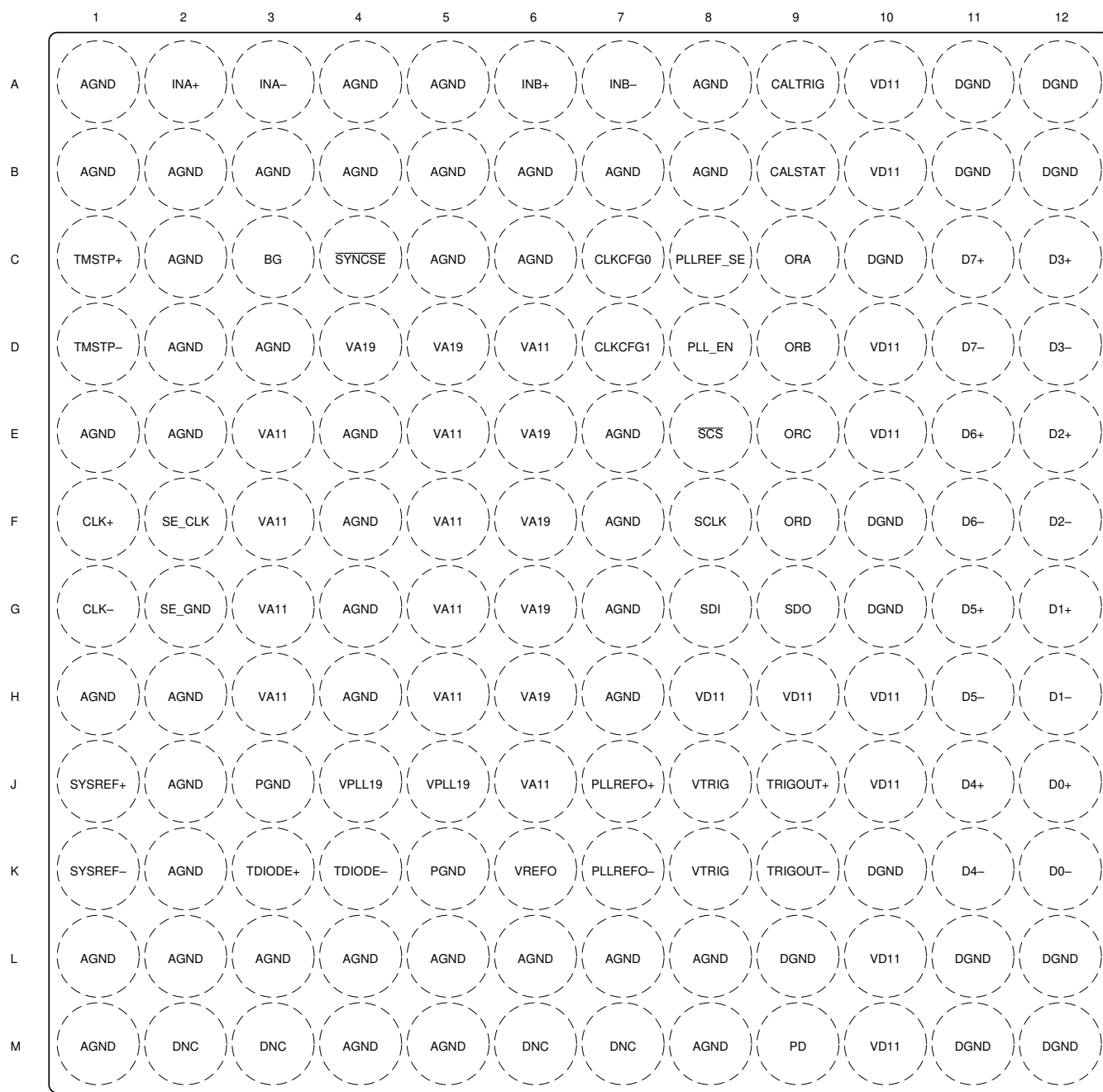
図 5-2. Dual Channel AAV Package, 144-Ball Flip Chip BGA (Top View)
