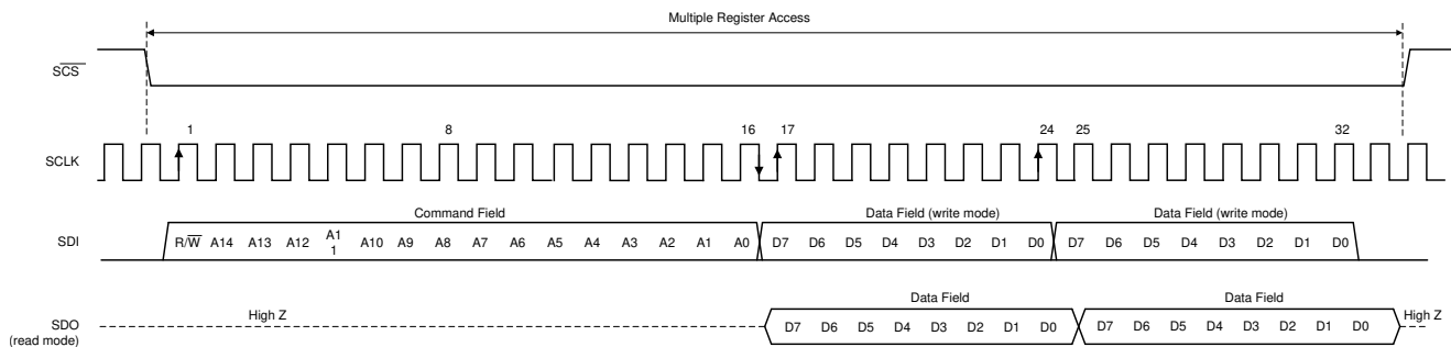
図 7-19. Serial Interface Protocol: Streaming Read/Write
