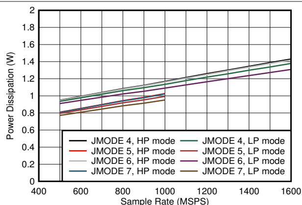
Figure 6-100. Single Channel, Power Dissipation vs F_S and JMODE 4 - 7
