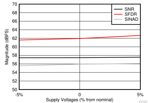
Figure 6-62. SNR, SFDR and SINAD vs Supply Voltages All supplies changed together, low power mode, F_S = 1000 MSPS
