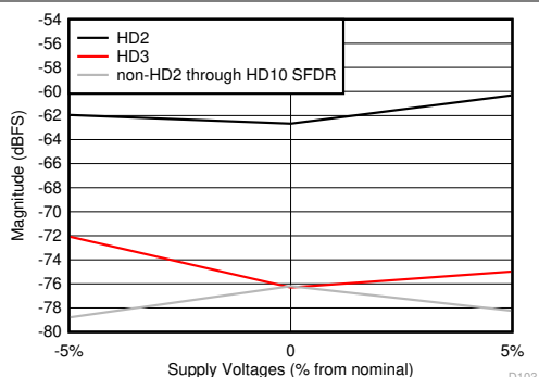
Figure 6-63. HD2, HD3 and Worst non-HD Spur vs Supply Voltage
