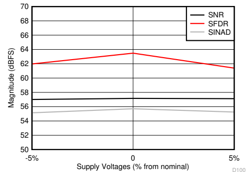
Figure 6-60. SNR, SFDR and SINAD vs Supply Voltage All supplies changed together, high power mode
