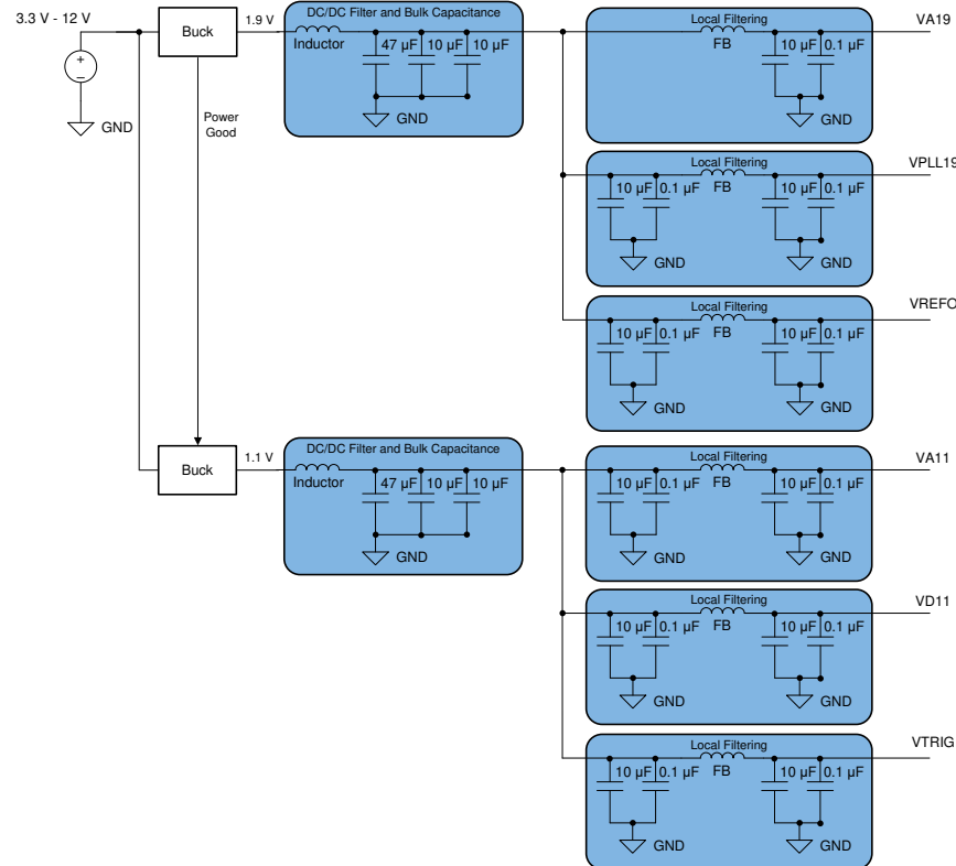
図 8-4. Switcher-Only Approach Example
