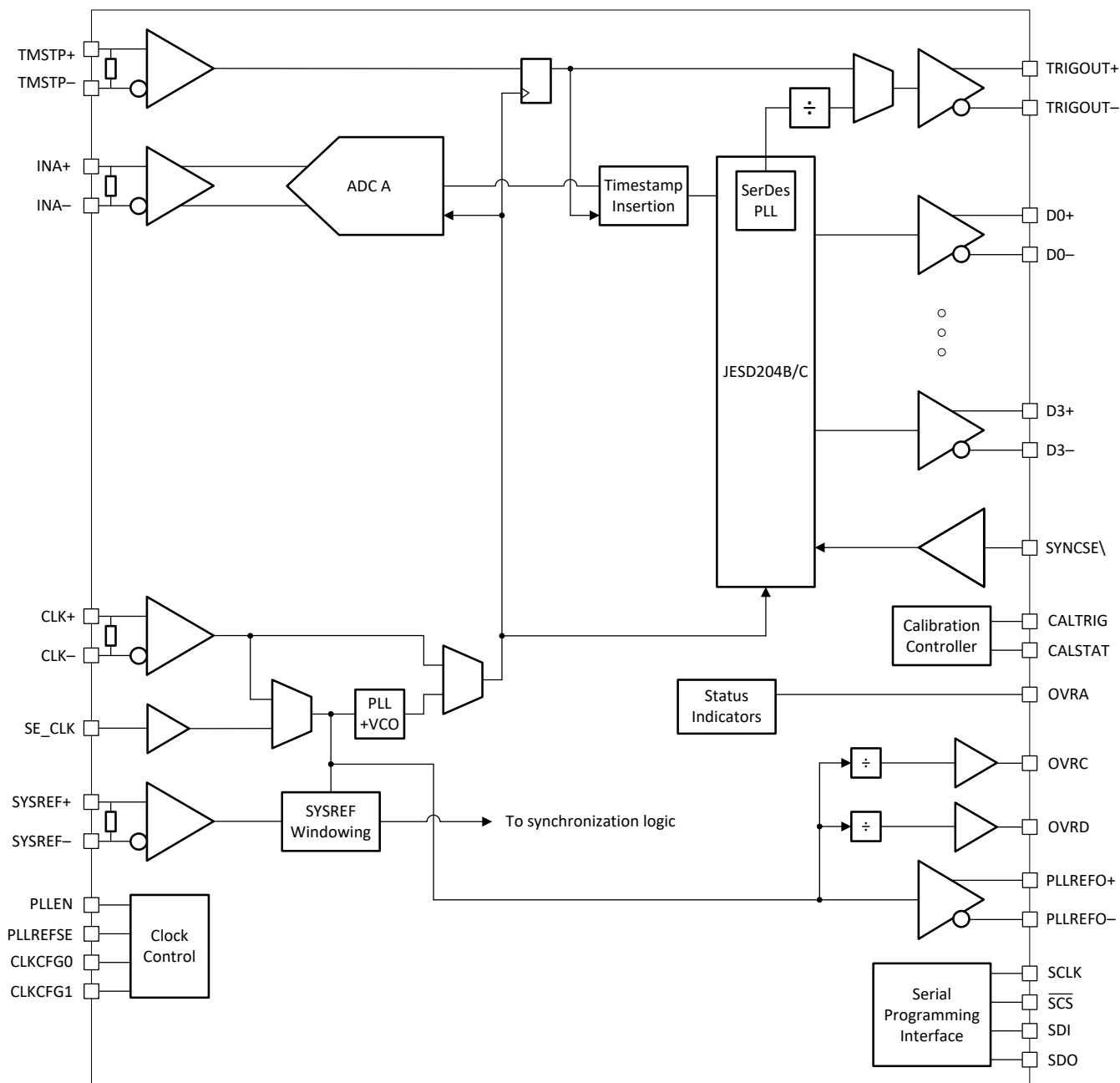
図 7-3. Single Channel Functional Block Diagram
