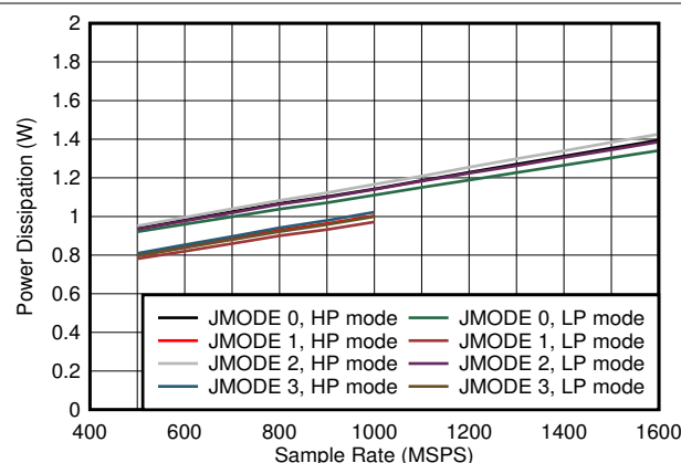
Figure 6-99. Single Channel, Power Dissipation vs F_S and JMODE 0 - 3
