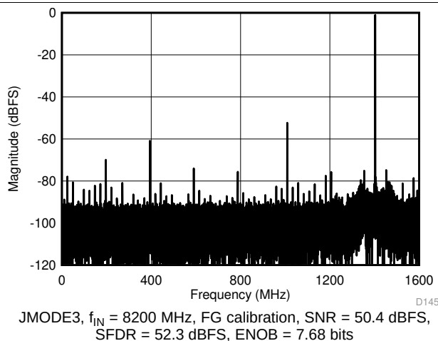
Figure 26. Single-Tone FFT at A_{\text{IN}} = -1\text{ dBFS}
