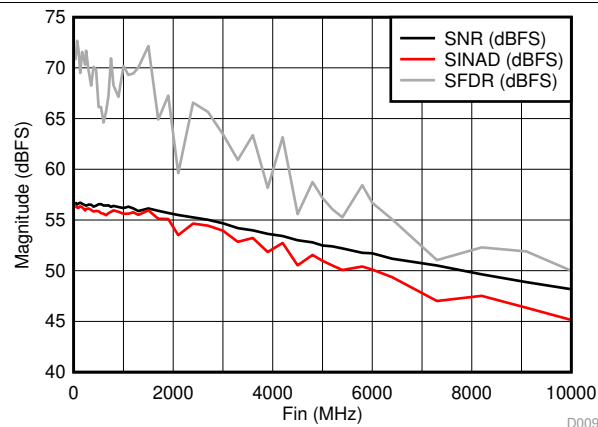
JMODE3, f_{\text{CLK}} = 3200\text{ MHz} , BG calibration
