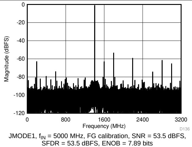
Figure 25. Single-Tone FFT at A_{\text{IN}} = -1\text{ dBFS}
