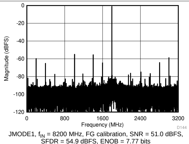
Figure 27. Single-Tone FFT at A_{\text{IN}} = -1\text{ dBFS}
