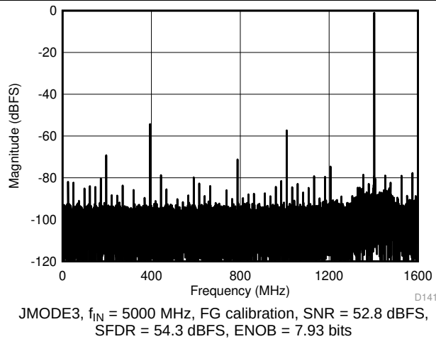
Figure 24. Single-Tone FFT at A_{\text{IN}} = -1\text{ dBFS}
