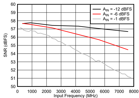
FIG 6-83. Dual Channel Mode: SNR vs Input Frequency
