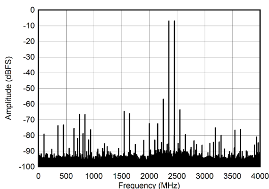
FIG 6-17. DES Mode: Two Tone FFT at 5597 MHz
