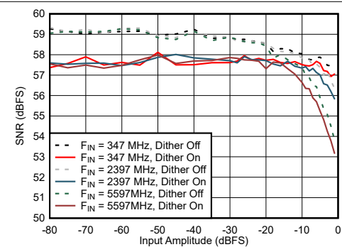
図 6-68. Dual Channel Mode: SNR vs Input Amplitude and Dither
