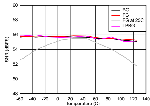
图 6-96. DES Mode: SNR vs Temperature and Calibration Mode
