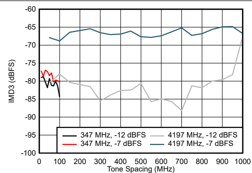
图 6-108. DES Mode: IMD3 vs Tone Spacing
