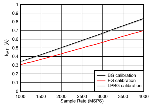
图 6-127. Dual Channel Mode: I_{VA11} vs Sample Rate
