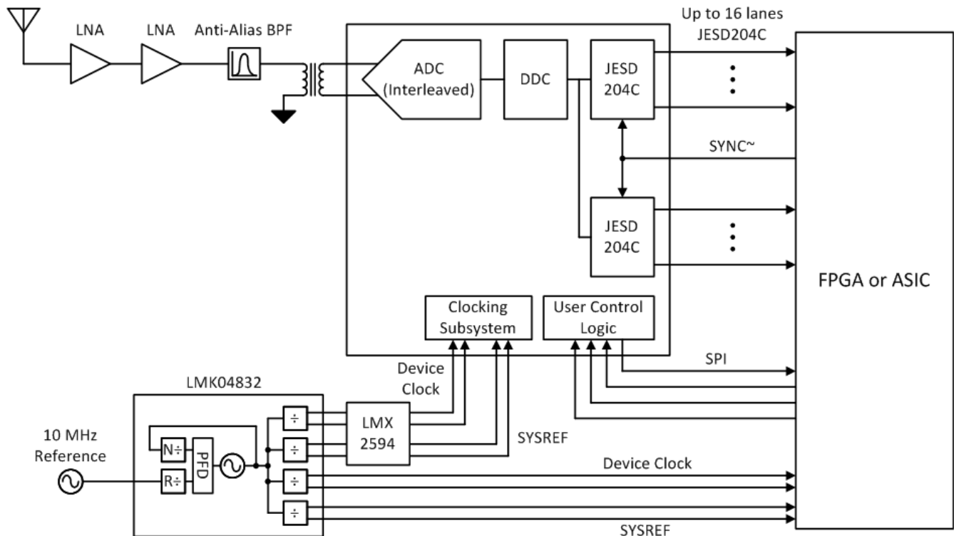
図 8-1. Typical Configuration for Wideband RF Sampling
