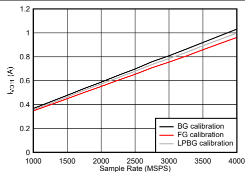
图 6-128. Dual Channel Mode: I_{VD11} vs Sample Rate
