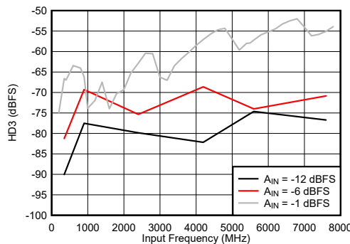
FIG 6-86. Dual Channel Mode: HD3 vs Input Frequency
