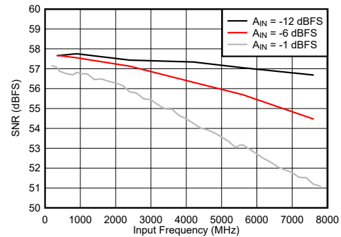
FIG 6-82. DES Mode: F_{\text{IN}} \pm F_S/4 vs Input Frequency
