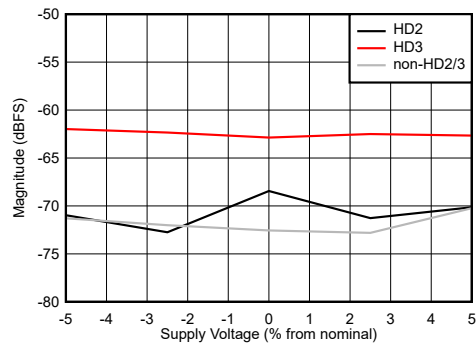
FIG 6-101. DES Mode: HD2, HD3 and Worst non-HD Spur vs Supply Voltage
