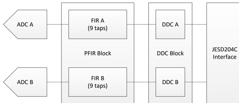
図 7-4. Dual Channel Equalization PFIR Block Diagram
