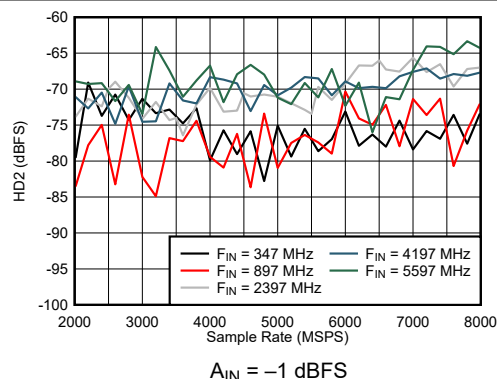
图 6-34. DES Mode: HD2 vs Sample Rate and Input Frequency
