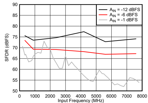
FIG 6-84. Dual Channel Mode: SFDR vs Input Frequency
