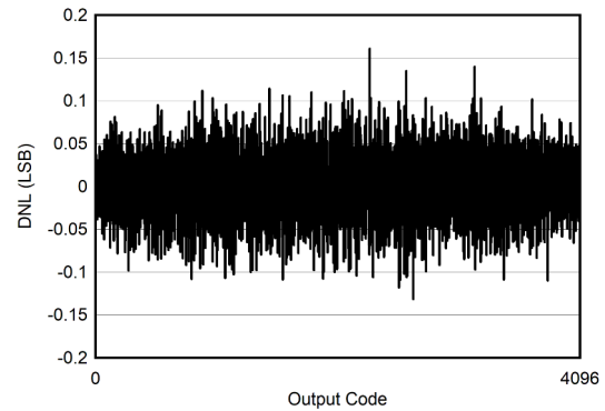
Figure 6-6. DNL vs ADC Code
