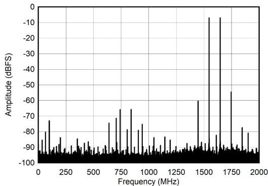
FIG 6-27. Dual Channel Mode: Two Tone FFT at 4197 MHz
