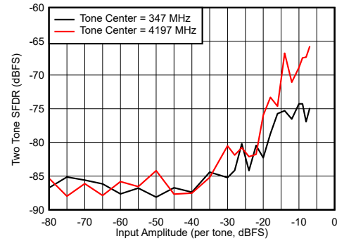
図 6-112. DES Mode: Two Tone SFDR vs Input Amplitude
