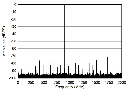
FIG 6-19. Dual Channel Mode: Single Tone FFT at 897 MHz
