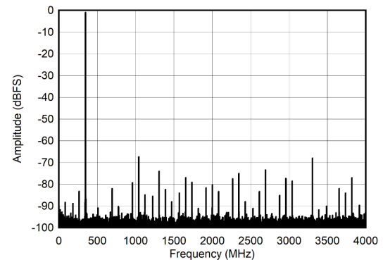
Figure 6-8. DES Mode: Single Tone FFT at 347 MHz
