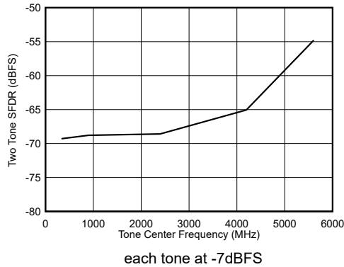
図 6-111. Dual Channel Mode: Two Tone SFDR vs Input Frequency
