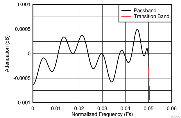
7-14. Decimate-by-8 Composite Zoomed Pass-Band Response
