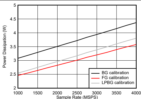
Figure 6-122. DES Mode: Power Dissipation vs Sample Rate
