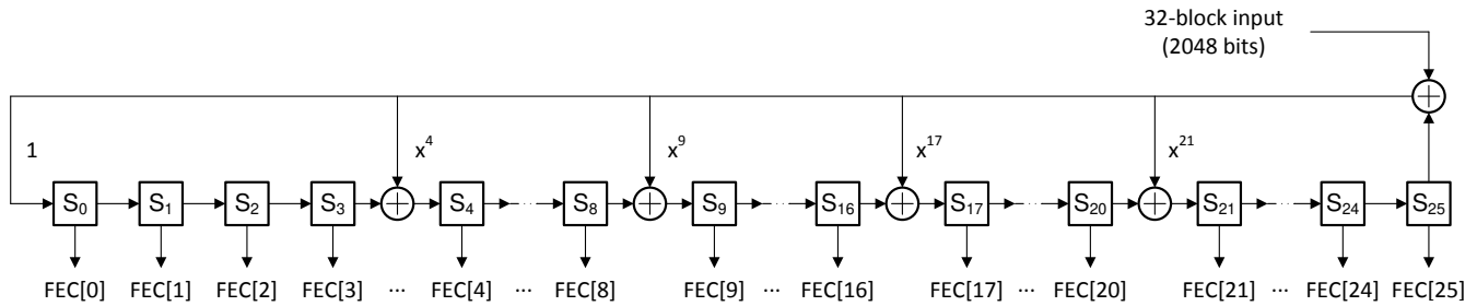
図 7-22. FEC Parity Bit Generator
