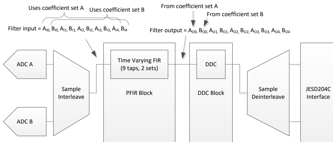
図 7-6. Time Varying Filter PFIR Block Diagram
