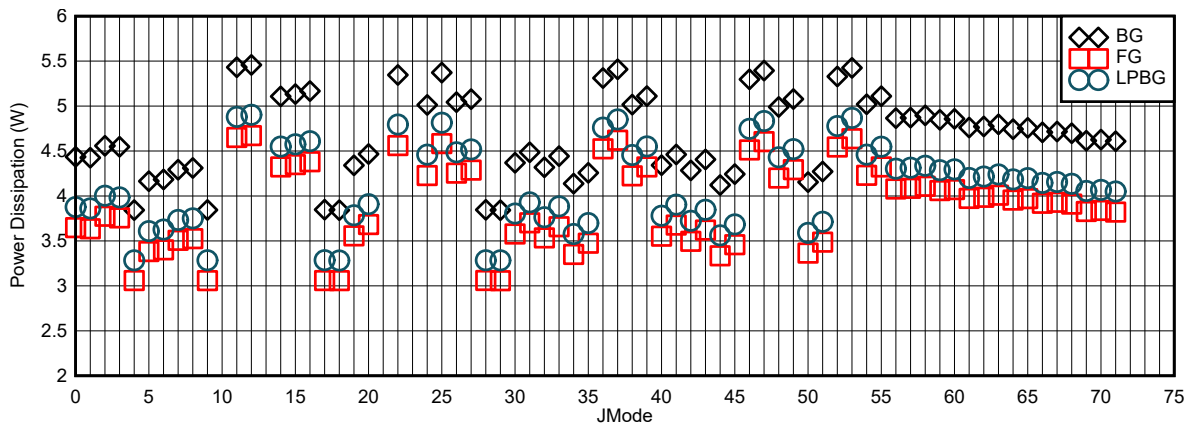
図 6-114. Power Dissipation vs JMODE at F_{\text{CLK}} = 4\text{ GHz}
