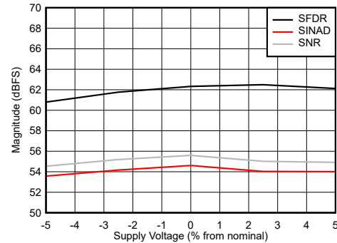
FIG 6-100. DES Mode: SNR, SINAD and SFDR vs Supply Voltage
