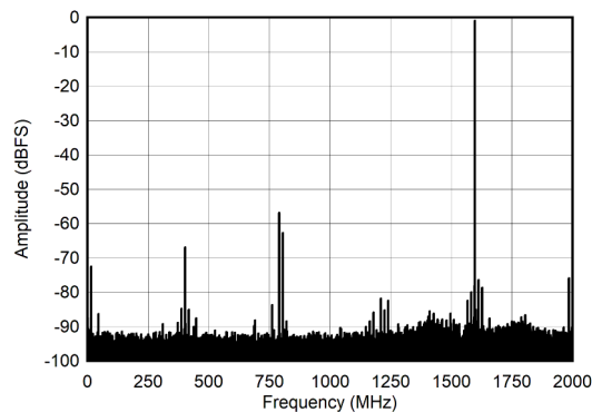
FIG 6-22. Dual Channel Mode: Single Tone FFT at 5597 MHz
