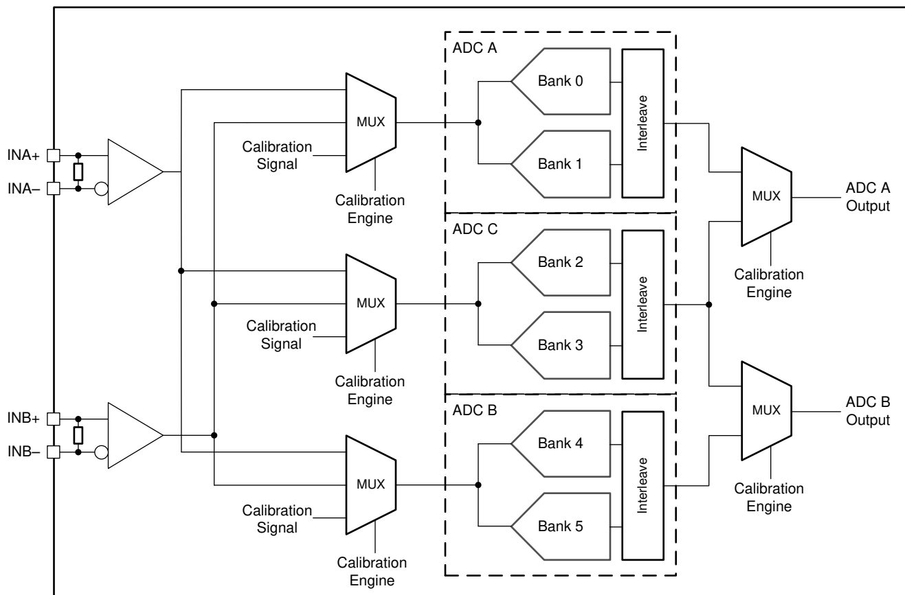
図 7-26. ADC12DJ4000RF Calibration System Block Diagram
