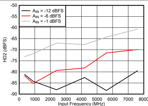
Figure 6-79. DES Mode: HD2 vs Input Frequency
