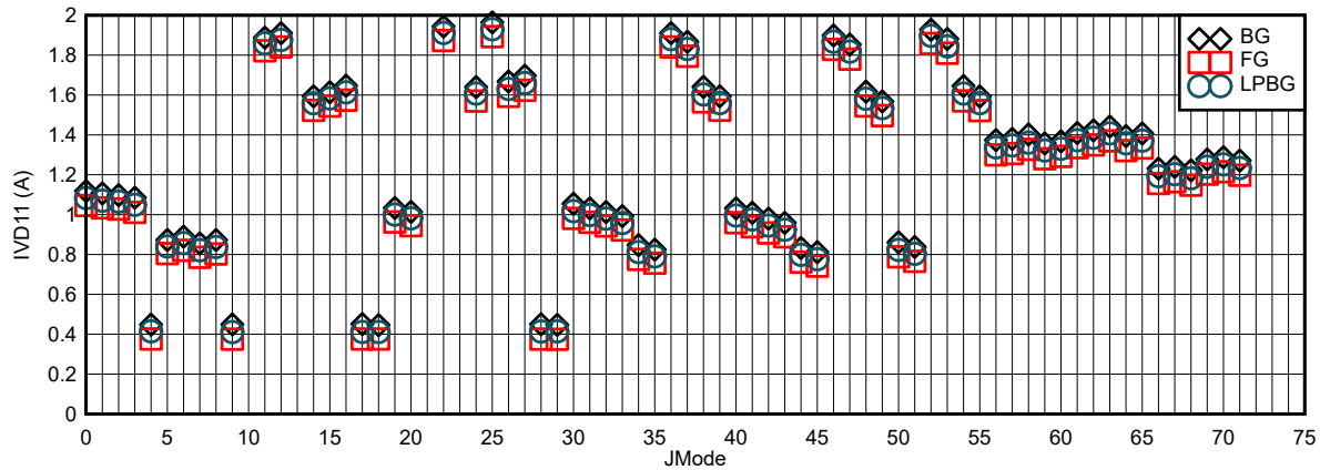
Figure 6-115. I_{VD11} vs \text{JMODE} at F_{\text{CLK}} = 4\text{ GHz}
