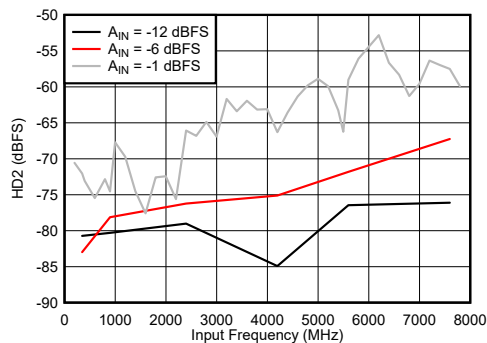
FIG 6-85. Dual Channel Mode: HD2 vs Input Frequency
