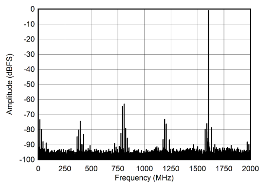
FIG 6-20. Dual Channel Mode: Single Tone FFT at 2397 MHz
