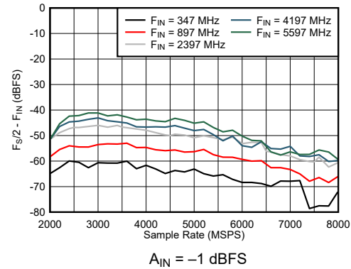
Figure 6-40. DES Mode: F_S/2 - F_{\text{IN}} vs Sample Rate and Input Frequency
