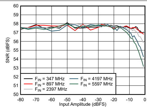
図 6-67. Dual Channel Mode: SNR vs Input Amplitude and Frequency
