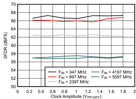
図 6-91. Dual Channel Mode: SFDR vs Clock Amplitude
