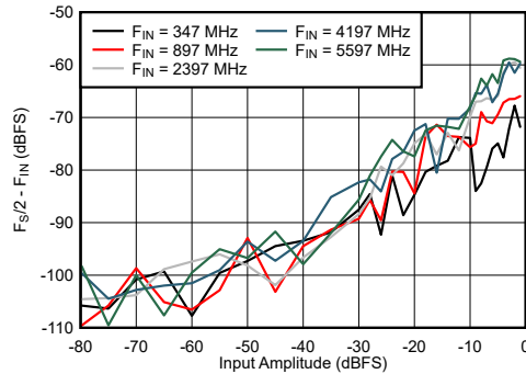
図 6-63. DES Mode: F_S/2 - F_{\text{IN}} vs Input Amplitude and Frequency
