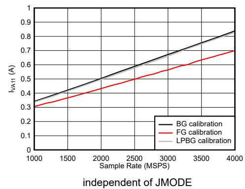
Figure 6-117. DES Mode: I_{VA11} vs Sample Rate
