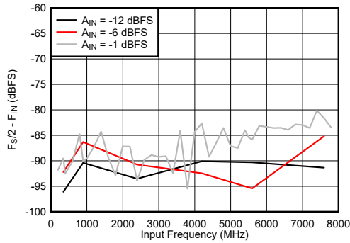
図 6-87. Dual Channel Mode: F_s/2 - F_{\text{IN}} vs Input Frequency
