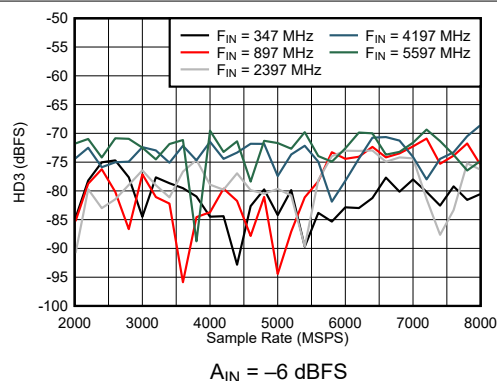
图 6-38. DES Mode: HD3 vs Sample Rate and Input Frequency
