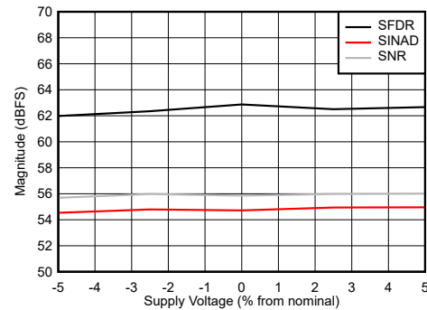
FIG 6-102. Dual Channel Mode: SNR, SINAD and SFDR vs Supply Voltage
