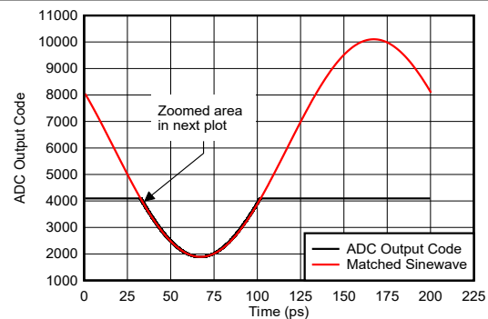
Figure 6-143. Sinewave Overdrive Recovery
