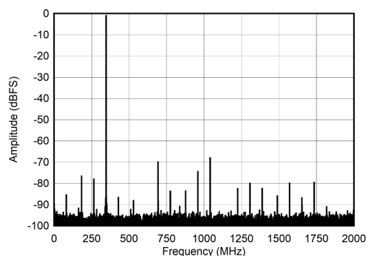
FIG 6-18. Dual Channel Mode: Single Tone FFT at 347 MHz
