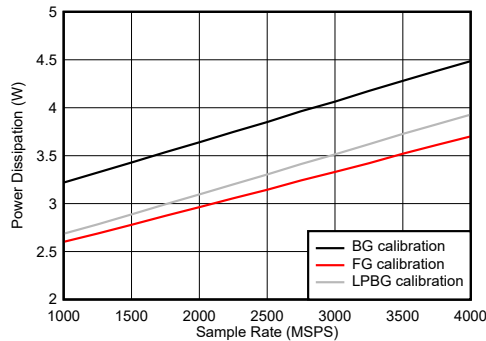
6-132. Dual Channel Mode: Power Dissipation vs Sample Rate
