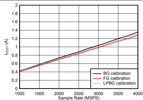
图 6-129. Dual Channel Mode: I_{VD11} vs Sample Rate
