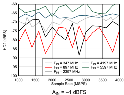
Figure 6-48. Dual Channel Mode: HD2 vs Sample Rate and Input Frequency
