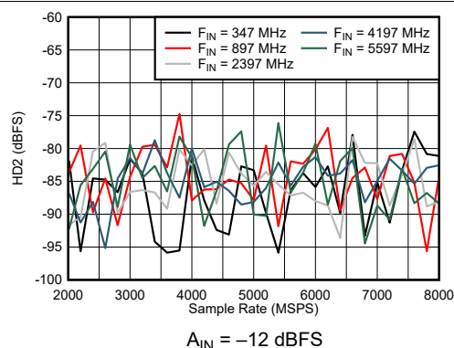
图 6-36. DES Mode: HD2 vs Sample Rate and Input Frequency
