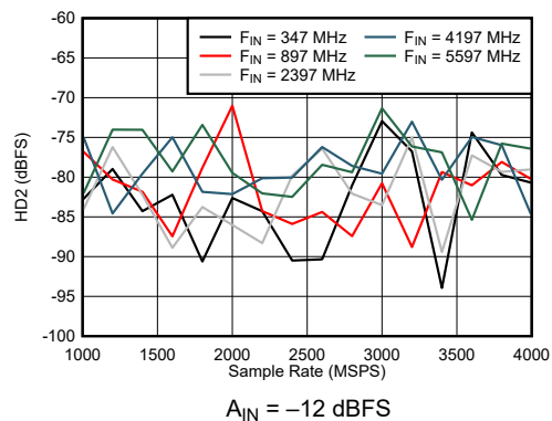
Figure 6-50. Dual Channel Mode: HD2 vs Sample Rate and Input Frequency
