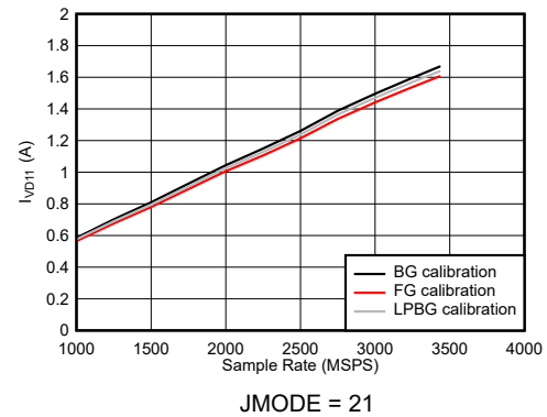
Figure 6-119. DES Mode: I_{VD11} vs Sample Rate
