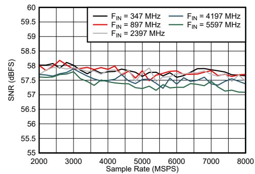
FIG 6-30. DES Mode: SNR vs Sample Rate and Input Frequency
