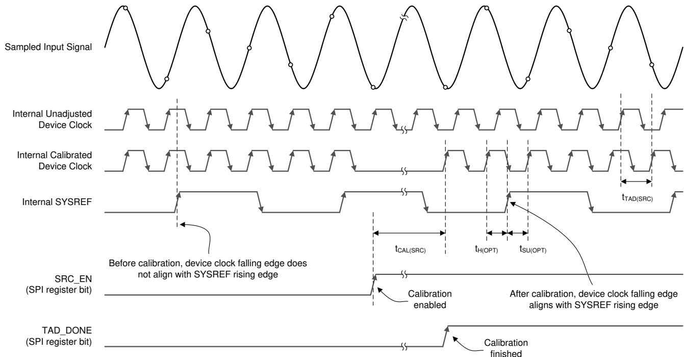
図 7-3. SYSREF Calibration Timing Diagram
