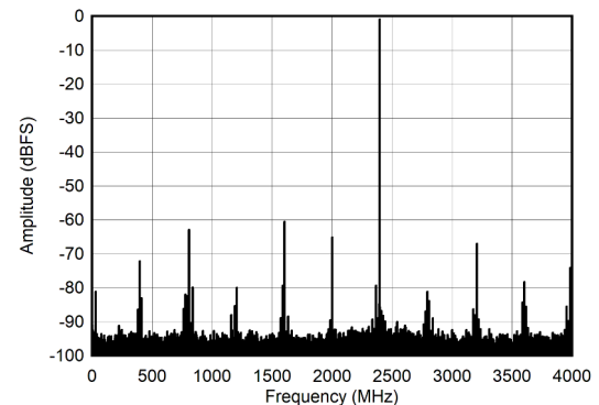
Figure 6-10. DES Mode: Single Tone FFT at 2397 MHz
