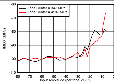
图 6-107. Dual Channel Mode: IMD3 vs Input Amplitude
