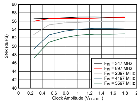
図 6-90. Dual Channel Mode: SNR vs Clock Amplitude
