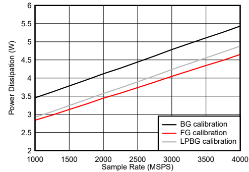
6-133. Dual Channel Mode: Power Dissipation vs Sample Rate
