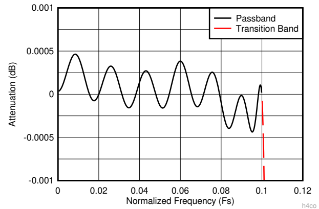
7-12. Decimate-by-4 Composite Zoomed Pass-Band Response
