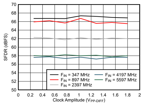
図 6-89. DES Mode: SFDR vs Clock Amplitude
