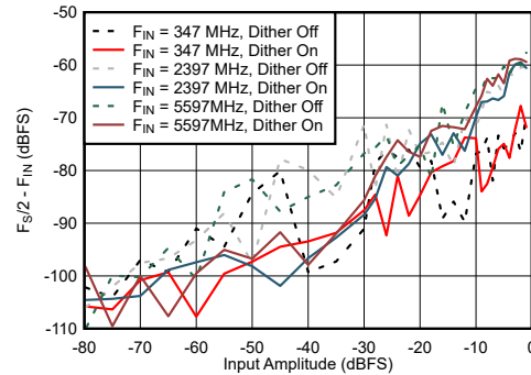
図 6-64. DES Mode: F_S/2 - F_{\text{IN}} vs Input Amplitude and Dither
