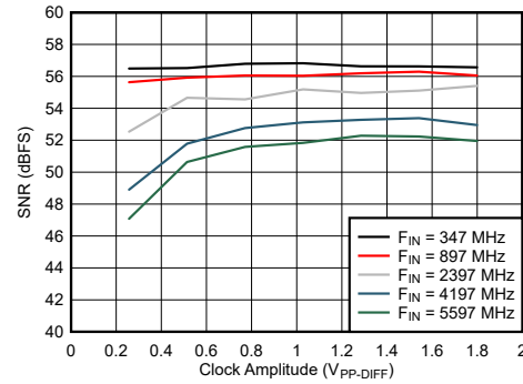
図 6-88. DES Mode: SNR vs Clock Amplitude
