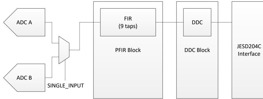
図 7-5. Single Channel Equalization PFIR Block Diagram
