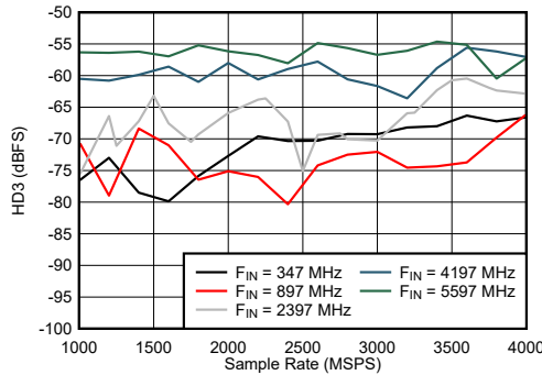
Figure 6-51. Dual Channel Mode: HD3 vs Sample Rate and Input Frequency
