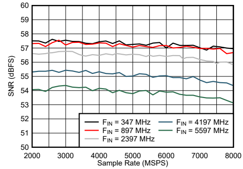
FIG 6-28. DES Mode: SNR vs Sample Rate and Input Frequency
