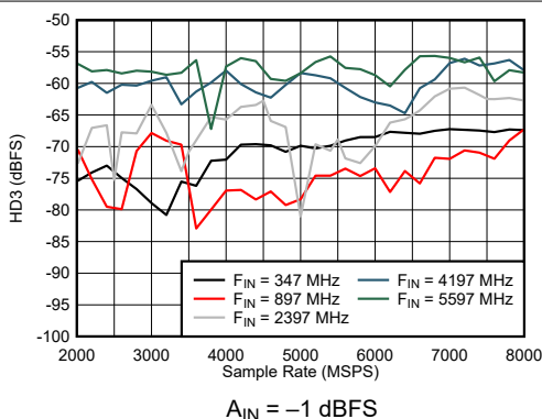
图 6-37. DES Mode: HD3 vs Sample Rate and Input Frequency
