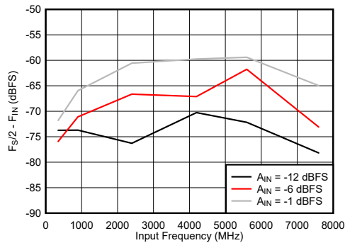
FIG 6-81. DES Mode: F_S/2 - F_{\text{IN}} vs Input Frequency
