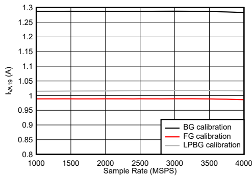
图 6-126. Dual Channel Mode: I_{VA19} vs Sample Rate
