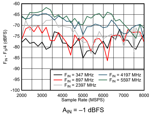
Figure 6-41. DES Mode: F_{\text{IN}} \pm F_S/4 vs Sample Rate and Input Frequency
