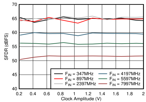
Figure 5-84. Dual Channel Mode: SFDR vs Clock Amplitude
