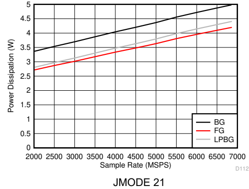
5-128. DES Mode: Power Dissipation vs Sample Rate
