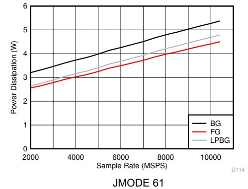
5-130. DES Mode: Power Dissipation vs Sample Rate
