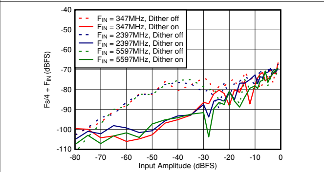
Figure 5-66. DES Mode: F_s/2 - F_{\text{IN}} vs Input Amplitude and Dither
