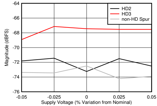
5-96. Dual Channel Mode: HD2, HD3 and Worst non-HD Spur vs Supply Voltage
