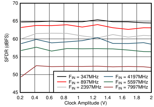
Figure 5-82. DES Mode: SFDR vs Clock Amplitude
