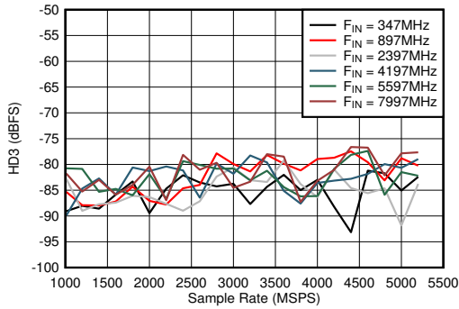
5-55. Dual Channel Mode: HD3 vs Sample Rate and Input Frequency
