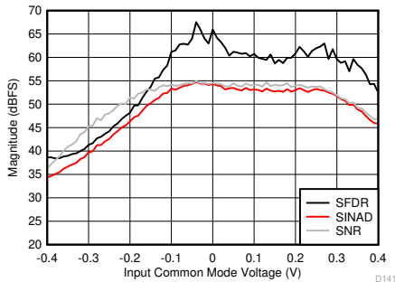
5-97. SNR, SFDR and SINAD vs Input Common Mode Voltage
