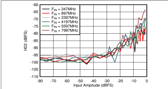
Figure 5-61. DES Mode: HD2 vs Input Amplitude and Frequency
