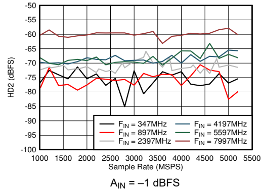
5-50. Dual Channel Mode: HD2 vs Sample Rate and Input Frequency
