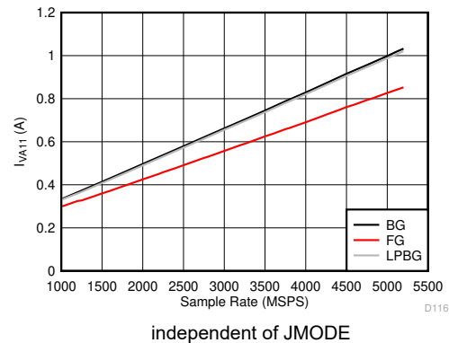
5-132. Dual Channel Mode: I_{VA11} vs Sample Rate
