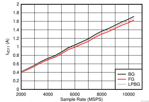
图 5-126. DES Mode: I_{VD11} vs Sample Rate
