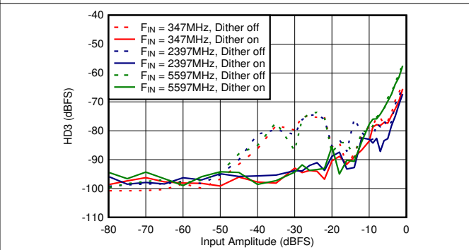
Figure 5-64. DES Mode: HD3 vs Input Amplitude and Dither
