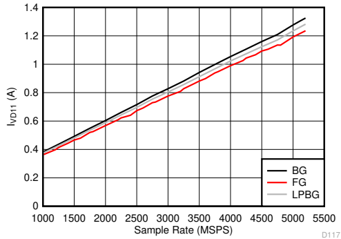
5-133. Dual Channel Mode: I_{VD11} vs Sample Rate
