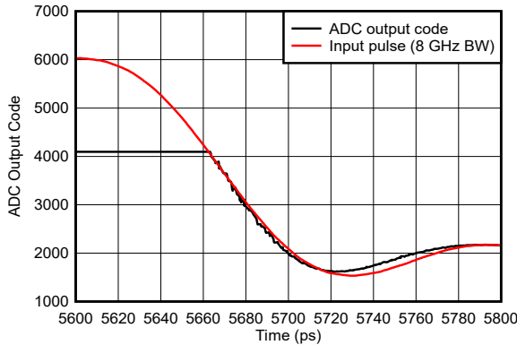
5-147. Pulse Overdrive Recovery Zoomed
