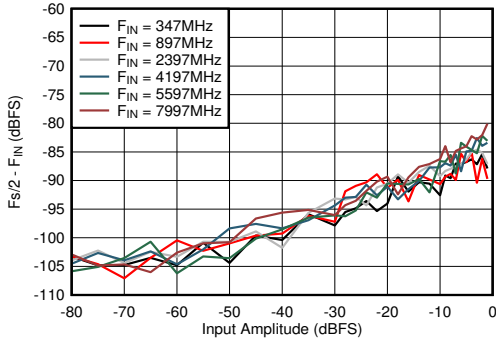
Figure 5-79. Dual Channel Mode: F_s/2 - F_{IN} vs Input Amplitude and Frequency
