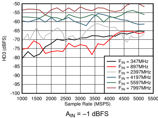
5-53. Dual Channel Mode: HD3 vs Sample Rate and Input Frequency
