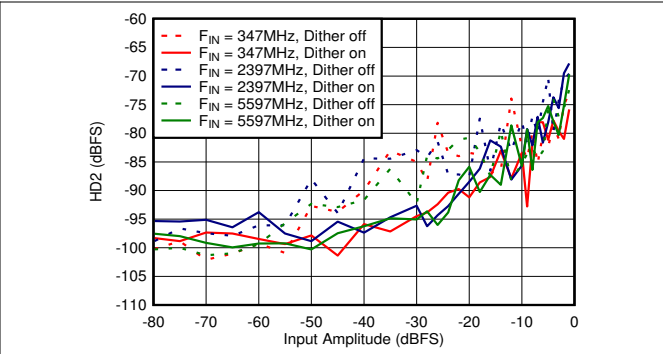
Figure 5-62. DES Mode: HD2 vs Input Amplitude and Dither
