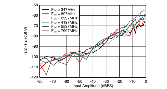
Figure 5-65. DES Mode: F_s/2 - F_{\text{IN}} vs Input Amplitude and Frequency
