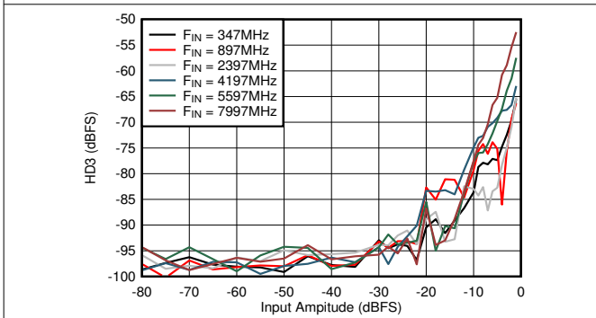
Figure 5-63. DES Mode: HD3 vs Input Amplitude and Frequency
