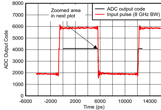
5-146. Pulse Overdrive Recovery
