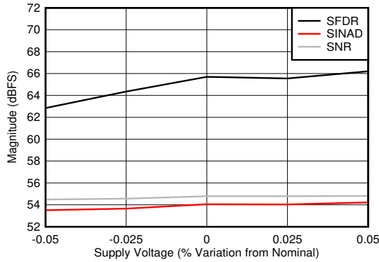
5-95. Dual Channel Mode: SNR, SINAD and SFDR vs Supply Voltage
