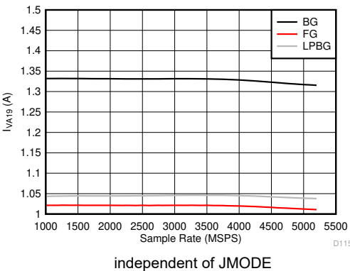
5-131. Dual Channel Mode: I_{VA19} vs Sample Rate
