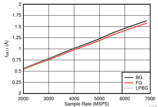
图 5-122. DES Mode: I_{VA11} vs Sample Rate
