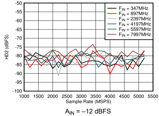
5-52. Dual Channel Mode: HD2 vs Sample Rate and Input Frequency
