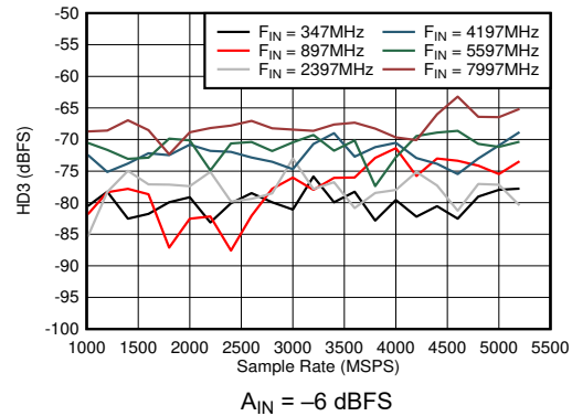
5-54. Dual Channel Mode: HD3 vs Sample Rate and Input Frequency
