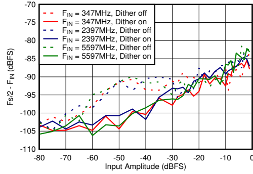
Figure 5-80. Dual Channel Mode: F_s/2 - F_{IN} vs Input Amplitude and Dither
