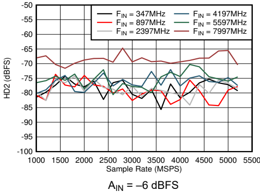
5-51. Dual Channel Mode: HD2 vs Sample Rate and Input Frequency
