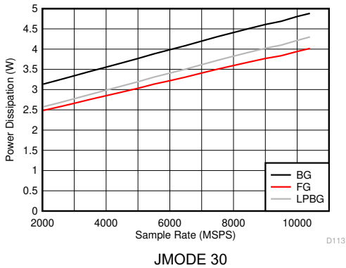
5-129. DES Mode: Power Dissipation vs Sample Rate
