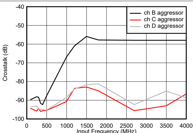
図 5-4. Crosstalk vs Input Frequency, Channel A victim
