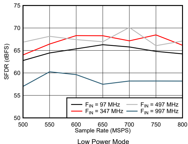
Figure 5-55. SFDR vs Sample Rate in Low Power Mode
