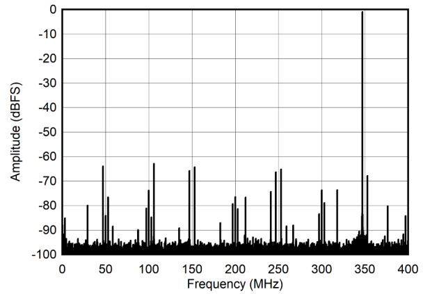
図 5-18. Single Tone FFT at 347 MHz and -1dBFS
