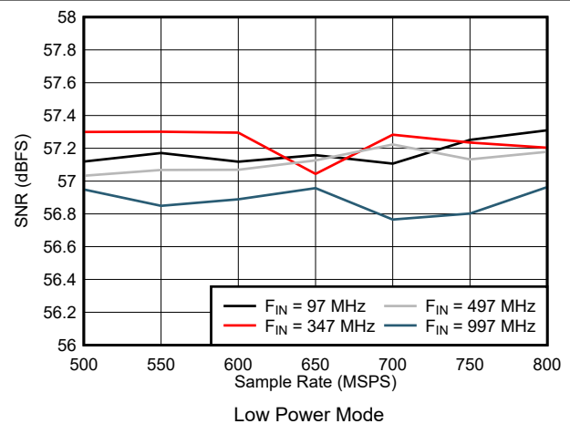
図 5-54. SNR vs Sample Rate in Low Power Mode
