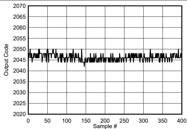
図 5-115. Background Calibration Core Transition (midscale)
