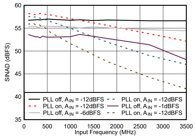
図 5-26. SINAD vs Input Frequency
