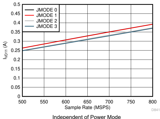
図 5-80. Quad Channel, I_{VD11} vs F_S for JMODES 0 - 3
