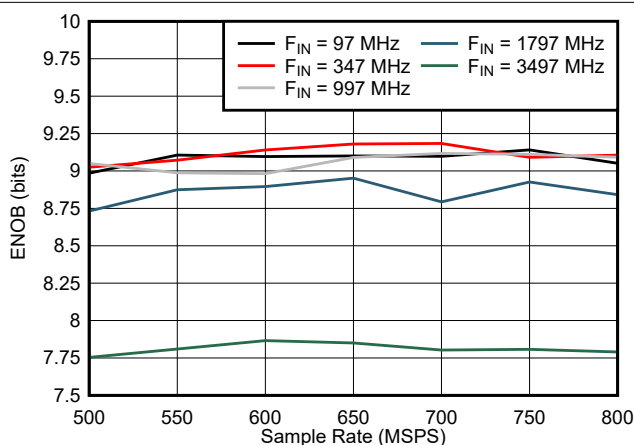
FIG 5-31. ENOB vs Sample Rate
