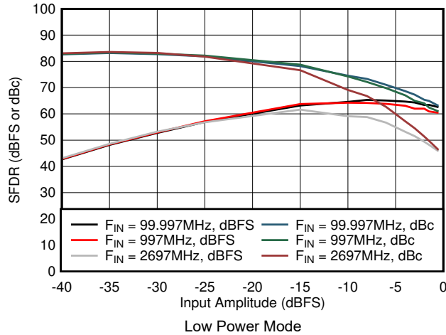
5-59. SFDR vs Input Amplitude in Low Power Mode
