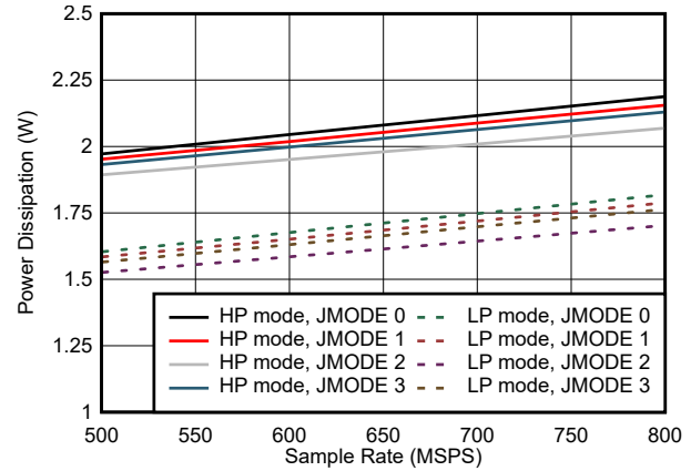
図 5-74. Quad Channel, Power Dissipation vs F_S for JMODES 0 - 3
