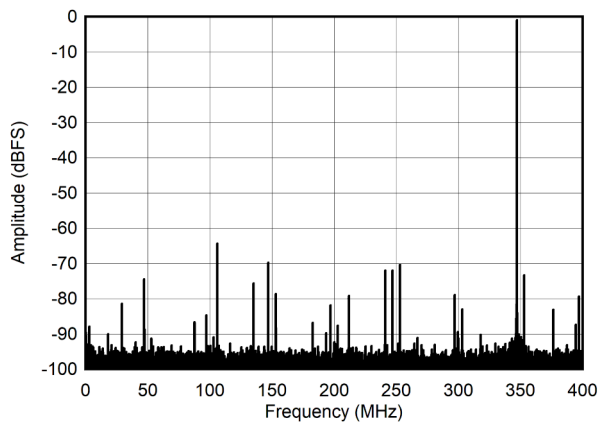
図 5-19. Single Tone FFT at 347 MHz and -1dBFS
