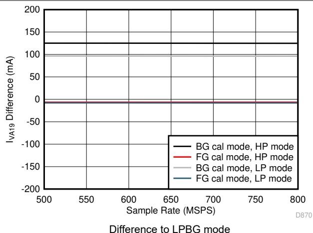
Figure 5-112. Single Channel, I_{VA19} vs F_S over Modes
