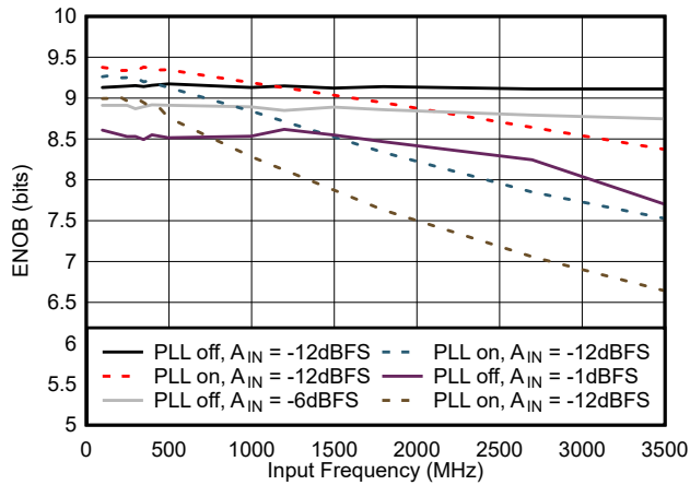
FIG 5-27. ENOB vs Input Frequency
