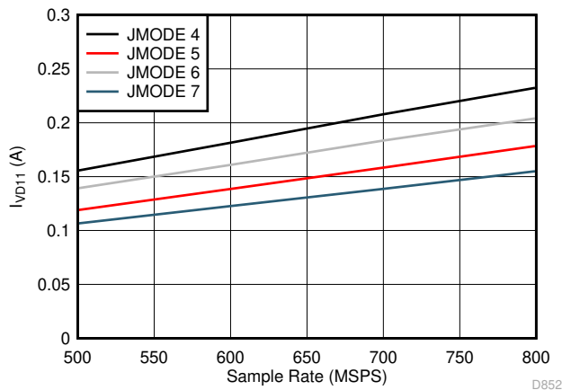
FIG 5-95. Dual Channel, I_{VD11} vs F_S for JMODES 4 - 7
