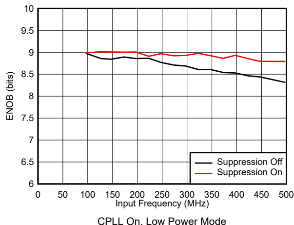
Figure 5-63. ENOB vs Input Frequency
