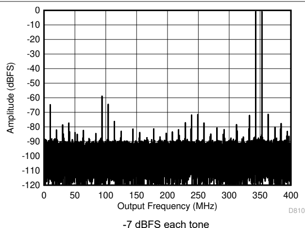
図 5-69. Two Tone FFT at 347 MHz in Low Power Mode
