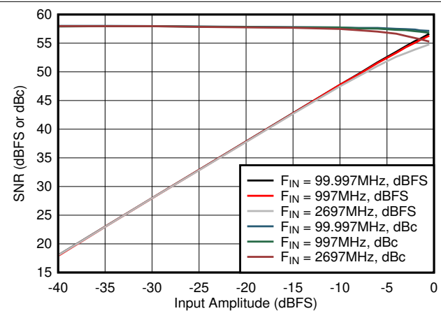
FIG 5-32. SNR vs Input Amplitude
