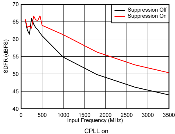
図 5-35. SFDR vs Input Frequency and Suppression
