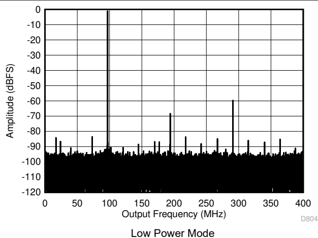
図 5-11. Single Tone FFT at 897 MHz and -1dBFS
