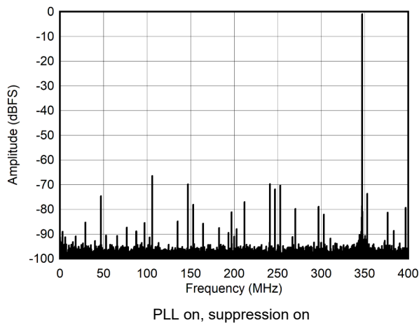
図 5-15. Single Tone FFT at 347 MHz and -1dBFS
