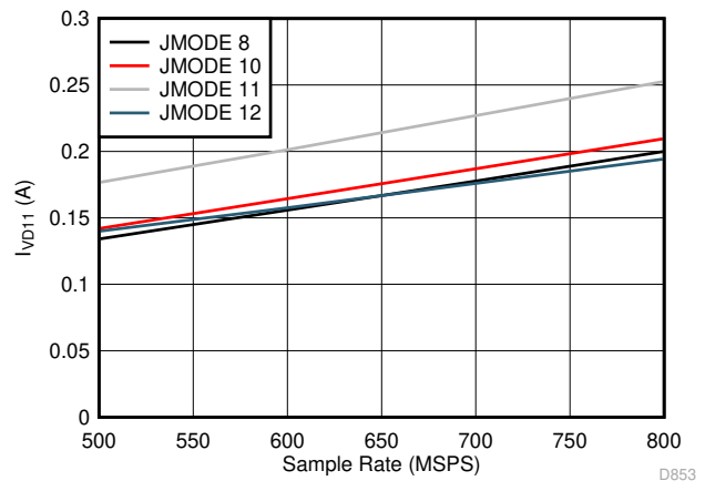
FIG 5-96. Dual Channel, I_{VD11} vs F_S for JMODES 8 - 12
