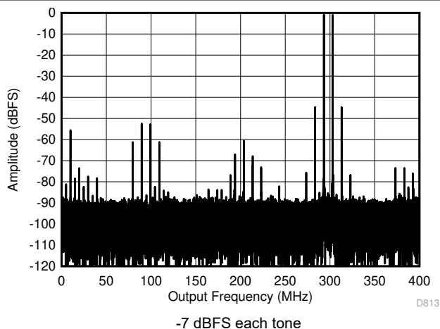
Figure 5-68. Two Tone FFT at 3498 MHz
