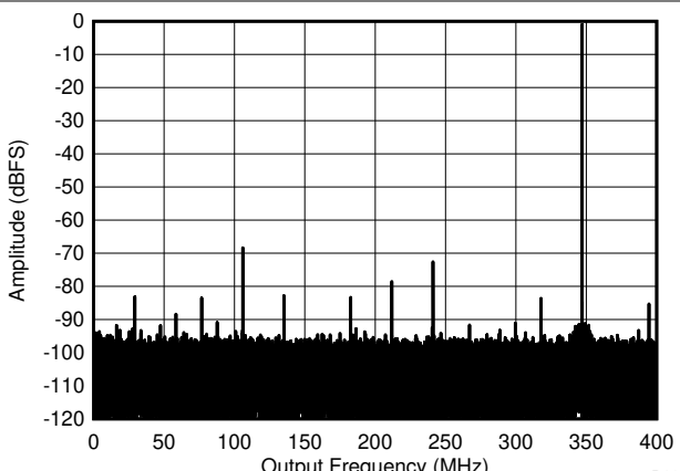
図 5-6. Single Tone FFT at 347 MHz and -1dBFS
