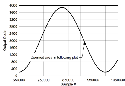
図 5-115. Background Calibration Core Transition (midscale)
