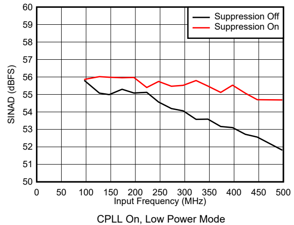
5-62. SINAD vs Input Frequency
