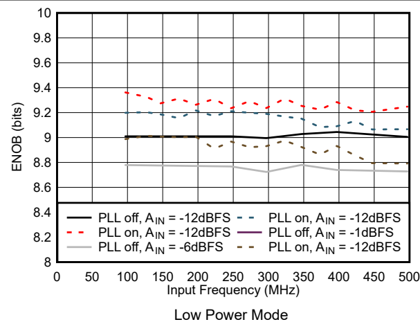
図 5-53. ENOB vs Input Frequency in Low Power Mode
