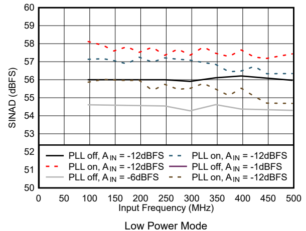
図 5-52. SINAD vs Input Frequency in Low Power Mode
