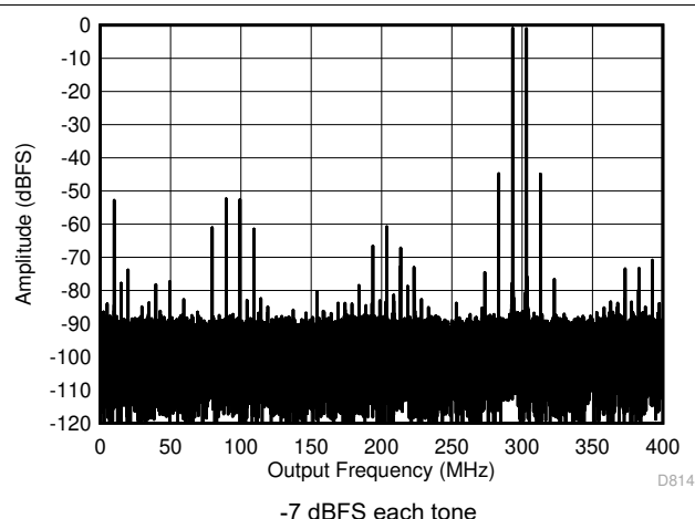
図 5-71. Two Tone FFT at 3498 MHz in Low Power Mode
