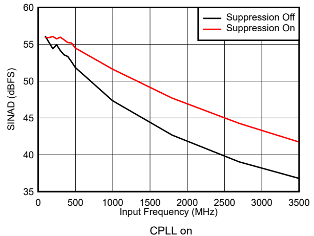
図 5-36. SINAD vs Input Frequency and Suppression
