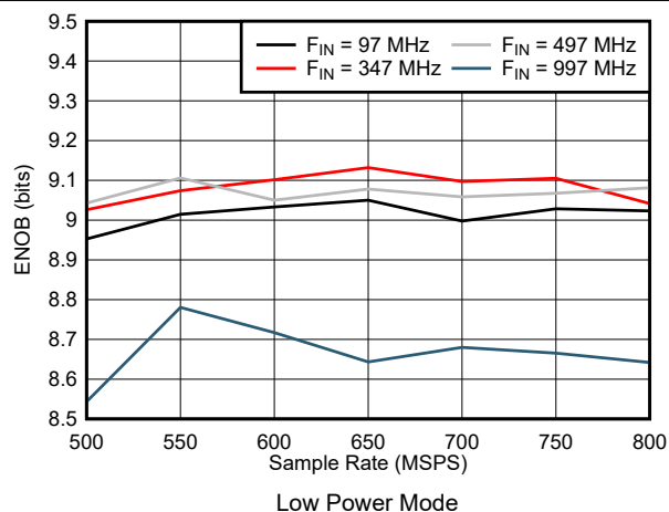
Figure 5-57. ENOB vs Sample Rate in Low Power Mode
