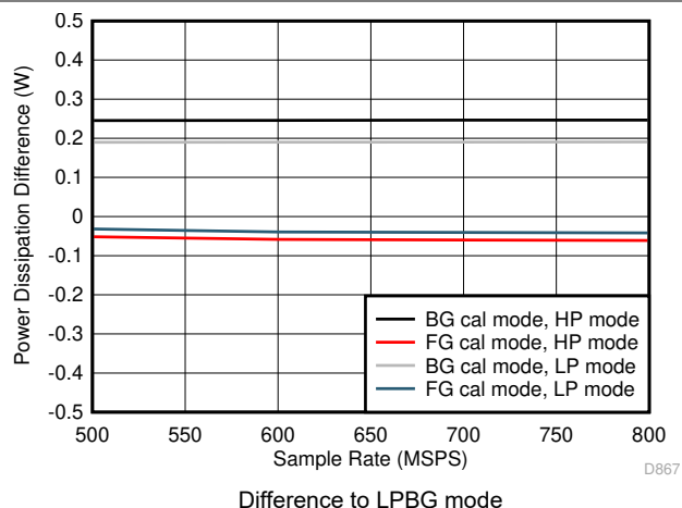
Figure 5-111. Single Channel, Power Dissipation vs F_S over Modes
