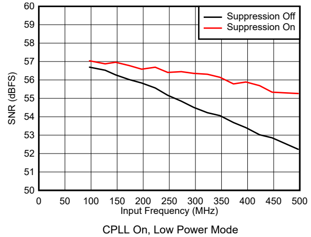
5-60. SNR vs Input Frequency
