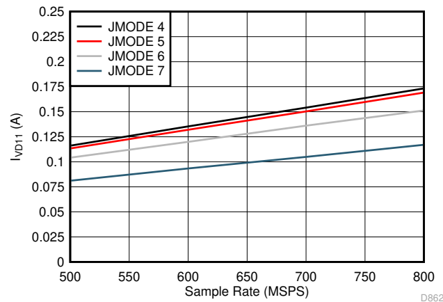
Figure 5-108. Single Channel, I_{VD11} vs F_S for JMODES 4 - 7
