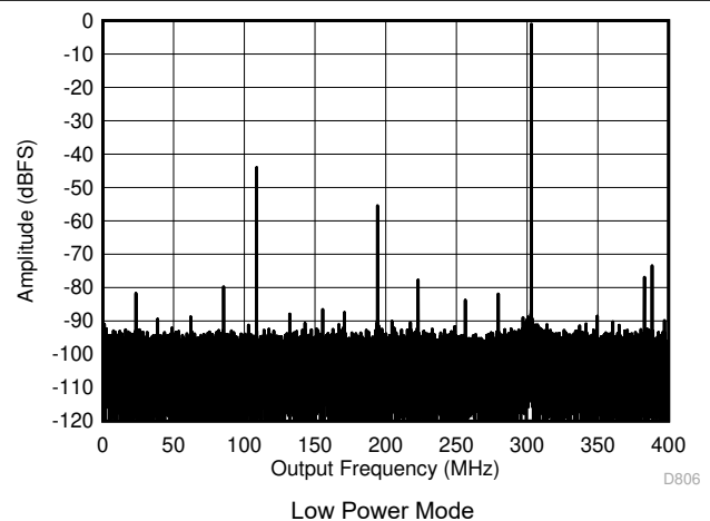
図 5-12. Single Tone FFT at 2097 MHz and -1dBFS
