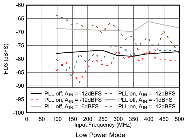
図 5-51. HD3 vs Input Frequency in Low Power Mode
