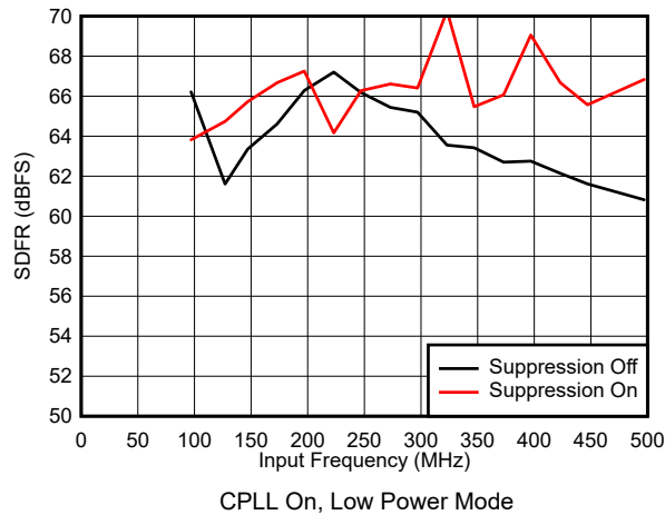
5-61. SFDR vs Input Frequency
