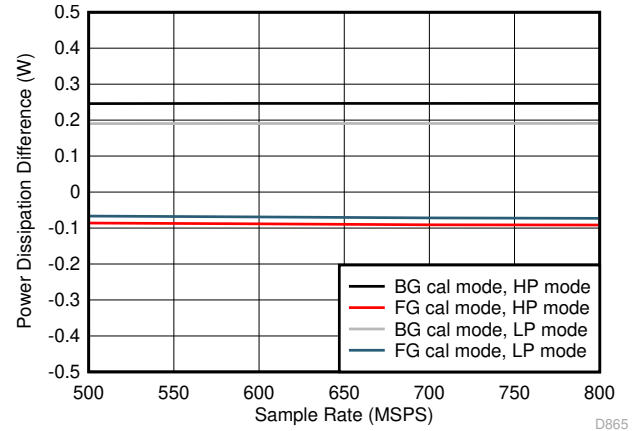
Figure 5-84. Quad Channel, Power Dissipation vs F_S over Modes
