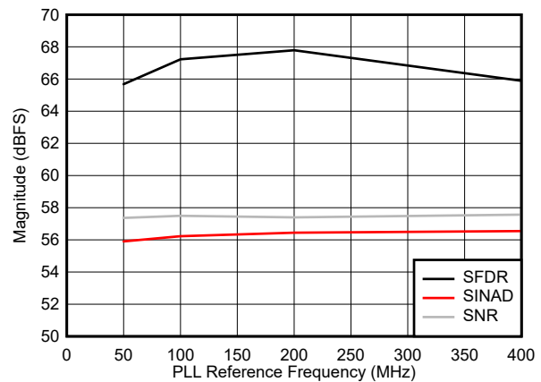
図 5-42. SNR, SFDR and SINAD vs Reference Frequency with PLL on
