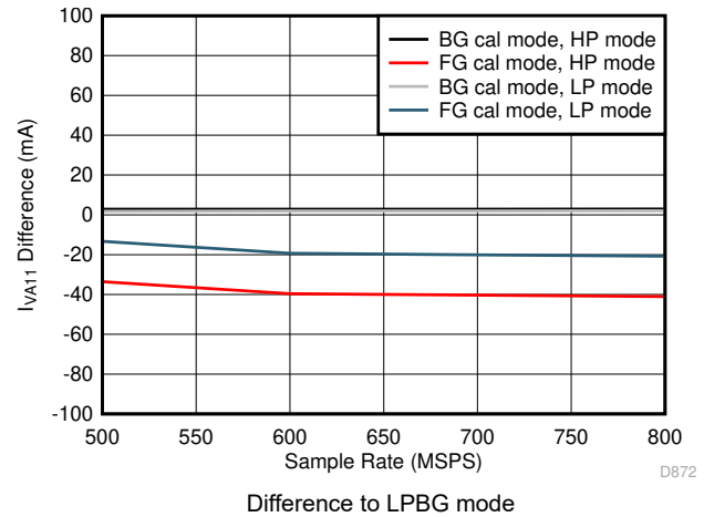
Figure 5-100. Dual Channel, I_{VA11} vs F_S over Modes
