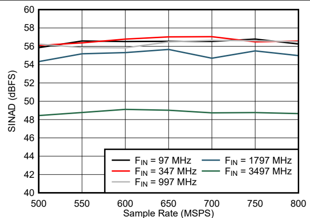
FIG 5-30. SINAD vs Sample Rate
