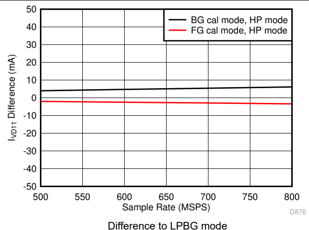
Figure 5-114. Single Channel, I_{VD11} vs F_S over Modes
