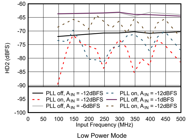
図 5-50. HD2 vs Input Frequency in Low Power Mode
