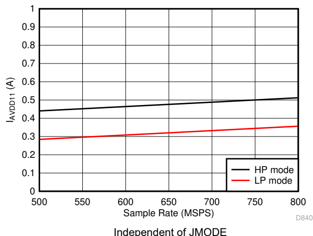
図 5-79. Quad Channel, I_{VA11} vs F_S
