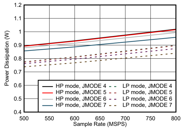
Figure 5-102. Single Channel, Power Dissipation vs F_S for JMODES 4 - 7
