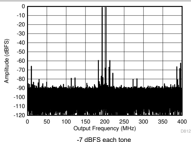
図 5-70. Two Tone FFT at 1798 MHz in Low Power Mode
