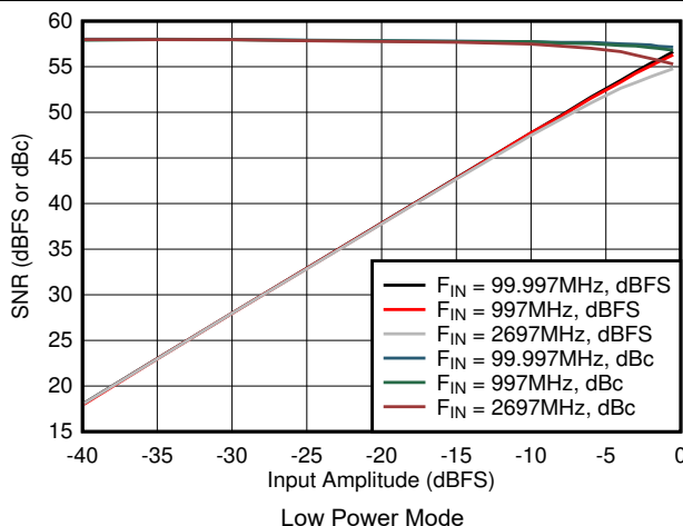
Figure 5-58. SNR vs Input Amplitude in Low Power Mode
