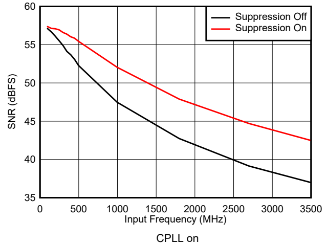
図 5-34. SNR vs Input Frequency and Suppression
