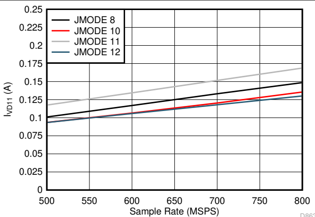
Figure 5-109. Single Channel, I_{VD11} vs F_S for JMODES 8 - 12
