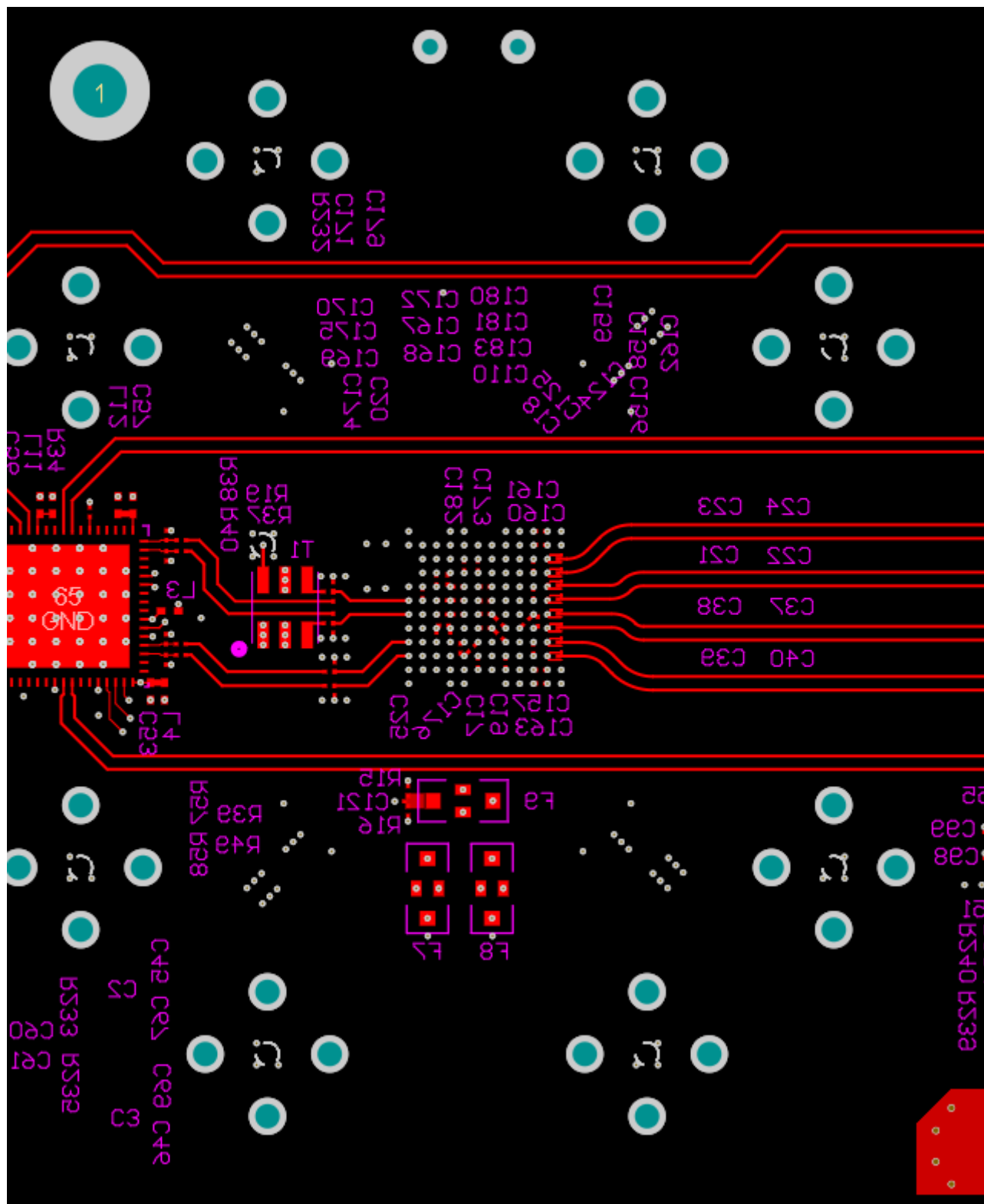
図 7-7. Bottom Layer Routing: CLK±, SYSREF and D[7:4]± Routing
