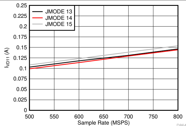
Figure 5-110. Single Channel, I_{VD11} vs F_S for JMODES 13 - 15
