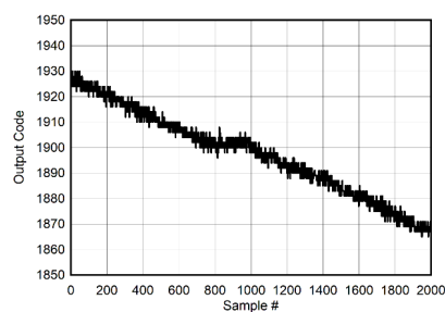
図 5-116. Background Calibration Core Transition (voltage offset)
