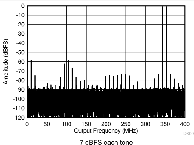
Figure 5-66. Two Tone FFT at 347 MHz
