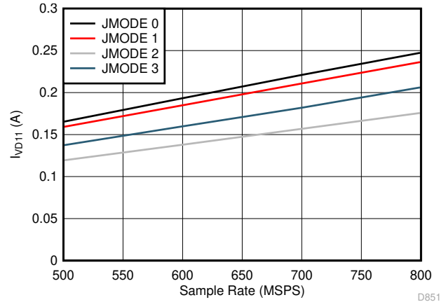
FIG 5-94. Dual Channel, I_{VD11} vs F_S for JMODES 0 - 3
