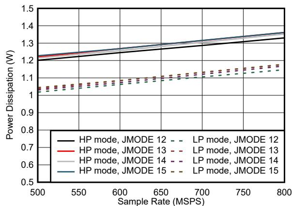
Figure 5-91. Dual Channel, Power Dissipation vs F_S for JMODES 12 - 15
