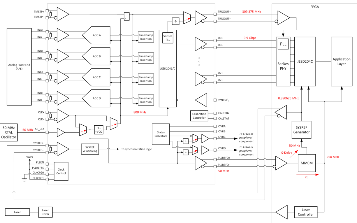
7-1. Typical Configuration for a LiDAR Digitizer
