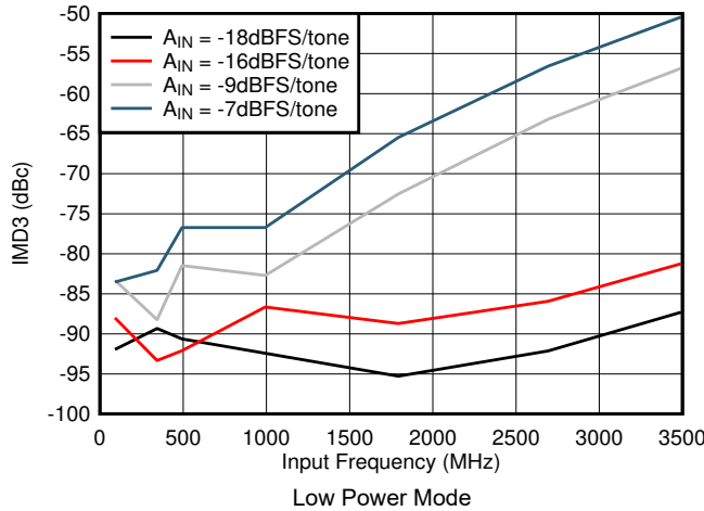
図 5-73. IMD3 vs Input Frequency in Low Power Mode
