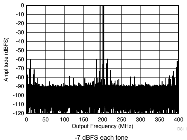
Figure 5-67. Two Tone FFT at 1798 MHz
