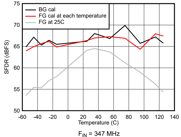
Figure 5-44. SFDR vs Temperature
