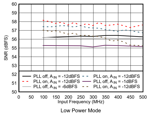
Figure 5-48. SNR vs Input Frequency in Low Power Mode
