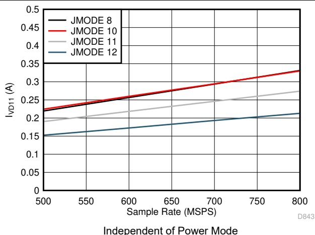
図 5-82. Quad Channel, I_{VD11} vs F_S for JMODES 8-12
