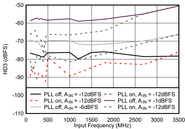
図 5-25. HD3 vs Input Frequency
