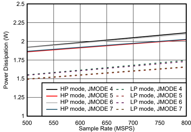
図 5-75. Quad Channel, Power Dissipation vs F_S for JMODES 4 - 7
