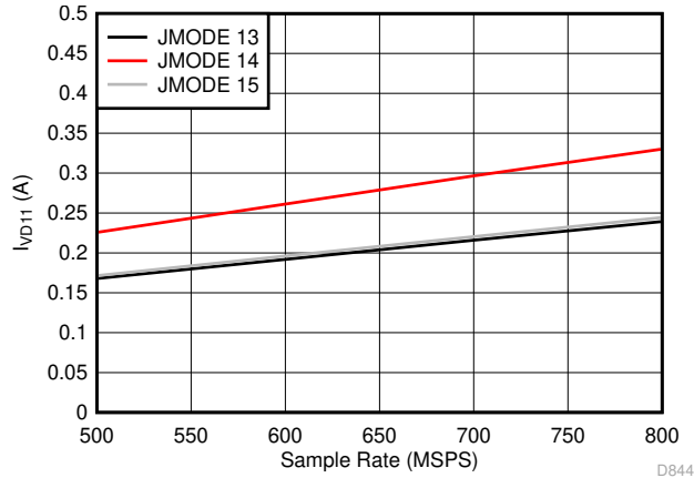
Figure 5-83. Quad Channel, I_{VD11} vs F_S for JMODES 13-15
