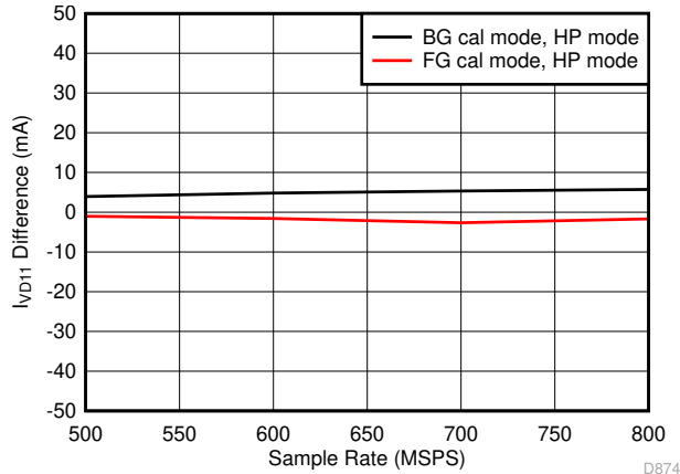
Figure 5-87. Quad Channel, I_{VD11} vs F_S over Modes
