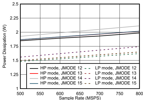
図 5-77. Quad Channel, Power Dissipation vs F_S for JMODES 12 - 15
