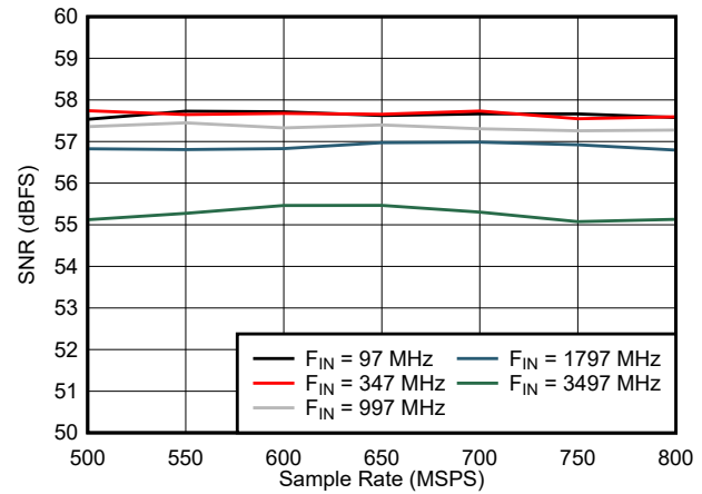
FIG 5-28. SNR vs Sample Rate
