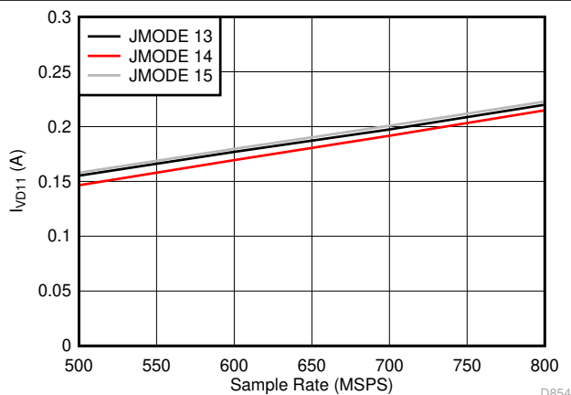
FIG 5-97. Dual Channel, I_{VD11} vs F_S for JMODES 13 - 15
