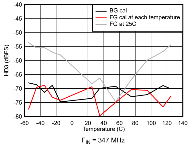
Figure 5-46. HD3 vs Temperature
