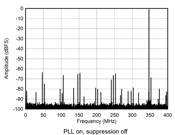
図 5-14. Single Tone FFT at 347 MHz and -1dBFS
