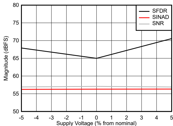
Figure 5-64. SNR, SFDR and SINAD vs Supply Voltage
