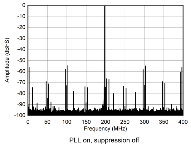
図 5-16. Single Tone FFT at 997 MHz and -1dBFS
