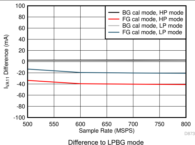
Figure 5-113. Single Channel, I_{VA11} vs F_S over Modes
