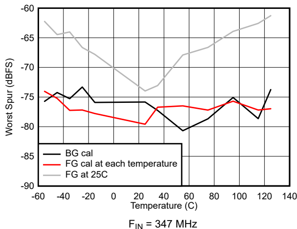
Figure 5-47. worst non-HD spur vs Temperature
