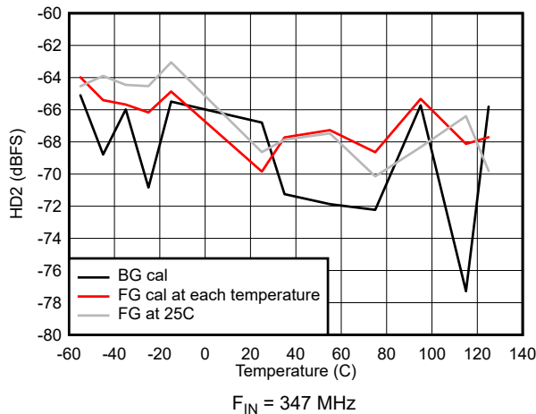
Figure 5-45. HD2 vs Temperature
