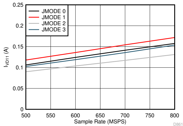
Figure 5-107. Single Channel, I_{VD11} vs F_S for JMODES 0 - 3
