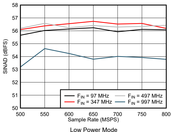
Figure 5-56. SINAD vs Sample Rate in Low Power Mode
