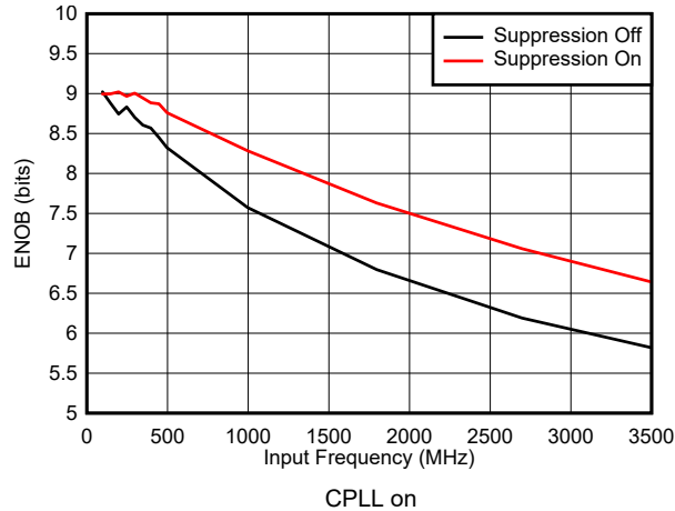
図 5-37. ENOB vs Input Frequency and Suppression
