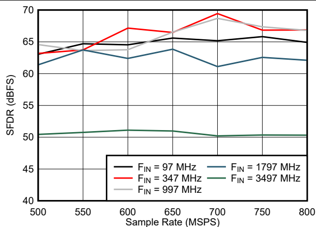
FIG 5-29. SFDR vs Sample Rate
