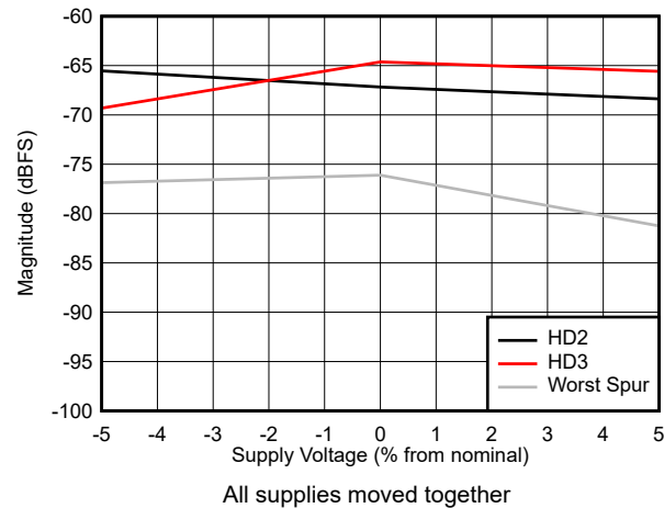
図 5-39. HD2, HD3 and worst non-HD vs Supply Voltage
