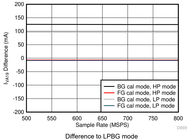
Figure 5-99. Dual Channel, I_{VA19} vs F_S over Modes
