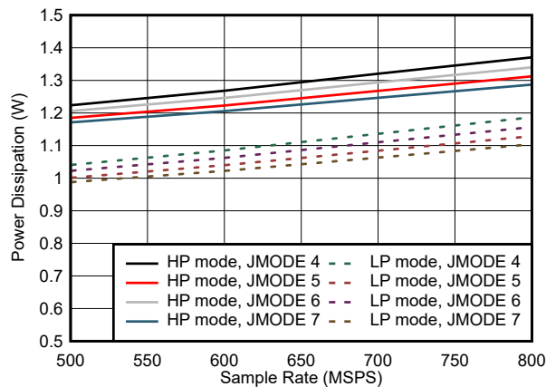
Figure 5-89. Dual Channel, Power Dissipation vs F_S for JMODES 4 - 7
