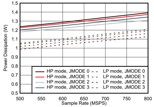
Figure 5-88. Dual Channel, Power Dissipation vs F_S for JMODES 0 - 3
