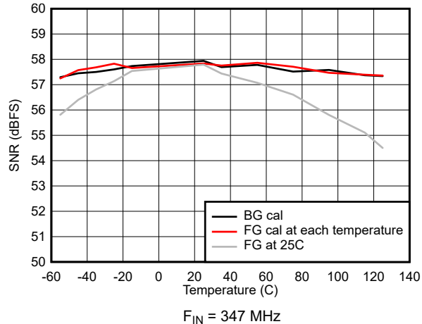
Figure 5-43. SNR vs Temperature
