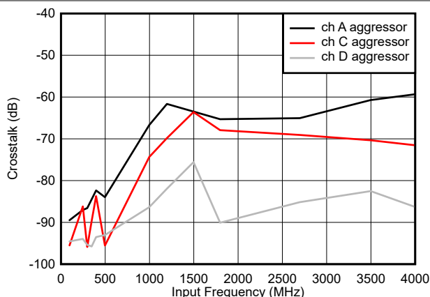
図 5-5. Crosstalk vs Input Frequency, Channel B victim
