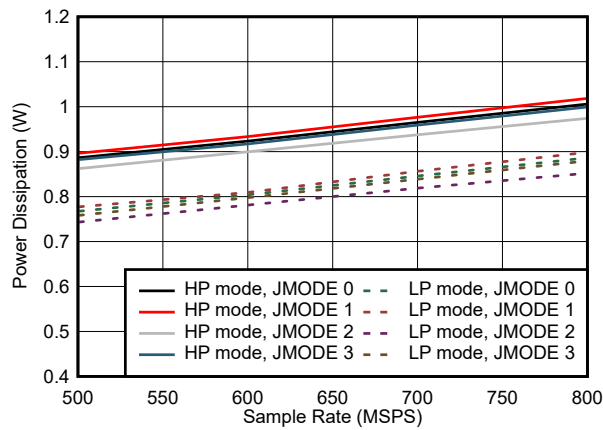
Figure 5-101. Dual Channel, Power Dissipation vs F_S for JMODES 0 - 3
