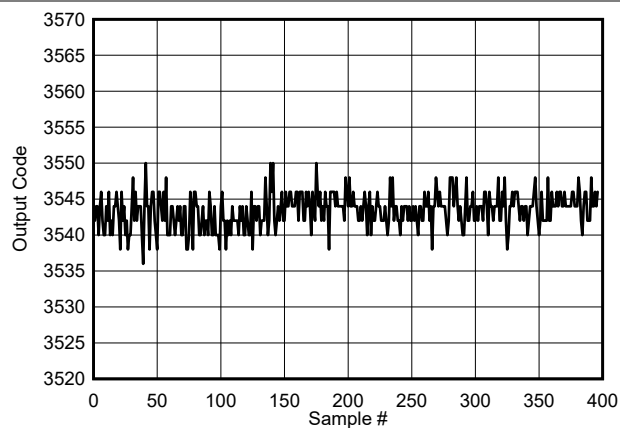
図 5-116. Background Calibration Core Transition (voltage offset)
