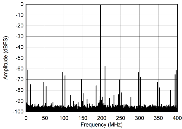
図 5-21. Single Tone FFT at 997 MHz and -1dBFS
