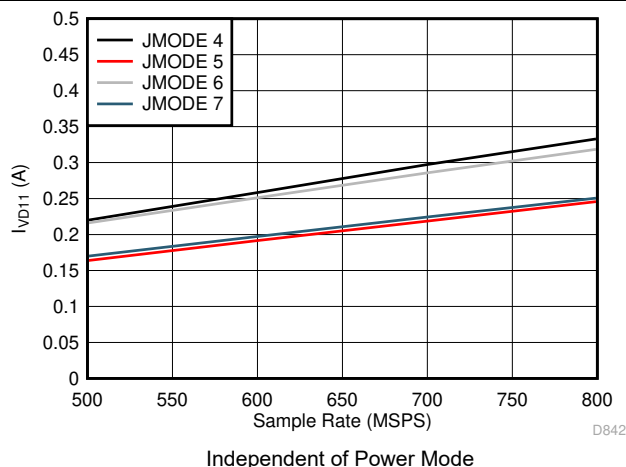
図 5-81. Quad Channel, I_{VD11} vs F_S for JMODES 4 - 7
