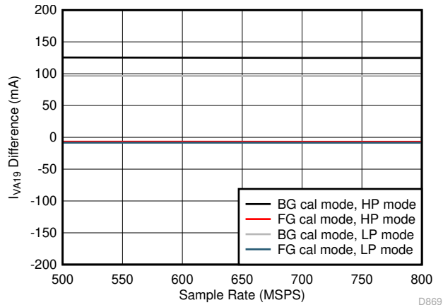
Figure 5-99. Dual Channel, I_{VA19} vs F_S over Modes
