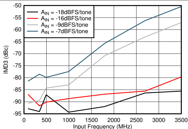
图 5-72. IMD3 vs Input Frequency
