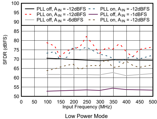
Figure 5-49. SFDR vs Input Frequency in Low Power Mode
