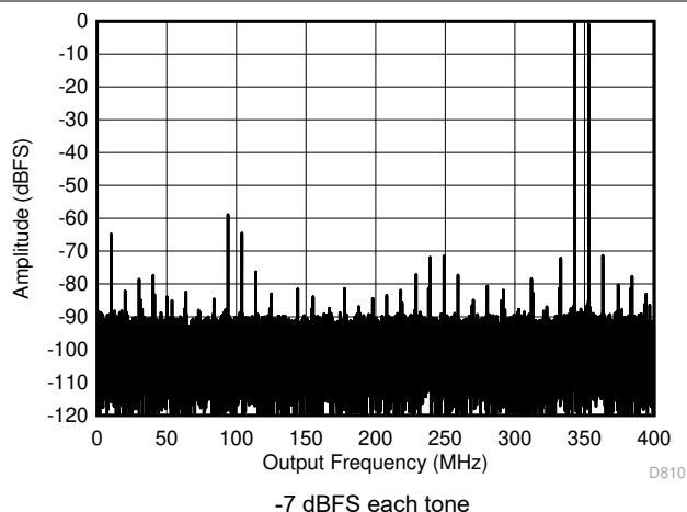
图 5-69. Two Tone FFT at 347 MHz in Low Power Mode
