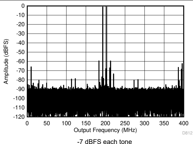
图 5-70. Two Tone FFT at 1798 MHz in Low Power Mode
