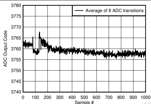
BG Calibration, input voltage offset ~ 90% of fullscale, ADC_SRC_DLY=31, MUX_DLY=30
