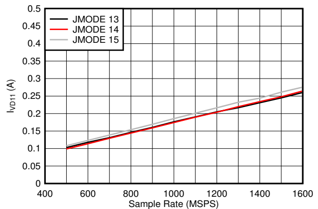
Figure 6-108. Single Channel, I_{VD11} vs F_S and JMODE 13 - 15
