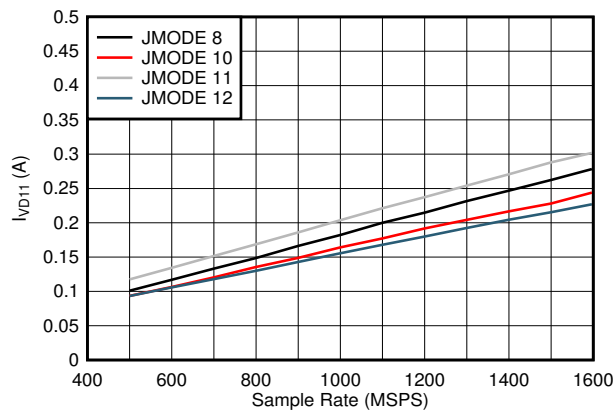
Figure 6-107. Single Channel, I_{VD11} vs F_S and JMODE 8 - 12
