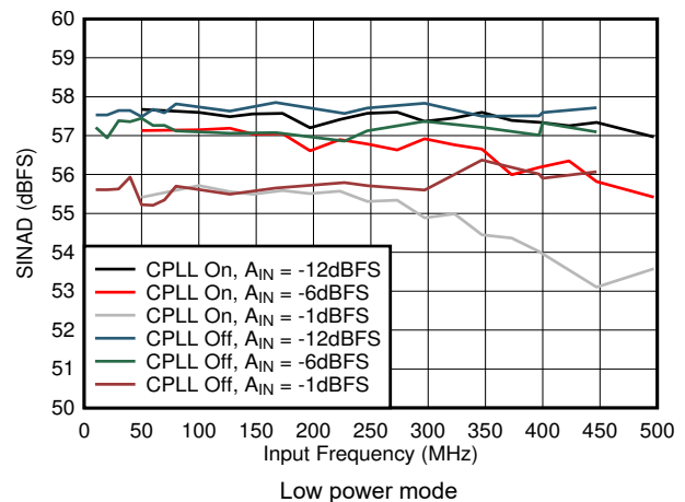
Figure 6-56. SINAD vs A_{IN} and C-PLL
