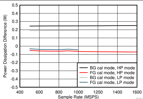
Figure 6-109. Quad Channel, Power Dissipation Change with Calibration Mode
