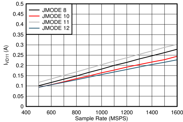
図 5-107. Single Channel, I_{VD11} vs F_S and JMODE 8 - 12
