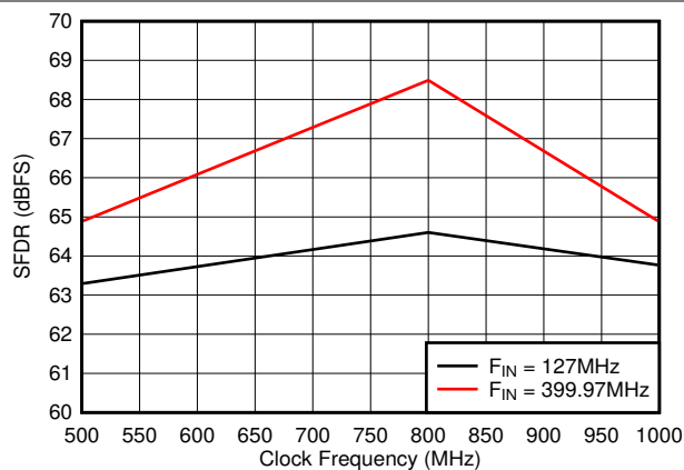
Figure 5-29. SFDR vs Sample Rate
