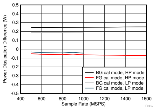
図 5-109. Quad Channel, Power Dissipation Change with Calibration Mode
