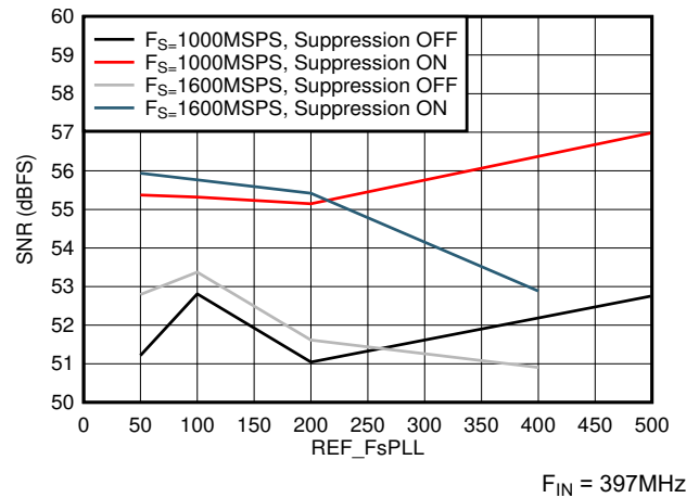
図 5-38. SNR vs F_{REF} and Suppression
