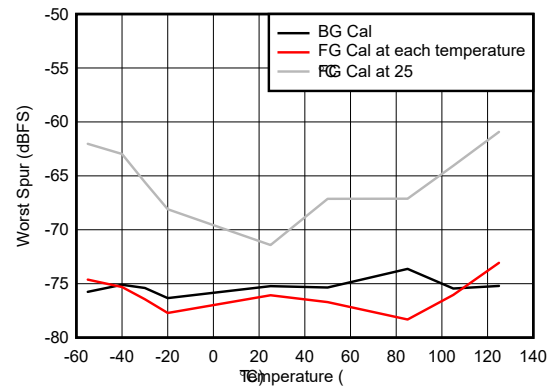
図 5-68. Worst Spur vs Temperature
