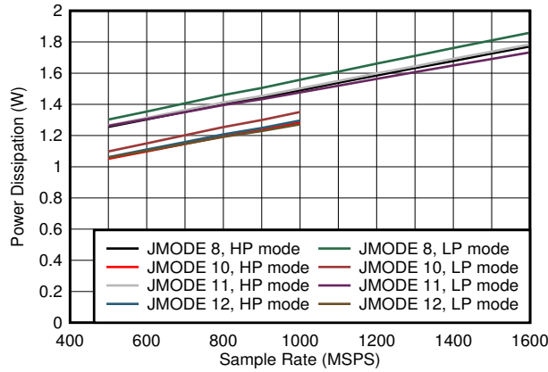
図 5-91. Dual Channel, Power Dissipation vs F_s and JMODE 8 - 12
