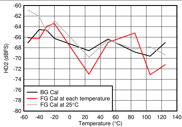
Figure 5-66. HD2 vs Temperature
