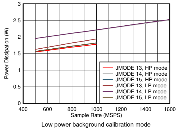
図 5-82. Quad Channel, Power Dissipation vs F_s and JMODE 13 - 15
