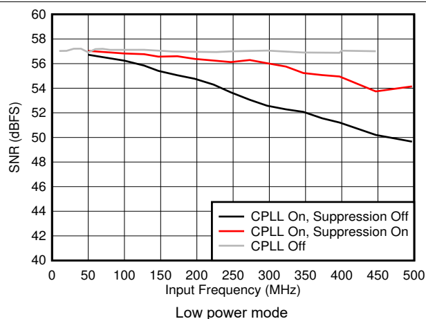
図 5-45. SNR vs F_{IN} and C-PLL modes
