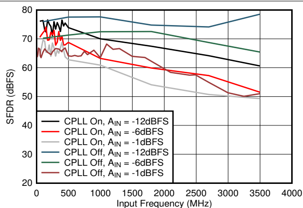
図 5-48. SFDR vs A_{IN} and C-PLL
