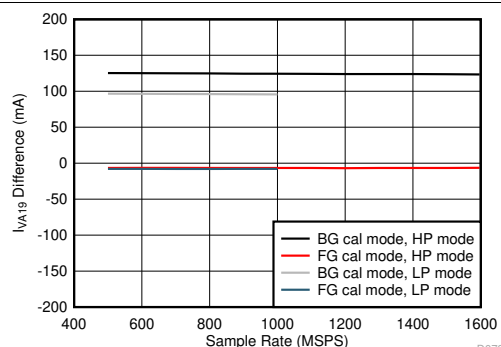
5-112. Quad Channel, I_{VA19} Change with Calibration Mode
