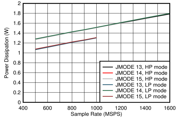
図 5-92. Dual Channel, Power Dissipation vs F_s and JMODE 13 - 15
