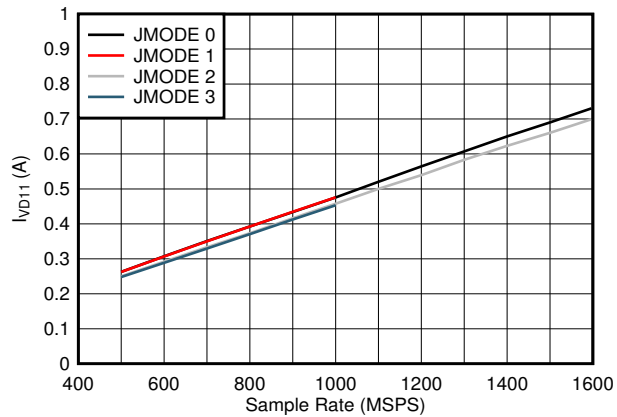
図 5-85. Quad Channel, I_{VD11} vs F_S and JMODE 0 - 3
