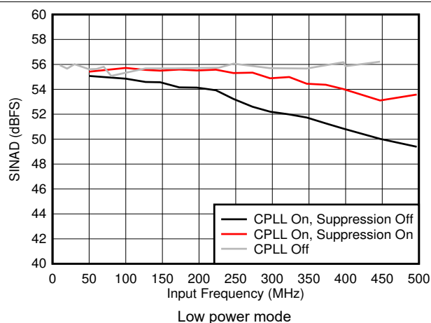
図 5-46. SINAD vs F_{IN} and C-PLL modes
