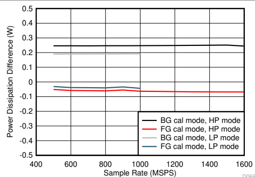
5-110. Dual Channel, Power Dissipation Change with Calibration Mode
