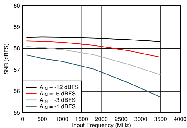
5-18. SNR vs Input Frequency
