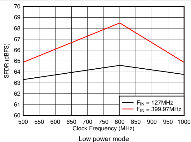
図 5-27. SFDR vs Sample Rate
