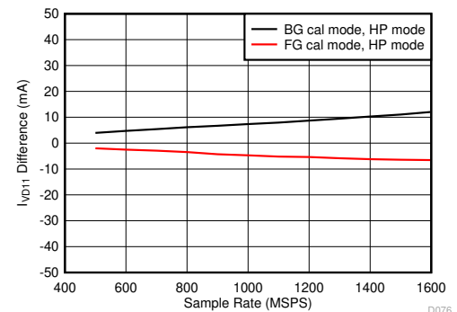
5-118. Quad Channel, I_{VD11} Change with Calibration Mode
