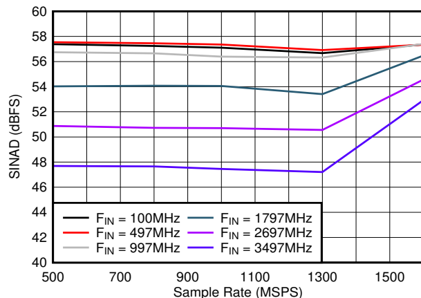
図 5-25. SINAD vs Sample Rate
