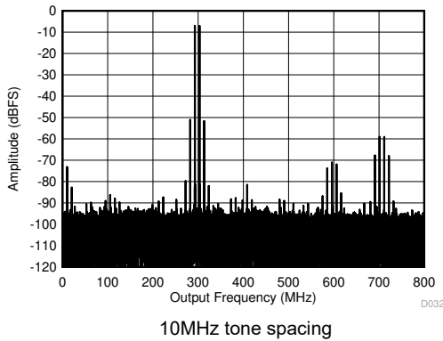
図 5-71. Two Tone FFT at 3498MHz
