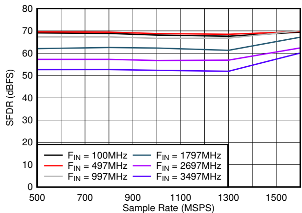
図 5-23. SFDR vs Sample Rate
