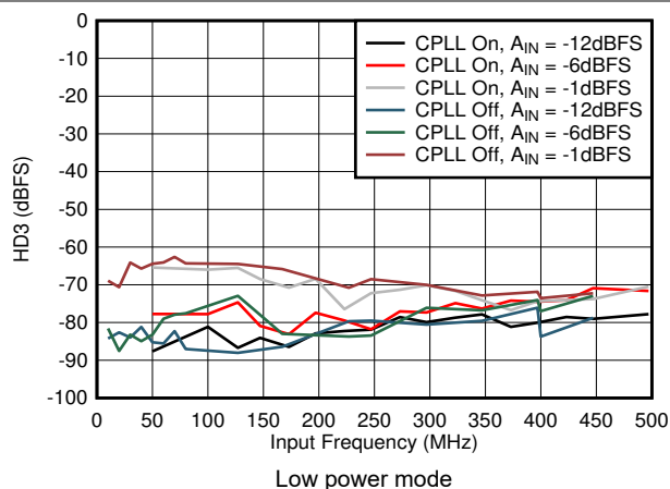
Figure 5-59. HD3 vs A_{IN} and C-PLL
