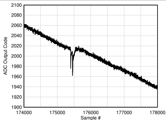
図 5-127. Background Calibration Core Transition (AC Signal Zoomed)
