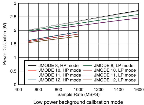
図 5-81. Quad Channel, Power Dissipation vs F_s and JMODE 8 - 12
