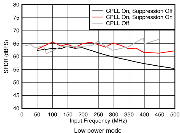
図 5-44. SFDR vs F_{IN} and C-PLL modes
