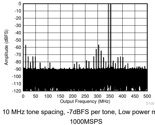
図 5-72. Two Tone FFT at 348 MHz
