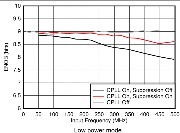
図 5-47. ENOB vs F_{IN} and C-PLL modes
