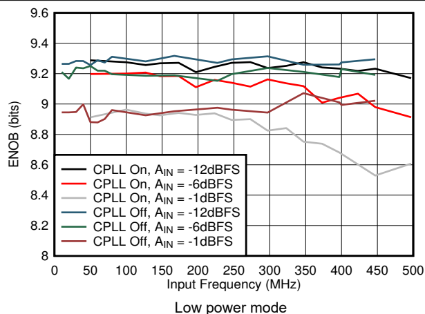
Figure 5-57. ENOB vs A_{IN} and C-PLL
