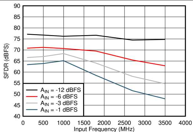
5-17. SFDR vs Input Frequency
