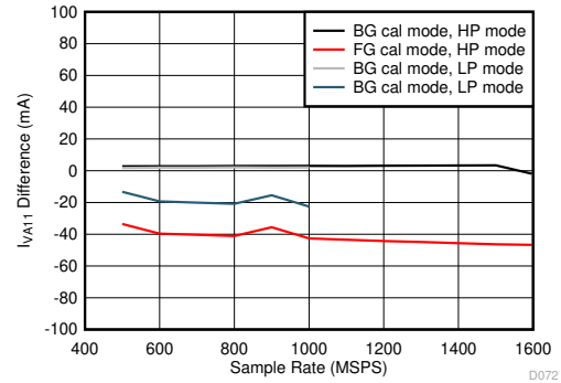
5-116. Dual Channel, I_{VA11} Change with Calibration Mode
