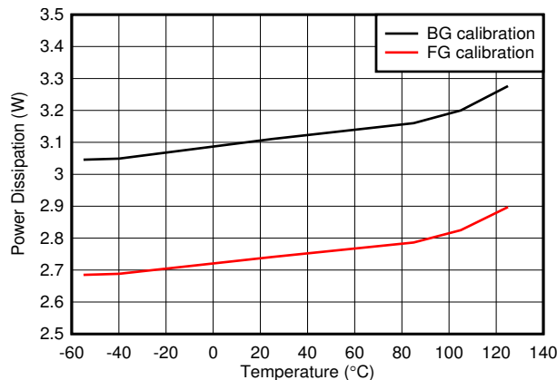
5-121. Quad Channel, Power Dissipation vs Temperature
