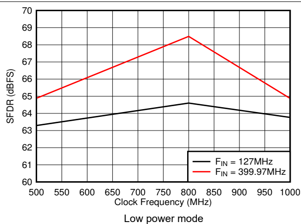
図 5-29. SFDR vs Sample Rate
