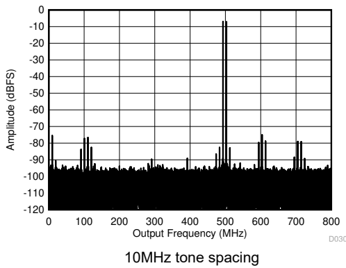
図 5-69. Two Tone FFT at 498MHz
