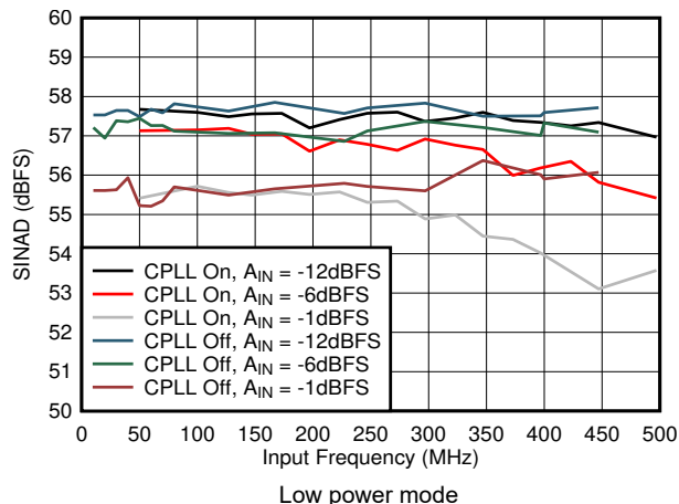
Figure 5-56. SINAD vs A_{IN} and C-PLL
