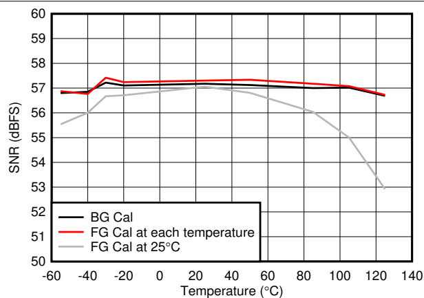
Figure 5-64. SNR vs Temperature
