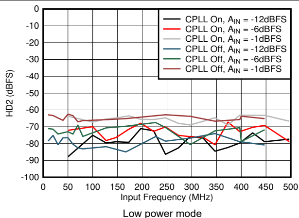
Figure 5-58. HD2 vs A_{IN} and C-PLL
