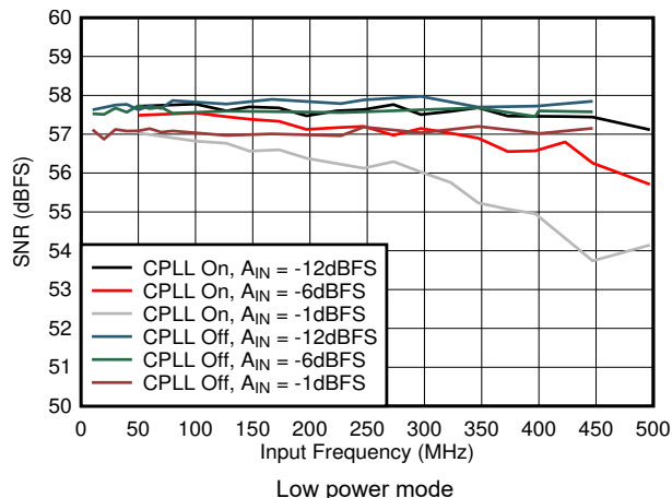
Figure 5-55. SNR vs A_{IN} and C-PLL
