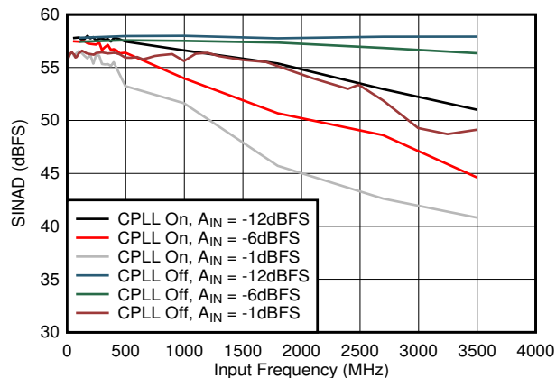
図 5-50. SINAD vs A_{IN} and C-PLL
