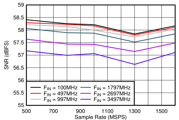
図 5-24. SNR vs Sample Rate
