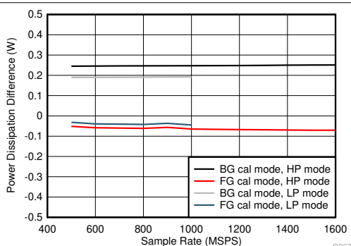
5-109. Quad Channel, Power Dissipation Change with Calibration Mode
