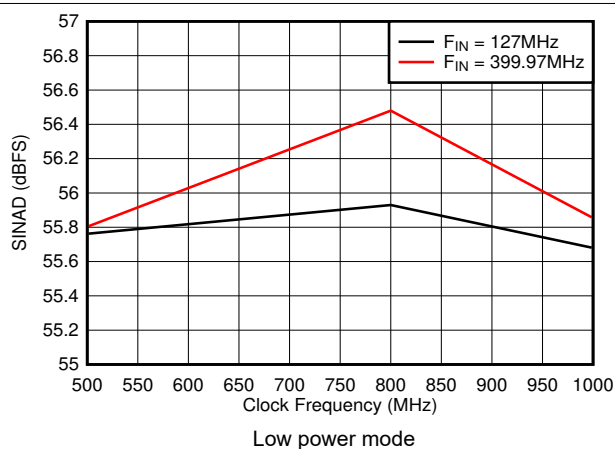
図 5-30. SINAD vs Sample Rate
