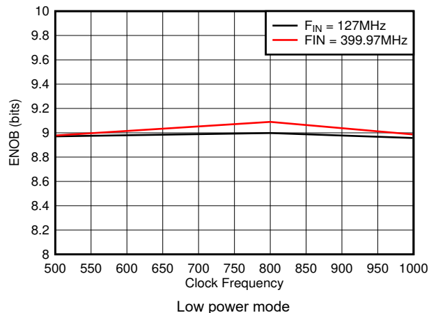
図 5-31. ENOB vs Sample Rate
