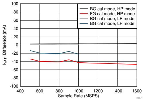
5-115. Quad Channel, I_{VA11} Change with Calibration Mode
