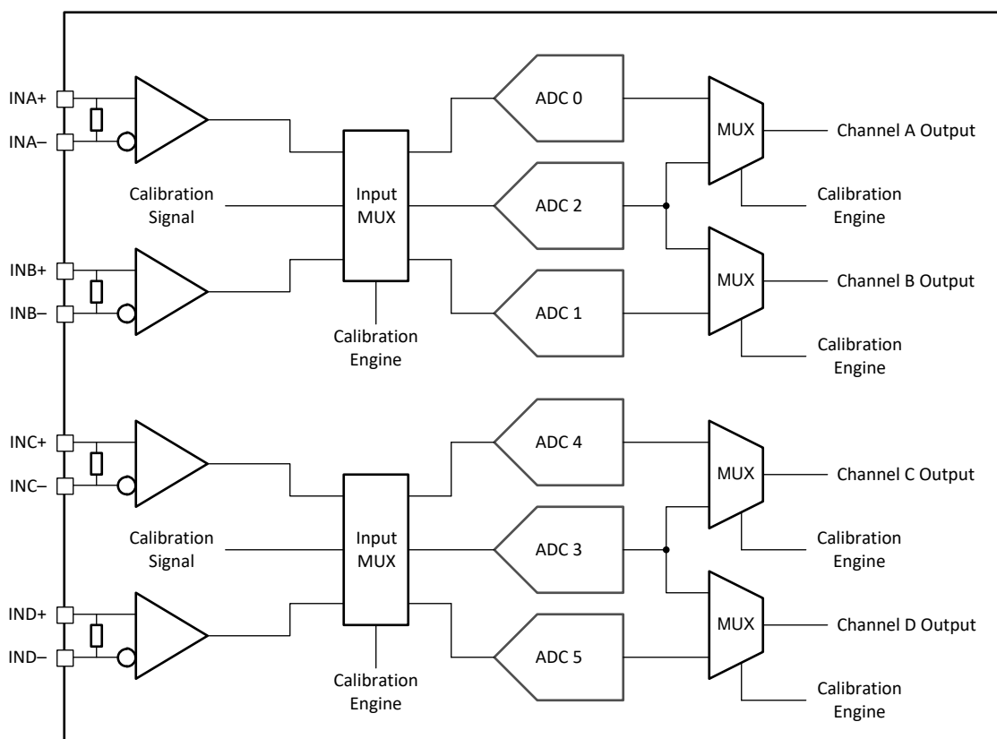
図 6-15. Quad Channel Calibration System Block Diagram
