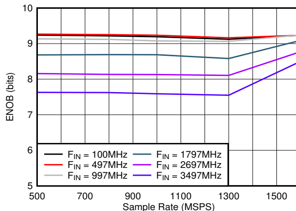
図 5-26. ENOB vs Sample Rate
