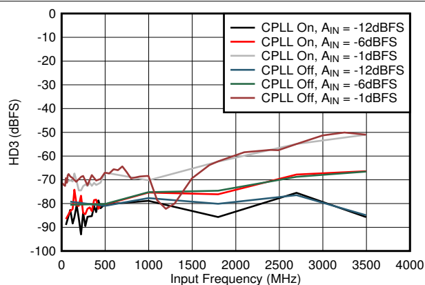
図 5-53. HD3 vs A_{IN} and C-PLL
