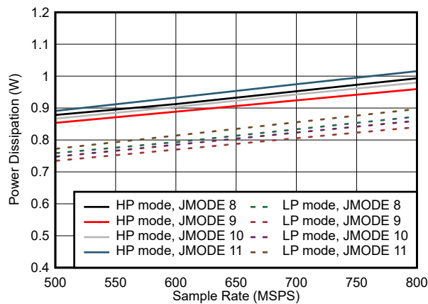
図 5-103. Single Channel, Power Dissipation vs F_S for JMODES 8 - 11
