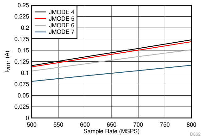
FIG 5-108. Single Channel, I_{VD11} vs F_S for JMODES 4 - 7
