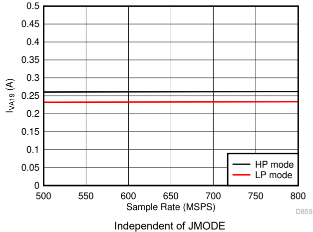
FIG 5-105. Single Channel, I_{VA19} vs F_S
