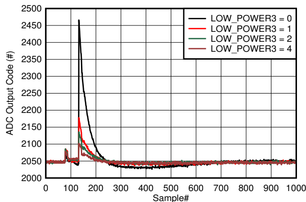
図 6-12. Background Calibration Core Transition In Low Power Mode
