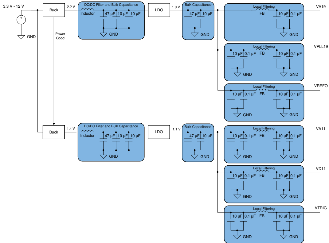
図 7-3. LDO Linear Regulator Approach Example
