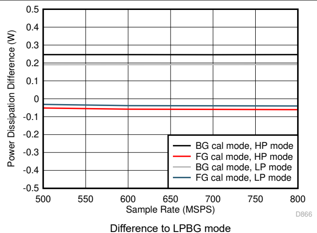
Figure 5-98. Dual Channel, Power Dissipation vs F_S over Modes
