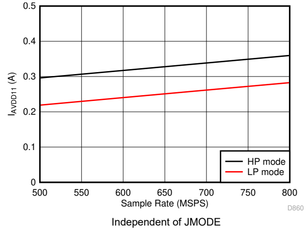
FIG 5-106. Single Channel, I_{VA11} vs F_S
