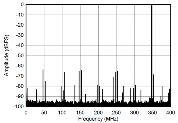
図 5-14. Single Tone FFT at 347 MHz and -1dBFS
