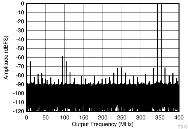
図 5-69. Two Tone FFT at 347 MHz in Low Power Mode
