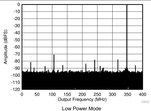
図 5-10. Single Tone FFT at 347 MHz and -1dBFS
