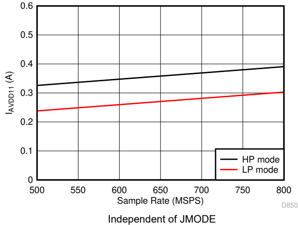
Figure 5-93. Dual Channel, I_{VA11} vs F_S
