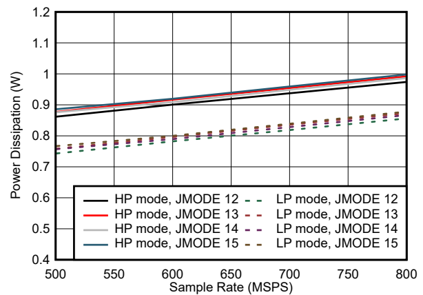
図 5-104. Single Channel, Power Dissipation vs F_S for JMODES 12 - 15
