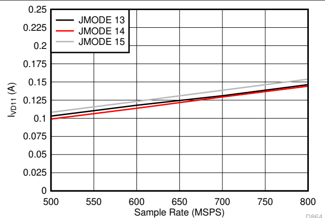
FIG 5-110. Single Channel, I_{VD11} vs F_S for JMODES 13 - 15
