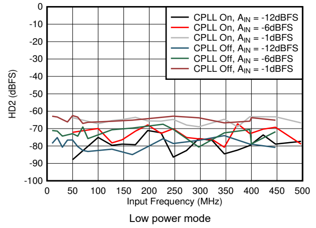
5-58. HD2 vs A_{IN} and C-PLL
