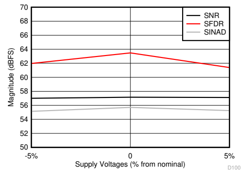
5-60. SNR, SFDR and SINAD vs Supply Voltage
