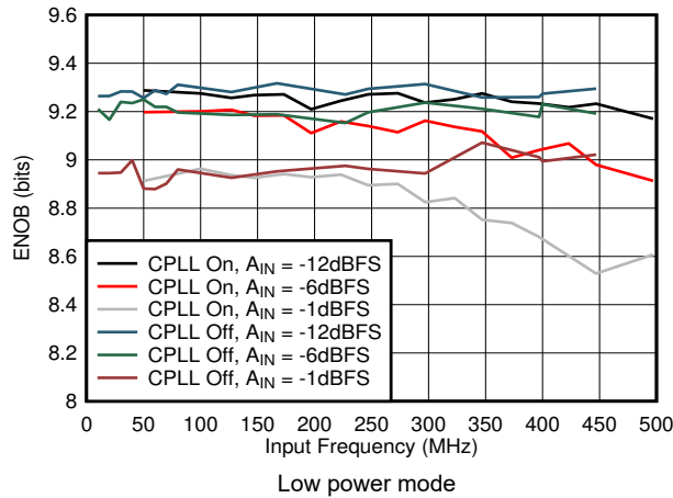
5-57. ENOB vs A_{IN} and C-PLL
