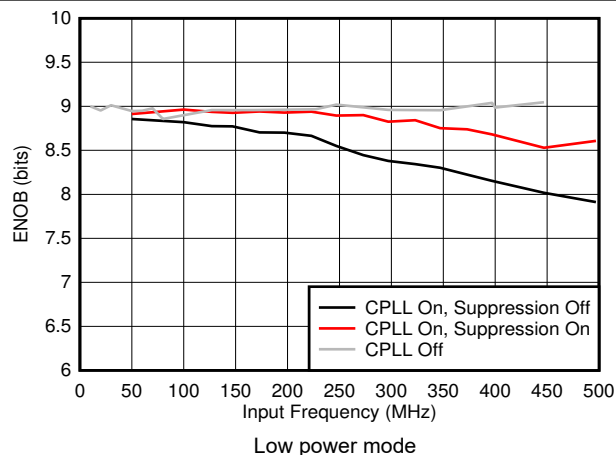
図 5-47. ENOB vs F_{IN} and C-PLL modes
