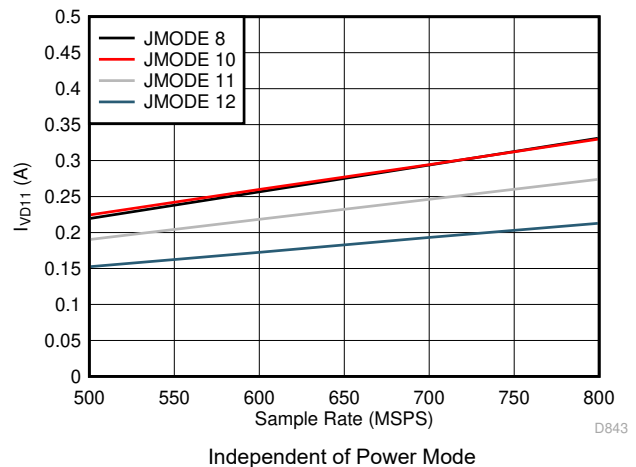
図 5-82. Quad Channel, I_{VD11} vs F_S for JMODES 8-12
