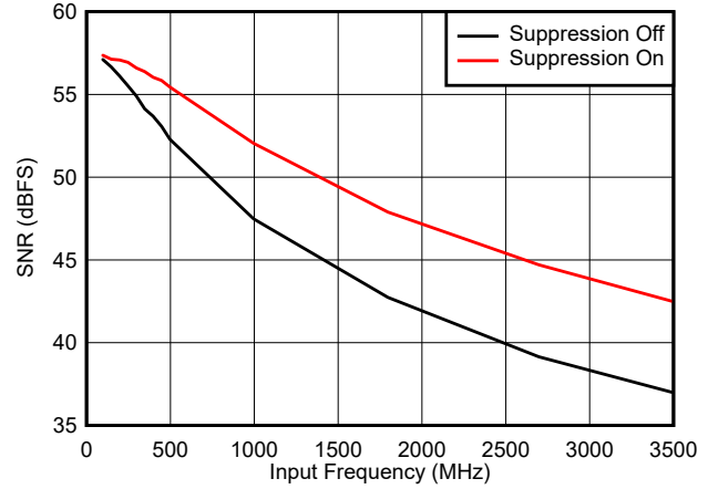
図 5-34. SNR vs Input Frequency and Suppression
