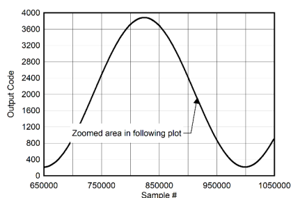
图 5-115. Background Calibration Core Transition (midscale)
