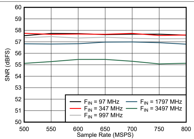
Figure 5-28. SNR vs Sample Rate
