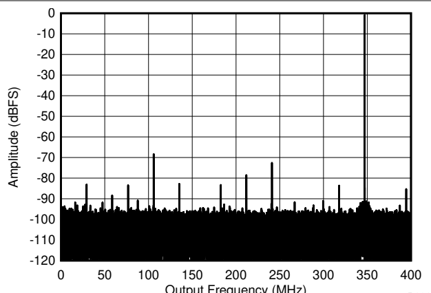
図 5-6. Single Tone FFT at 347 MHz and -1dBFS
