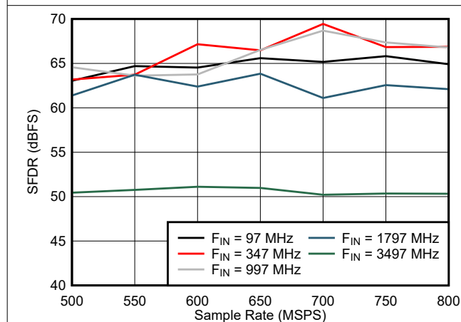
Figure 5-29. SFDR vs Sample Rate
