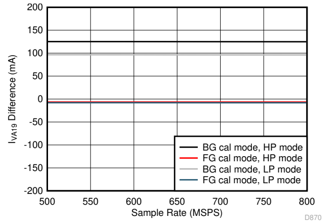
Figure 5-112. Single Channel, I_{VA19} vs F_S over Modes
