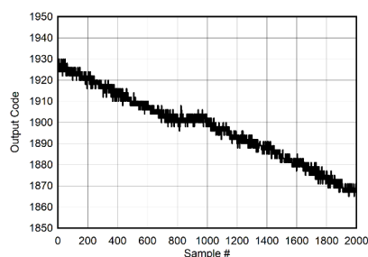
图 5-116. Background Calibration Core Transition (voltage offset)
