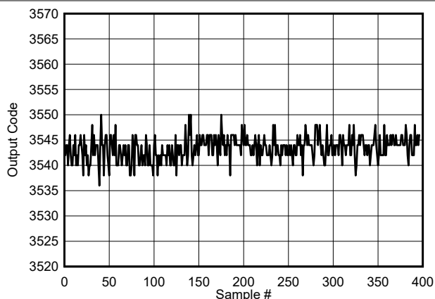
图 5-116. Background Calibration Core Transition (voltage offset)
