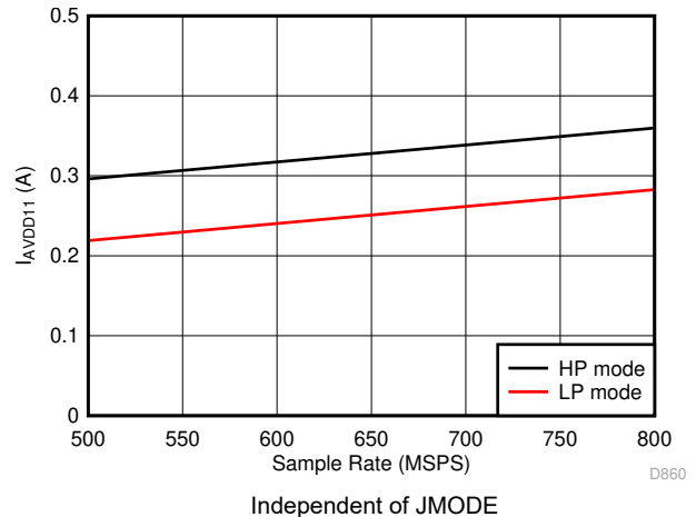
Figure 5-106. Single Channel, I_{VA11} vs F_S
