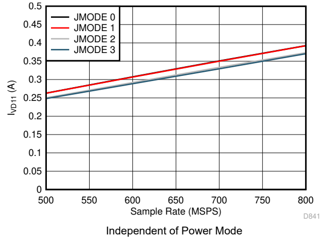
図 5-80. Quad Channel, I_{VD11} vs F_S for JMODES 0 - 3
