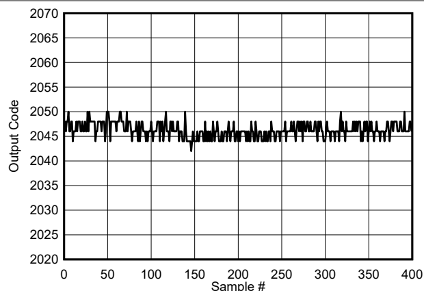
图 5-115. Background Calibration Core Transition (midscale)
