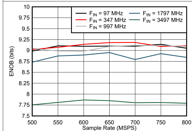
Figure 5-31. ENOB vs Sample Rate
