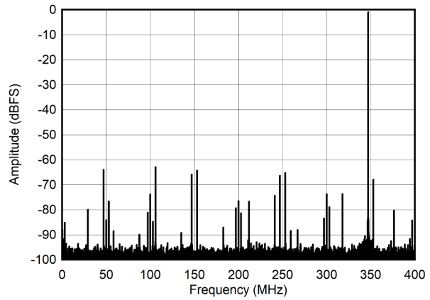
Low Lower Mode, PLL on, suppression off 図 5-18. Single Tone FFT at 347 MHz and -1dBFS
