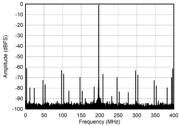
PLL on, suppression on 図 5-17. Single Tone FFT at 997 MHz and -1dBFS
