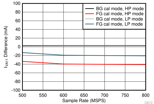
Figure 5-100. Dual Channel, I_{VA11} vs F_S over Modes
