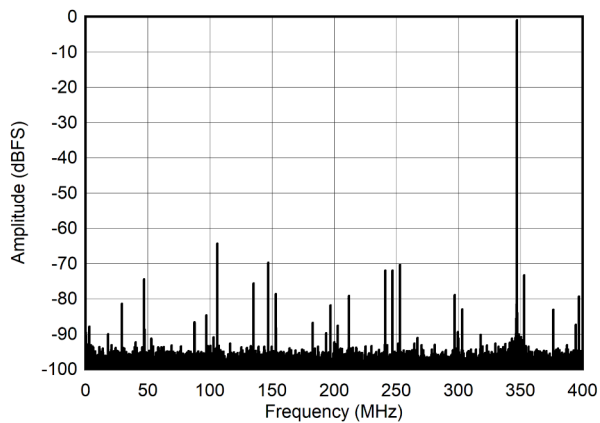
Low Lower Mode, PLL on, suppression on 図 5-19. Single Tone FFT at 347 MHz and -1dBFS
