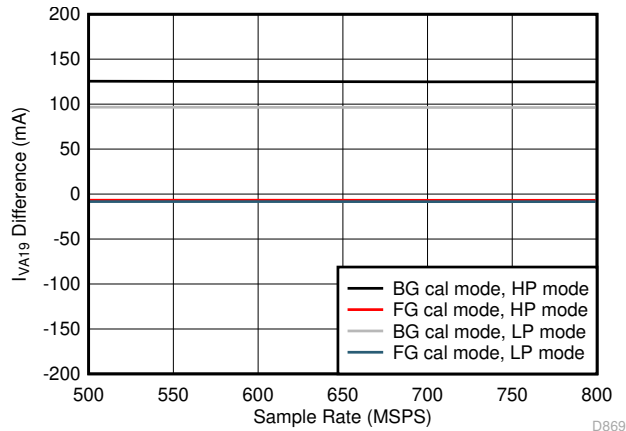
Figure 5-99. Dual Channel, I_{VA19} vs F_S over Modes
