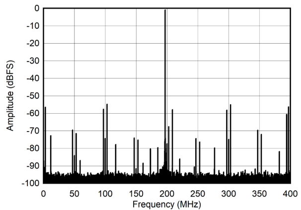
Low Lower Mode, PLL on, suppression off 図 5-20. Single Tone FFT at 997 MHz and -1dBFS
