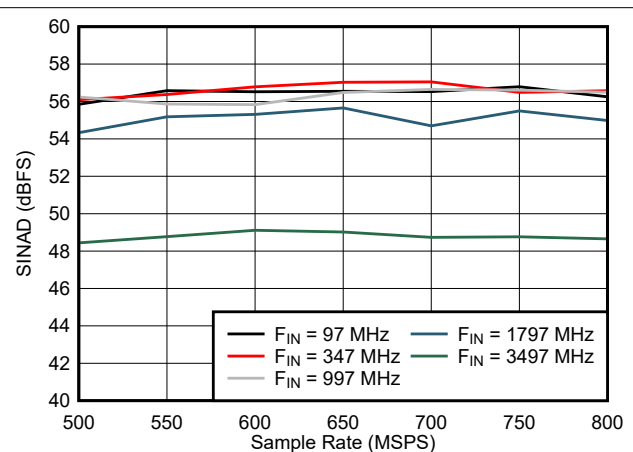
Figure 5-30. SINAD vs Sample Rate
