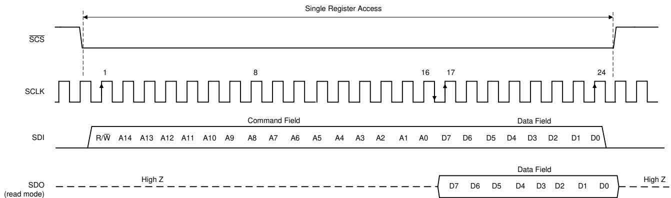
図 6-18. Serial Interface Protocol: Single Read/Write
