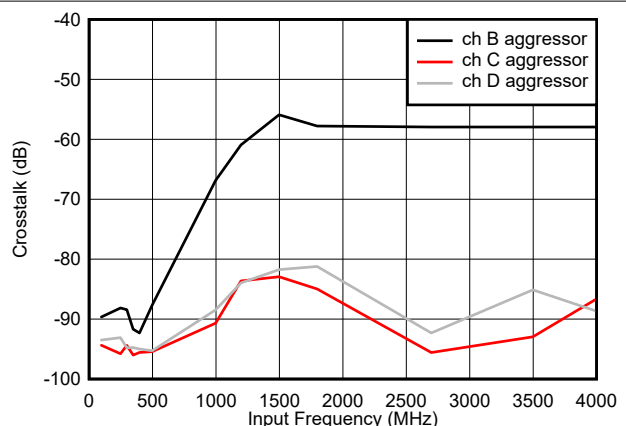
図 5-4. Crosstalk vs Input Frequency, Channel A victim
