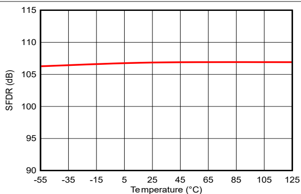
図 5-22. Spurious-Free Dynamic Range vs Temperature
