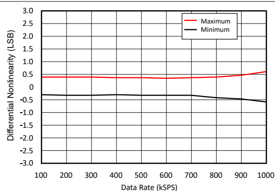
図 5-4. Differential Nonlinearity vs Data Rate
