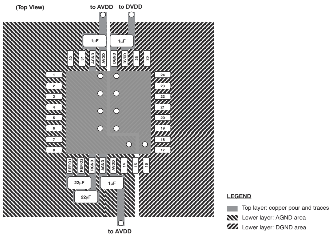
図 8-4. Optimized Layout Recommendation
