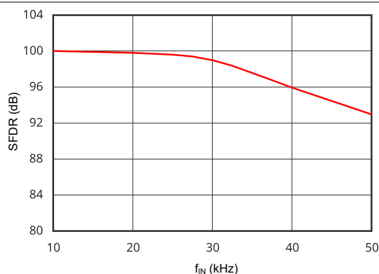
図 5-21. Spurious-Free Dynamic Range vs Input Signal Frequency
