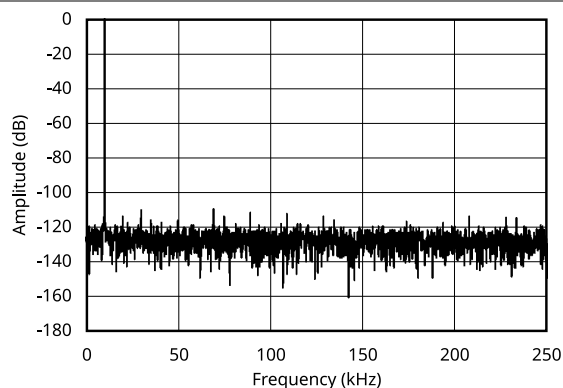
Figure 5-16. Frequency Spectrum (4096 Point FFT; f_{IN} = 10\text{kHz} , f_{SAMPLE} = 0.5\text{MSPS} )
