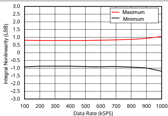
図 5-3. Integral Nonlinearity vs Data Rate
