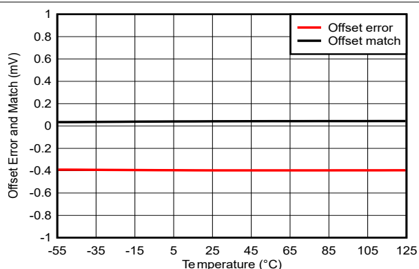
Figure 5-10. Offset Error and Offset Match vs Temperature
