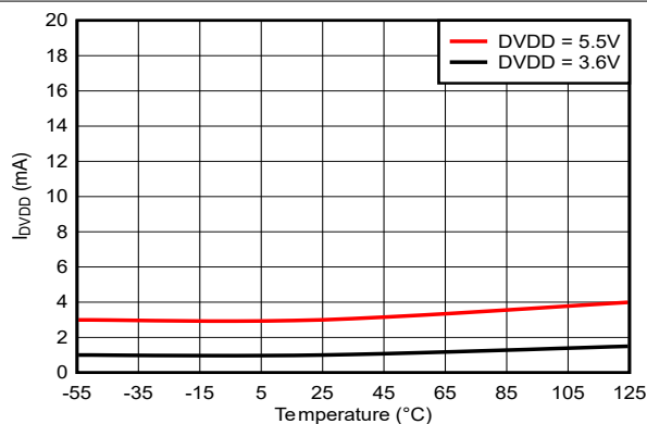
図 5-24. Digital Supply Current vs Temperature
