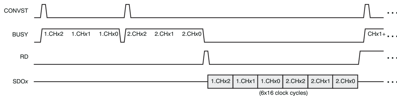
図 7-8. FIFO and Sequencer Operation Example
