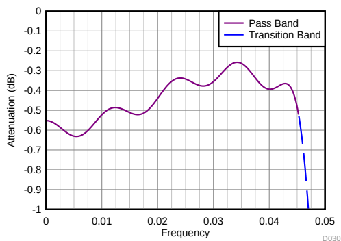
Figure 83. Divide-by-9 Filter Response (Zoomed)
