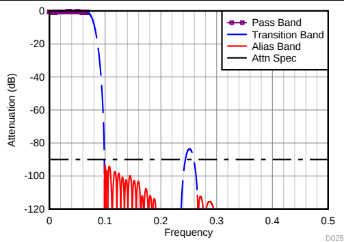
Figure 78. Divide-by-6 Filter Response
