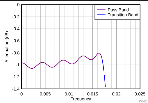
Figure 95. Divide-by-24 Filter Response (Zoomed)
