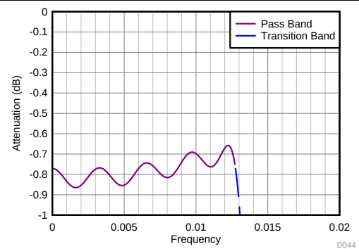
Figure 97. Divide-by-32 Filter Response (Zoomed)
