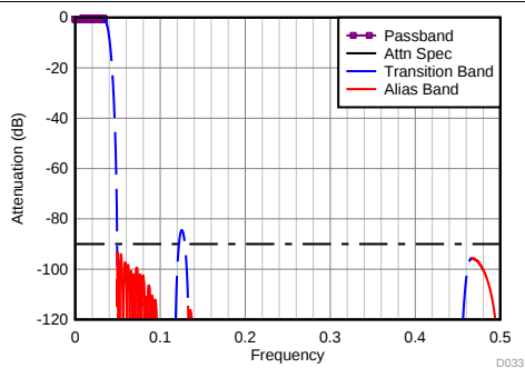
Figure 86. Divide-by-12 Filter Response
