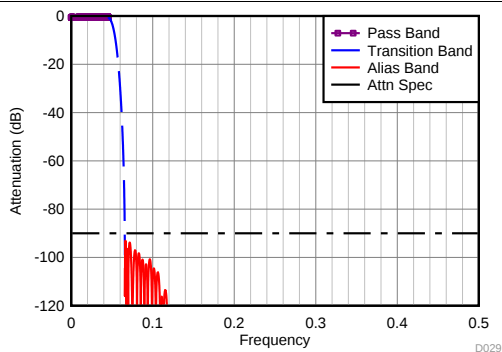
Figure 82. Divide-by-9 Filter Response
