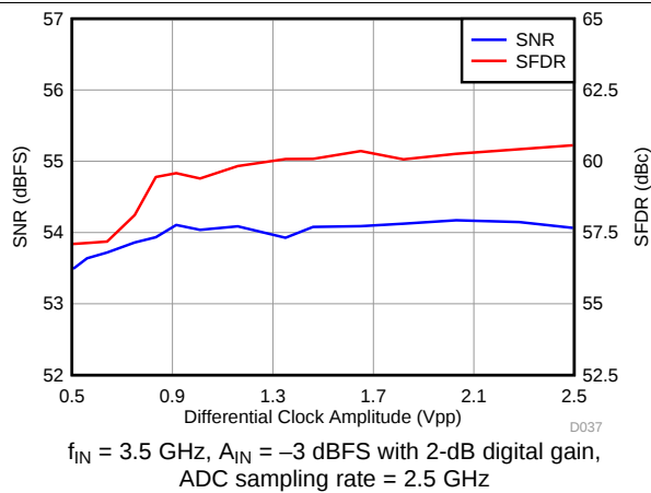
Figure 39. Performance vs Clock Amplitude
