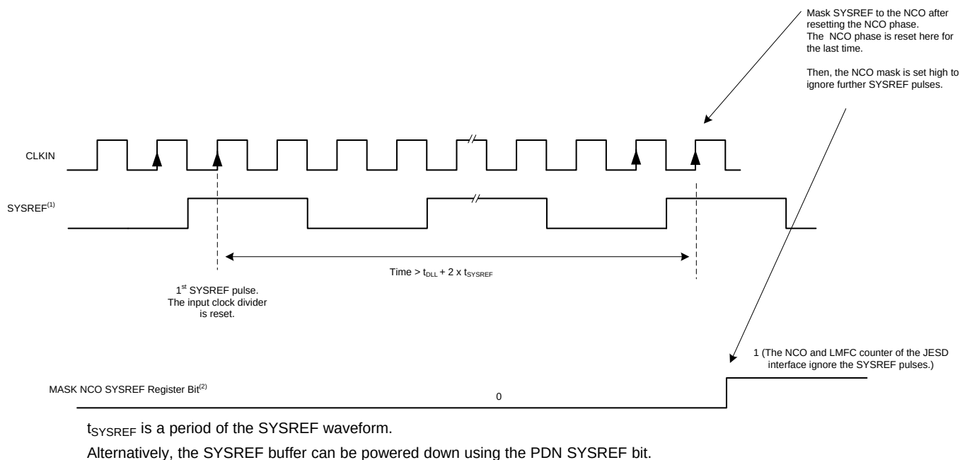
Figure 70. SYSREF Used as a Periodic Waveform
