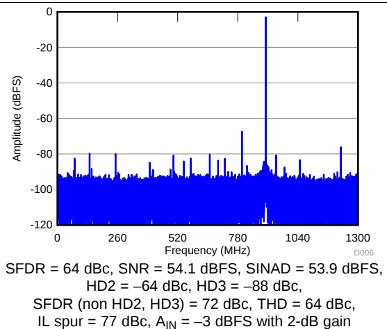
Figure 8. FFT for 3500-MHz Input Signal
