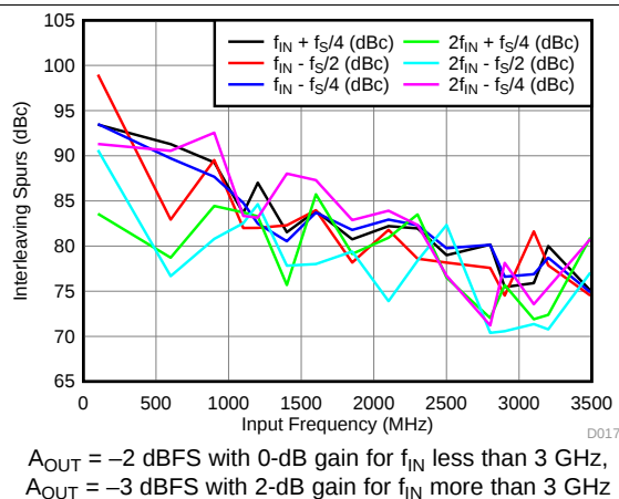
Figure 19. IL Spur vs Input Frequency
