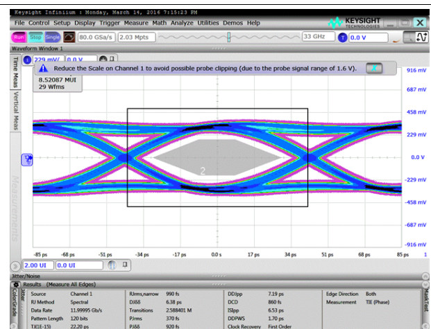
Figure 102. Data Eye at 12 Gbps
