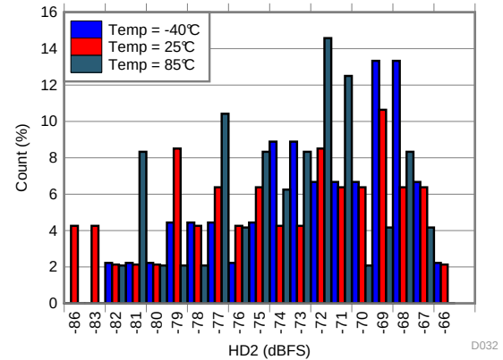
Figure 34. HD2 Histogram at AVDD19 = 1.9 V
