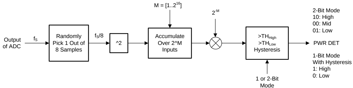
Figure 107. RMS Power Detector Implementation
