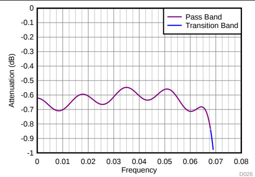
Figure 79. Divide-by-6 Filter Response (Zoomed)
