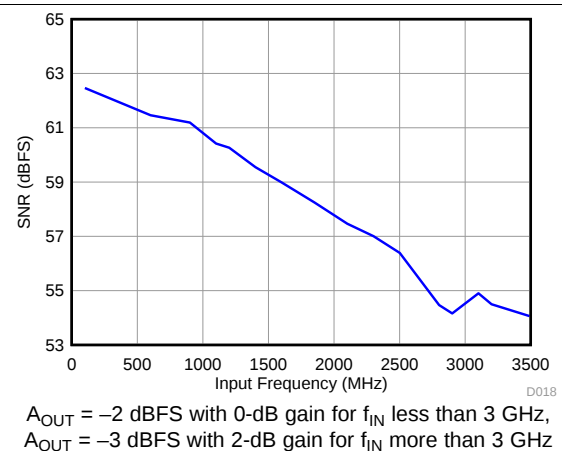
Figure 20. Signal-to-Noise Ratio vs Input Frequency
