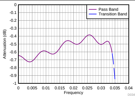
Figure 87. Divide-by-12 Filter Response (Zoomed)
