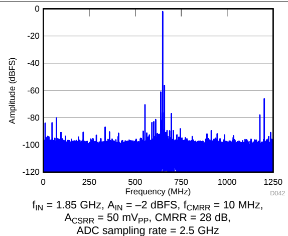
Figure 44. Common-Mode Rejection Ratio FFT
