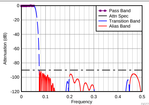
Figure 80. Divide-by-8 Filter Response
