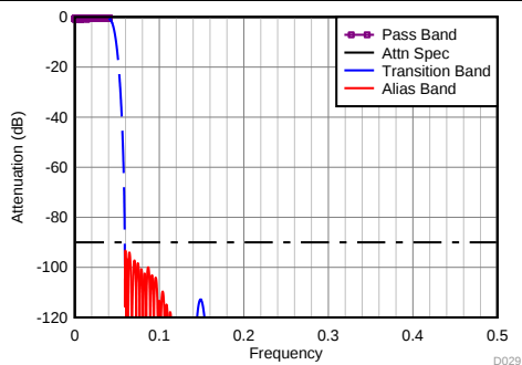
Figure 84. Divide-by-10 Filter Response
