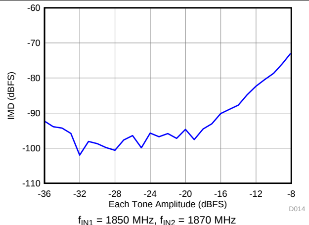
Figure 16. Intermodulation Distortion vs Input Amplitude (1850 MHz and 1870 MHz)
