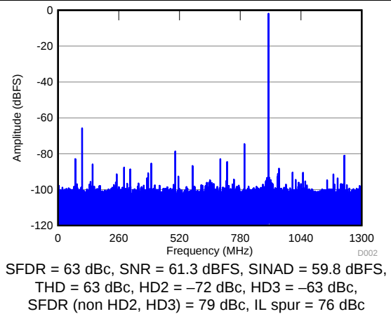
Figure 4. FFT for 900-MHz Input Signal
