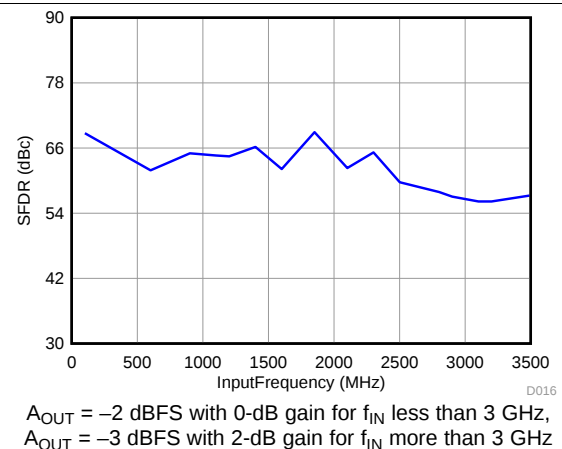
Figure 18. Spurious-Free Dynamic Range vs Input Frequency
