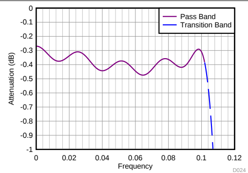
Figure 77. Divide-by-4 Filter Response (Zoomed)
