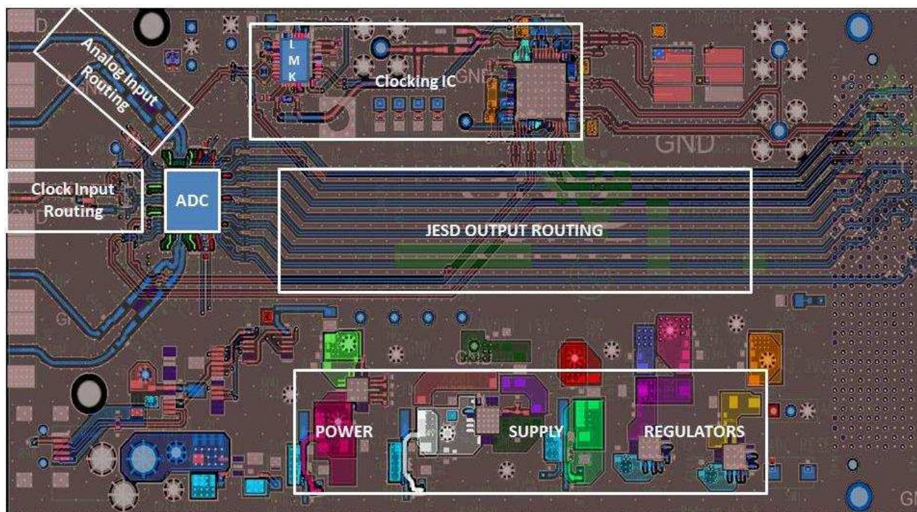
Figure 244. ADC32RF42EVM Layout
