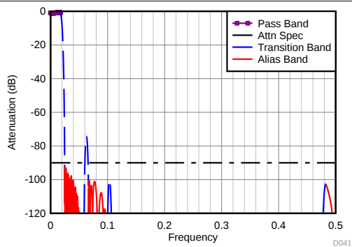
Figure 94. Divide-by-24 Filter Response
