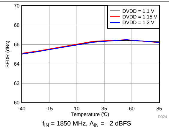
Figure 26. Spurious-Free Dynamic Range vs DVDD Supply and Temperature
