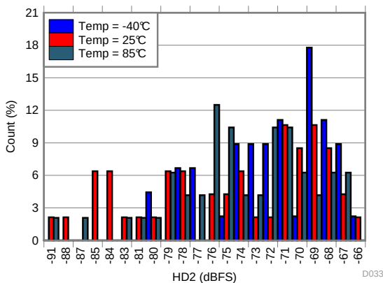
Figure 33. HD2 Histogram at AVDD19 = 1.8 V
