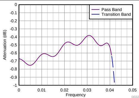
Figure 85. Divide-by-10 Filter Response (Zoomed)
