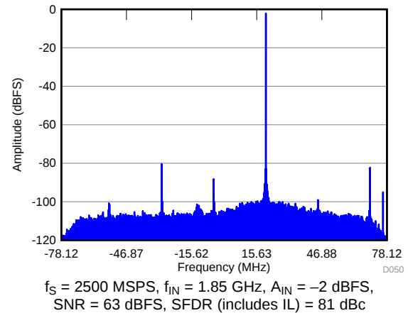
Figure 52. FFT in 16X Decimation
