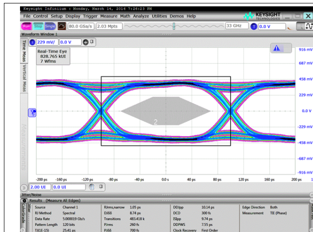
Figure 101. Data Eye at 5 Gbps
