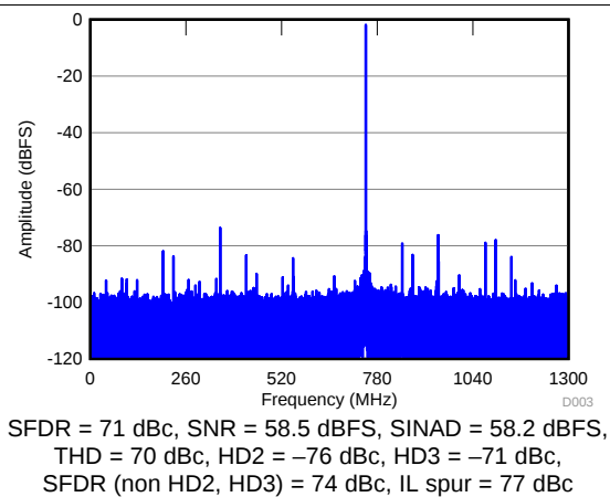
Figure 5. FFT for 1850-MHz Input Signal
