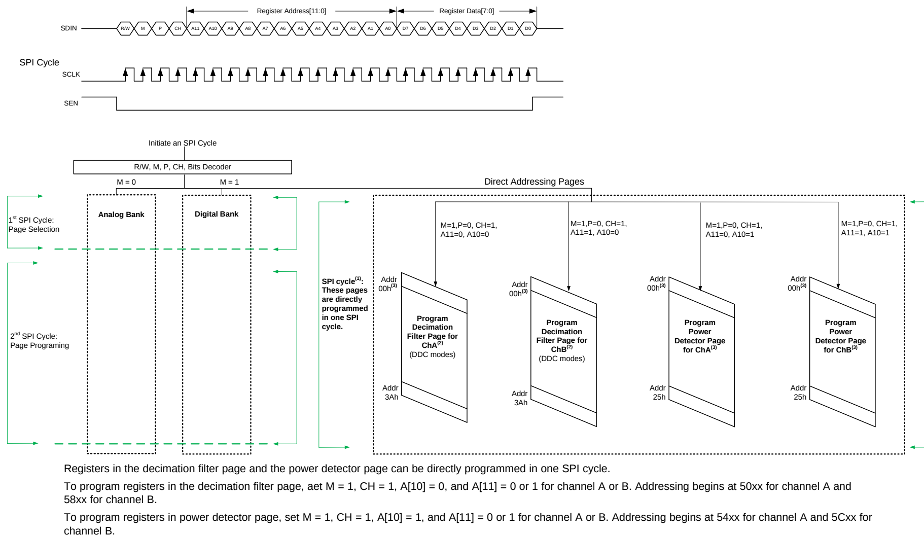
Figure 122. SPI Registers: Direct Addressing
