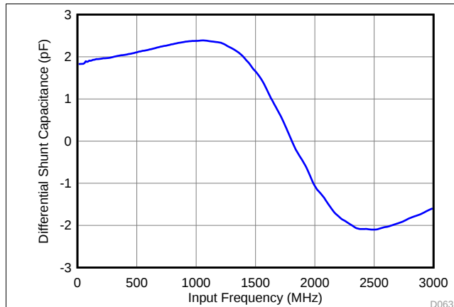
Figure 60. Differential Input Capacitance vs Input Frequency
