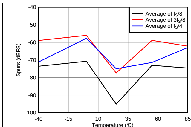
Figure 237. Offset Corrector Block Frozen at Room Temperature
