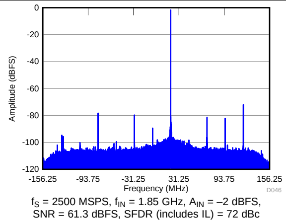
Figure 48. FFT in 8X Decimation
