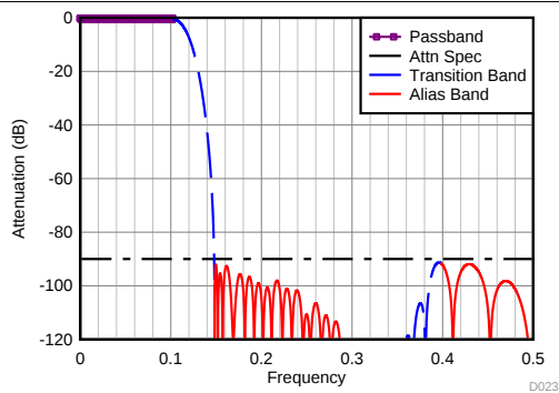
Figure 76. Divide-by-4 Filter Response
