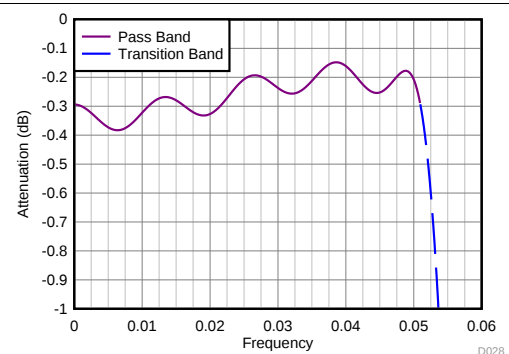
Figure 81. Divide-by-8 Filter Response (Zoomed)
