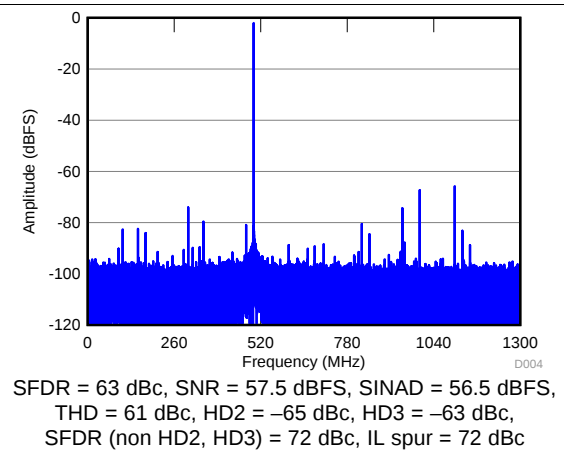
Figure 6. FFT for 2100-MHz Input Signal
