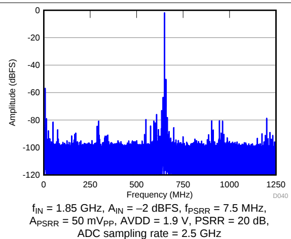
Figure 42. Power-Supply Rejection Ratio FFT for Test Signal on AVDD Supply
