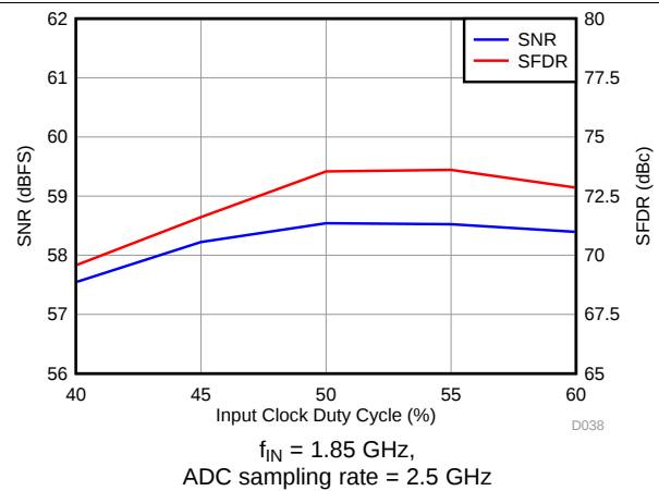
Figure 40. Performance vs Clock Duty Cycle
