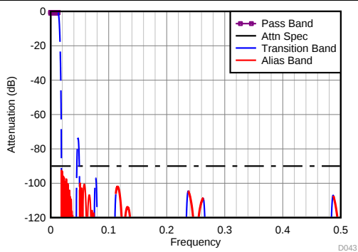
Figure 96. Divide-by-32 Filter Response
