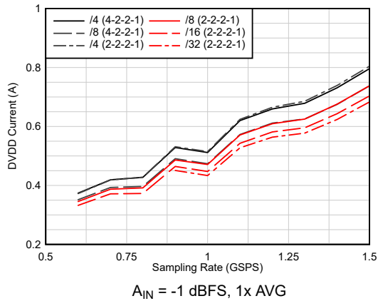
6-49. Current vs Sampling Rate vs Real Decimation
