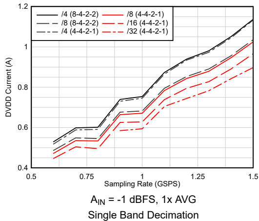
6-51. Current vs Sampling Rate vs Complex Decimation
