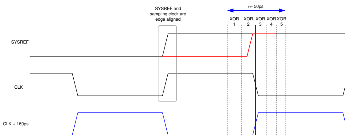
7-14. Detection of SYSREF Transition within Capture Window
