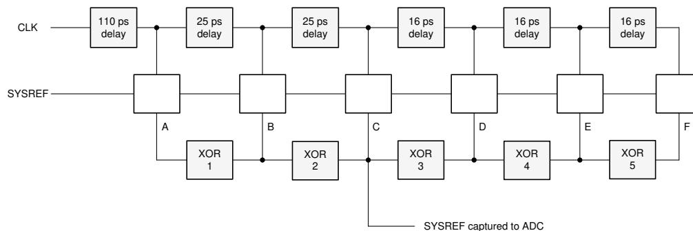
7-13. SYSREF Detection Circuitry
