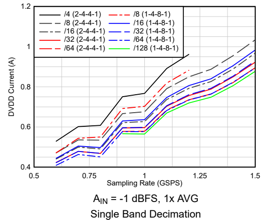
6-52. Current vs Sampling Rate vs Complex Decimation
