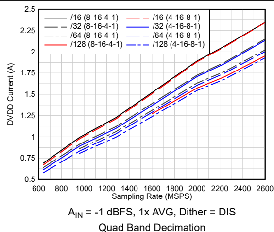
FIG 6-54. Current vs Sampling Rate vs Decimation
