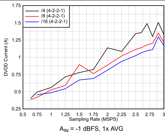
6-102. Current vs Sampling Rate vs Real Decimation
