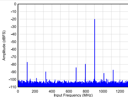
FIG 6-19. Single Tone FFT at F_{IN} = 900\text{ MHz}
