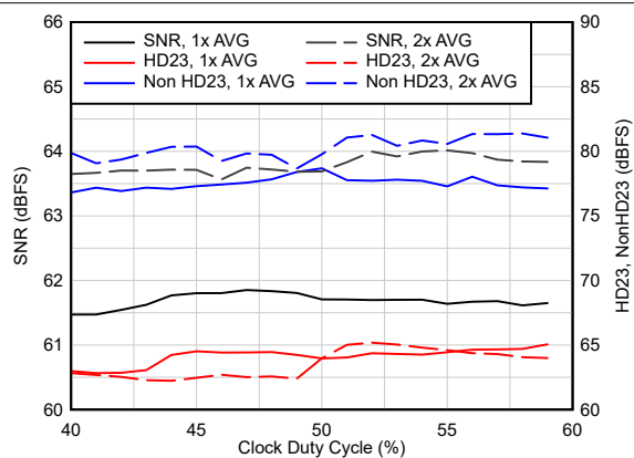
FIG 6-95. AC Performance vs Clock Duty Cycle
