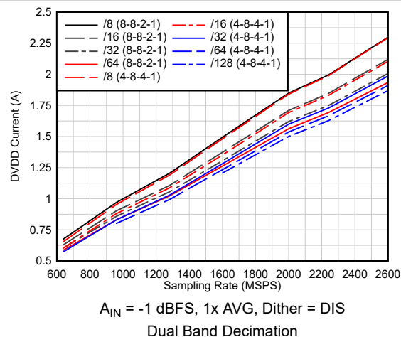
FIG 6-52. Current vs Sampling Rate vs Decimation
