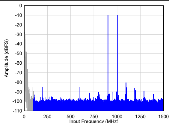
IMD3 = 70 dBc A_{IN} = -10 dBFS/tone, 1x AVG, Dither = EN FIG 6-79. Two Tone FFT at F_{IN} = 900/1000 MHz
