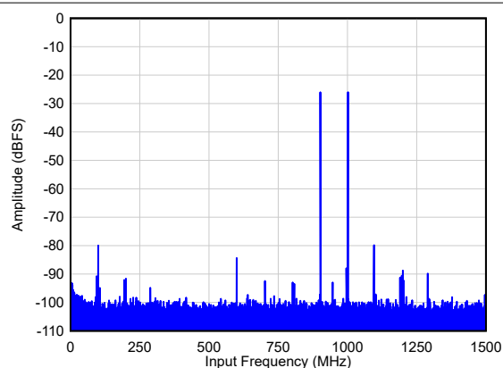
IMD3 = 54 dBc A_{IN} = -26 dBFS/tone, 1x AVG, Dither = DIS FIG 6-80. Two Tone FFT at F_{IN} = 900/1000 MHz
