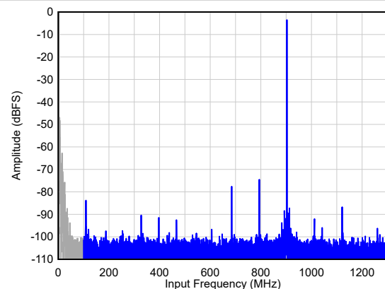
FIG 6-14. Single Tone FFT at F_{IN} = 900 MHz
