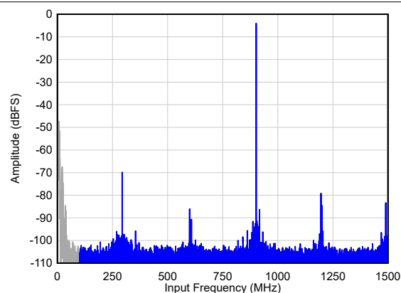
FIG 6-69. Single Tone FFT at F_{IN} = 900 MHz
