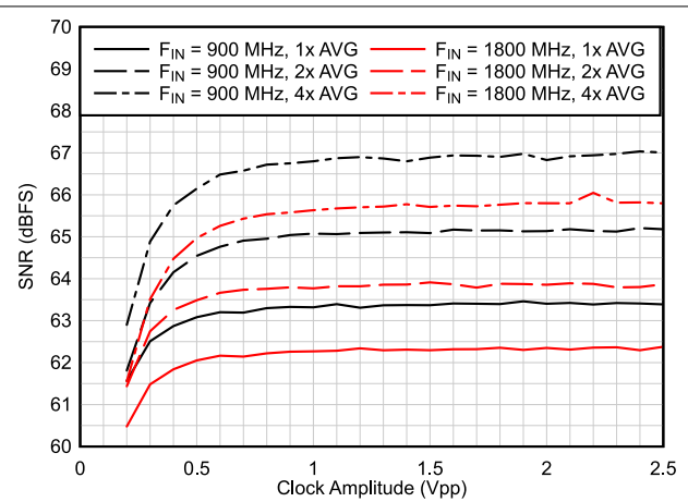
8-3. SNR vs Clock Amplitude (dither off)
