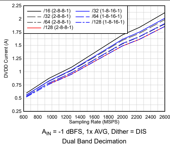
FIG 6-53. Current vs Sampling Rate vs Decimation
