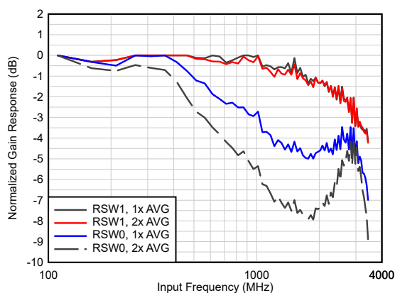
Figure 7-2. Input Bandwidth - Reset switch DIS
