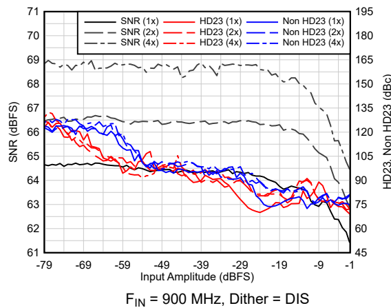
Figure 6-86. AC Performance vs A_{IN}
