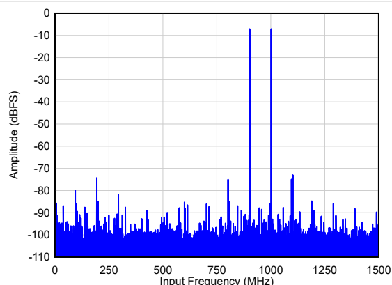
IMD3 = 68 dBc A_{IN} = -7 dBFS/tone, 1x AVG, Dither = DIS FIG 6-78. Two Tone FFT at F_{IN} = 900/1000 MHz
