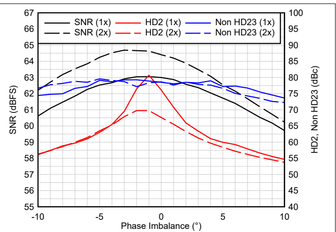
7-4. Phase Imbalance - 2.6 GSPS
