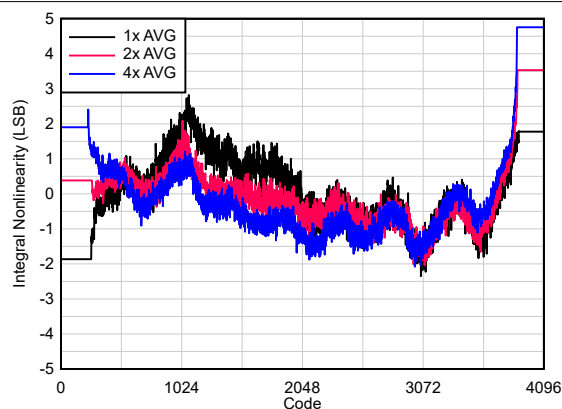
6-97. INL vs Code
