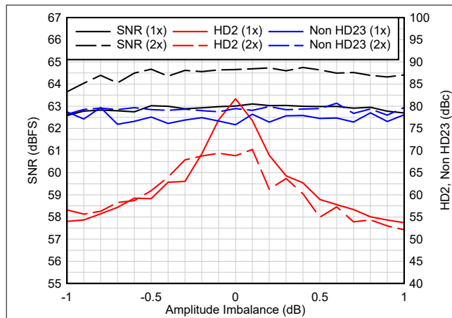
7-3. Amplitude Imbalance - 2.6 GSPS
