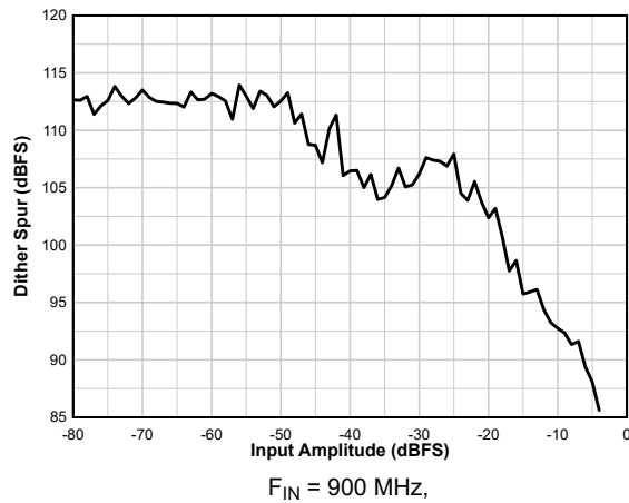
Figure 6-84. Dither Spur vs A_{IN}
