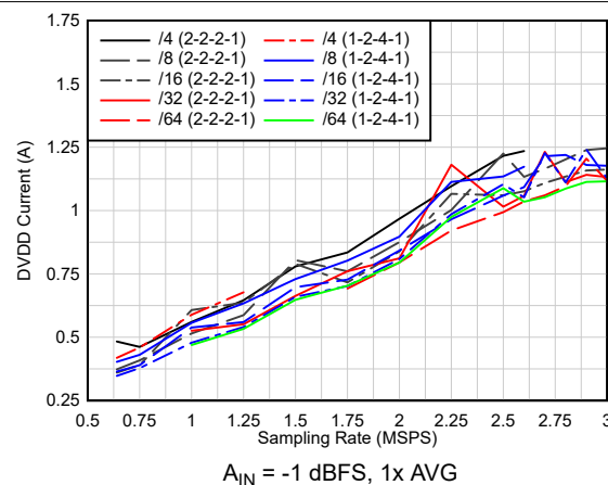
6-103. Current vs Sampling Rate vs Real Decimation
