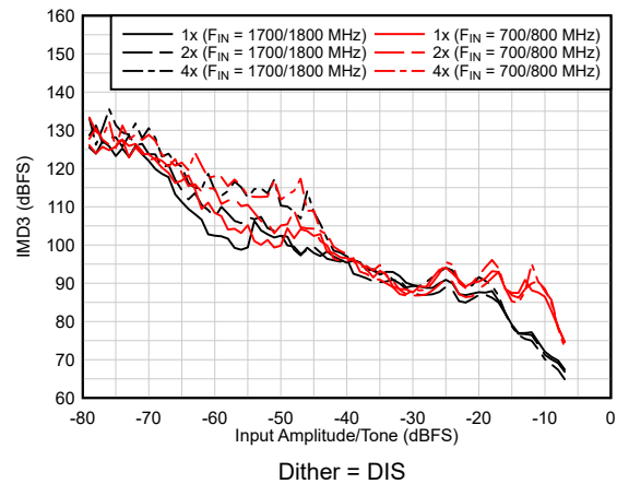
Figure 6-88. IMD3 Performance vs A_{IN}
