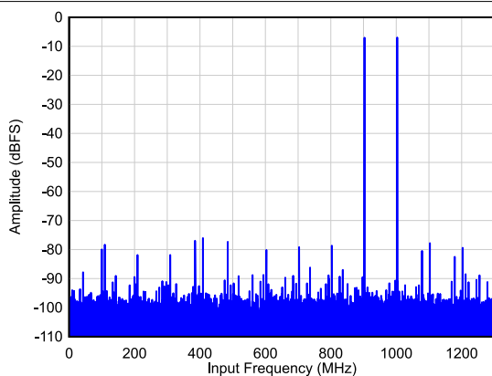
FIG 6-23. Two Tone FFT at F_{IN} = 900/1000 MHz
