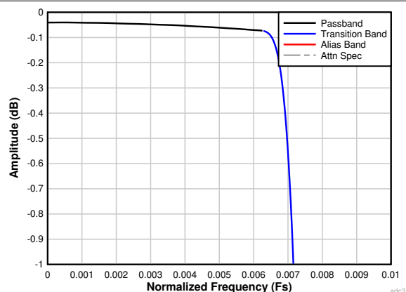
7-34. Decimation by 64 Passband Ripple Response
