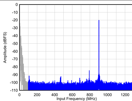
FIG 6-18. Single Tone FFT at F_{IN} = 900\text{ MHz}
