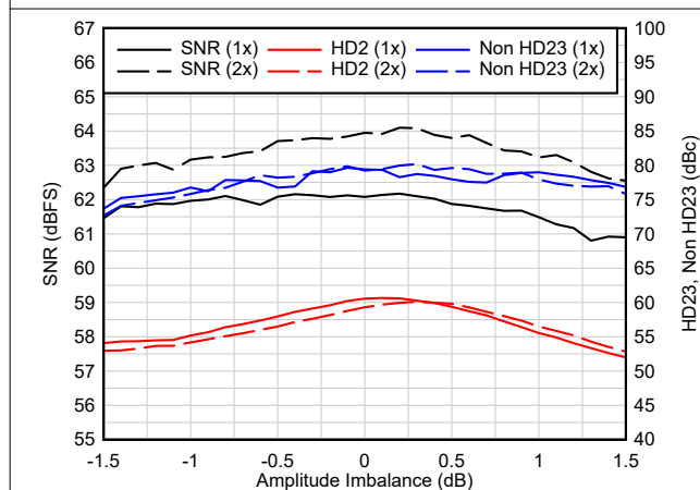
7-5. Amplitude Imbalance - 3.0 GSPS
