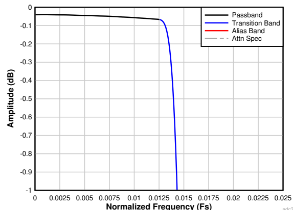
7-31. Decimation by 32 Passband Ripple Response
