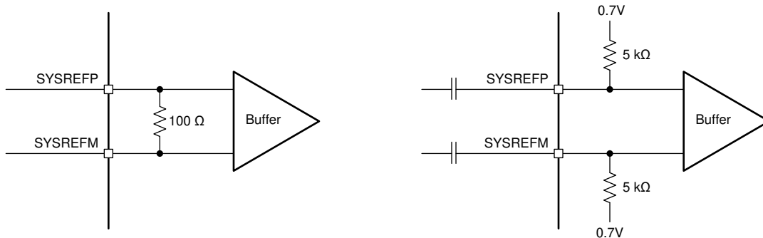
図 7-15. SYSREF Input Circuitry and Edge Alignment
