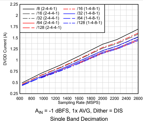
FIG 6-51. Current vs Sampling Rate vs Decimation
