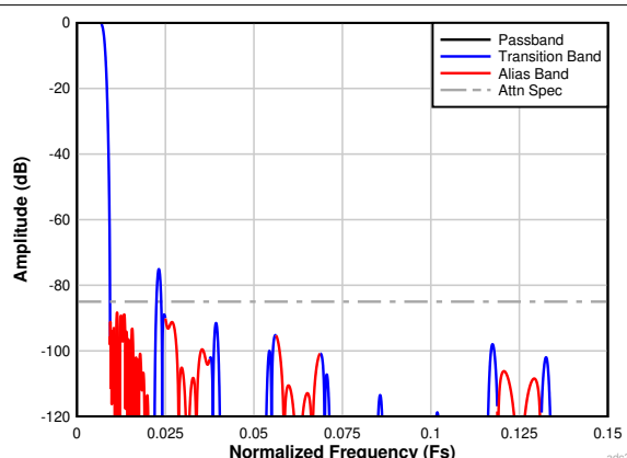
7-33. Complex Decimation by 64 Filter Response
