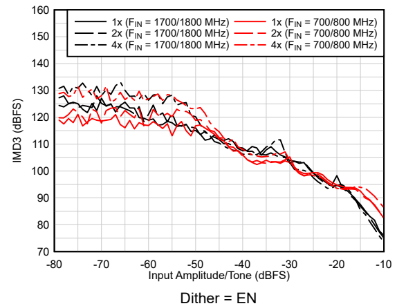
Figure 6-89. IMD3 Performance vs A_{IN}
