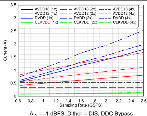
FIG 6-47. Current vs Sampling Rate vs Averaging
