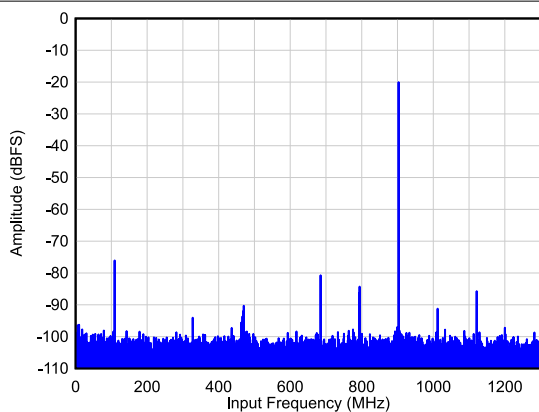
FIG 6-17. Single Tone FFT at F_{IN} = 900\text{ MHz}
