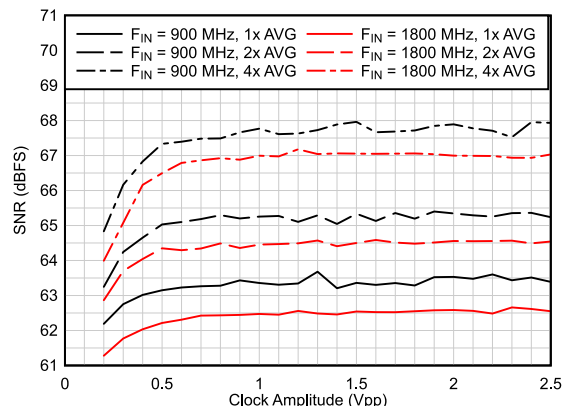
7-13. SNR vs Clock Amplitude (Dither ON)
