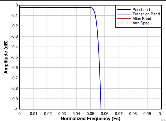
7-27. Decimation by 8 Passband Ripple Response
