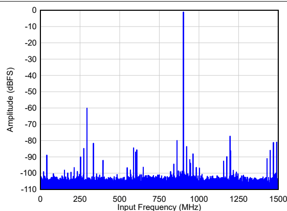
FIG 6-68. Single Tone FFT at F_{IN} = 900 MHz
