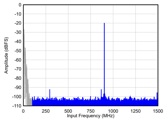
FIG 6-73. Single Tone FFT at F_{IN} = 900 MHz
