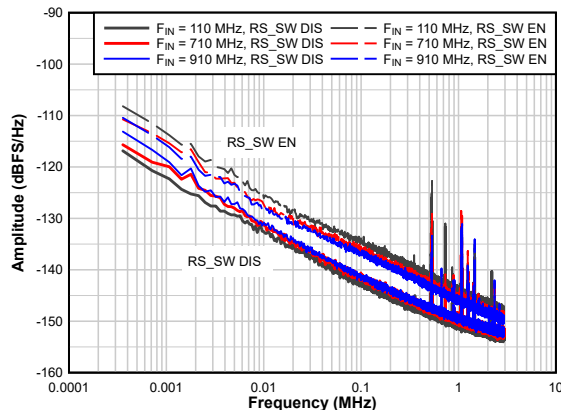
7-10. Amplitude Noise vs Input Frequency
