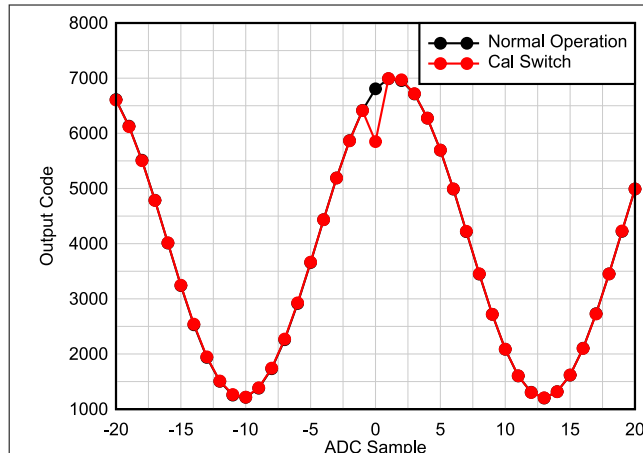
Figure 7-21. Output Code vs ADC Sample
