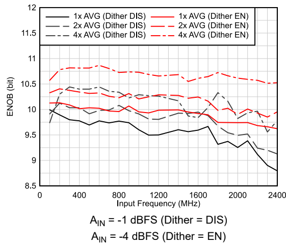
Figure 6-29. ENOB Performance vs F_{IN}
