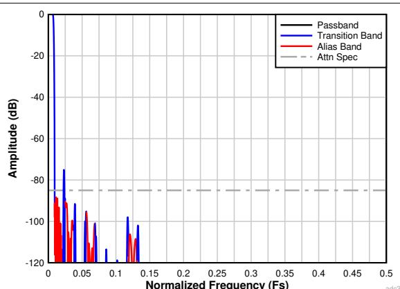
7-32. Complex Decimation by 64 Filter Response
