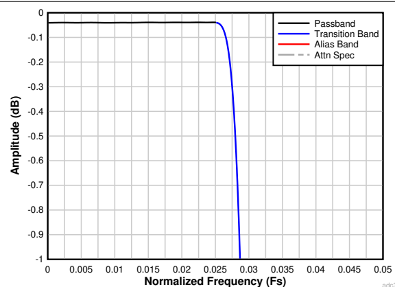
7-29. Decimation by 16 Passband Ripple Response
