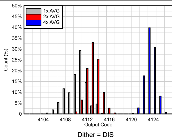
Figure 6-45. DC Offset Histogram
