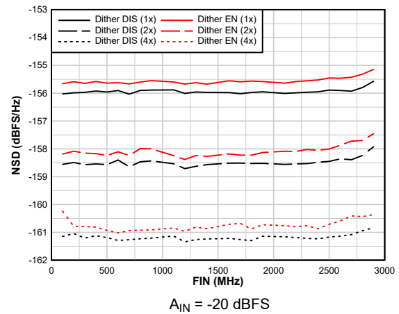
Figure 6-85. NSD Performance vs F_{IN}
