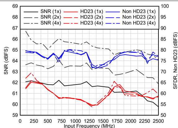
A_{IN} = -1 dBFS, Dither = DIS FIG 6-82. AC Performance vs F_{IN}
