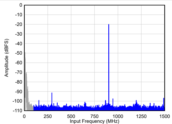
FIG 6-75. Single Tone FFT at F_{IN} = 900 MHz
