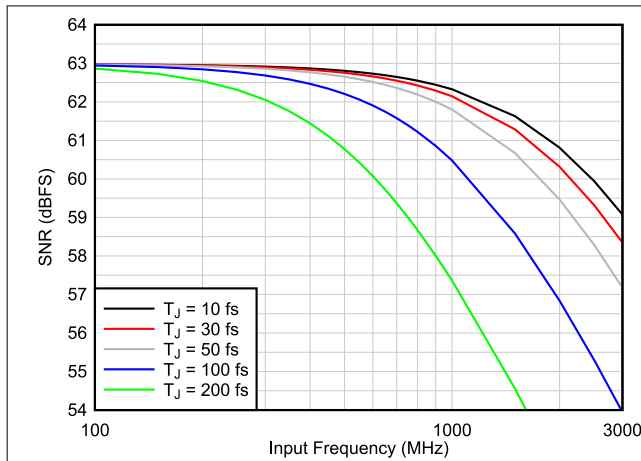
8-2. SNR vs T_{Jitter} vs F_{IN} (1x AVG)
