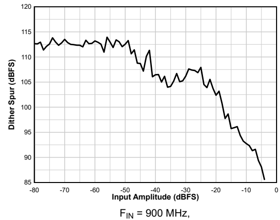
Figure 6-30. Dither Spur vs A_{IN}
