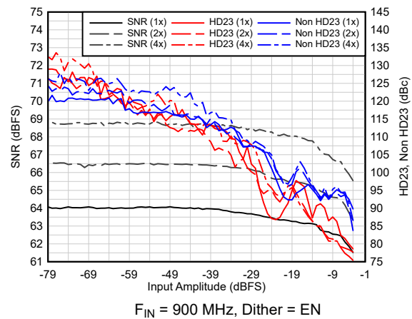
Figure 6-87. AC Performance vs A_{IN}
