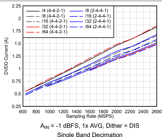
FIG 6-50. Current vs Sampling Rate vs Decimation
