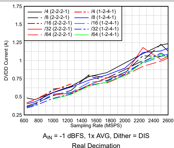
FIG 6-49. Current vs Sampling Rate vs Decimation
