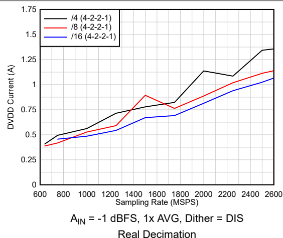
FIG 6-48. Current vs Sampling Rate vs Decimation
