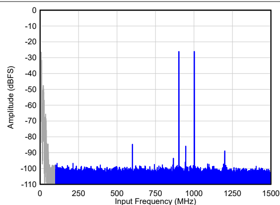
IMD3 = 71 dBc A_{IN} = -26 dBFS/tone, 1x AVG, Dither = EN FIG 6-81. Two Tone FFT at F_{IN} = 900/1000 MHz
