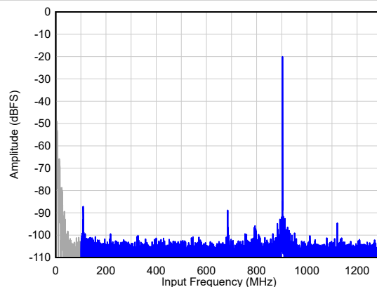
FIG 6-20. Single Tone FFT at F_{IN} = 900\text{ MHz}
