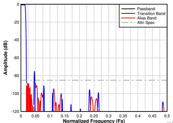
7-30. Complex Decimation by 32 Filter Response
