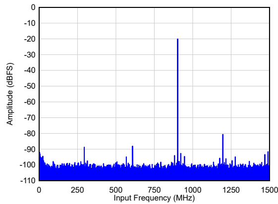
FIG 6-72. Single Tone FFT at F_{IN} = 900 MHz
