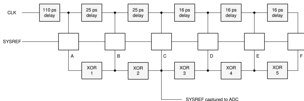
7-16. SYSREF Detection Circuitry
