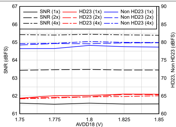
FIG 6-91. AC Performance vs AVDD18
