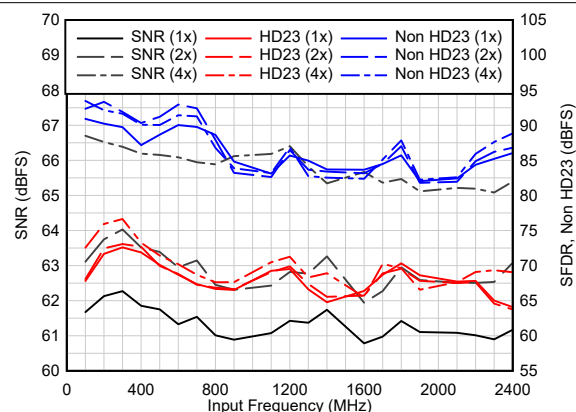
A_{IN} = -4 dBFS, Dither = EN FIG 6-83. AC Performance vs F_{IN}
