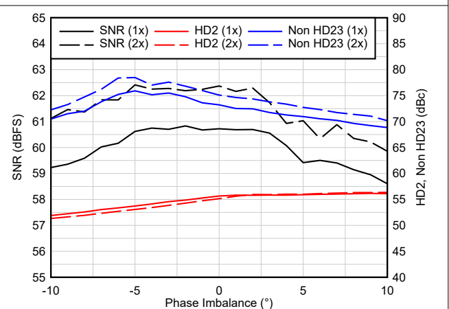
7-6. Phase Imbalance - 3.0 GSPS
