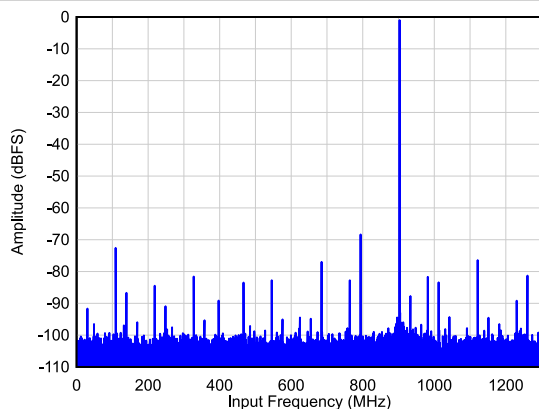
FIG 6-13. Single Tone FFT at F_{IN} = 900 MHz
