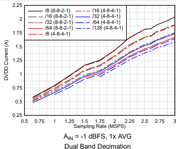
6-106. Current vs Sampling Rate vs Complex Decimation
