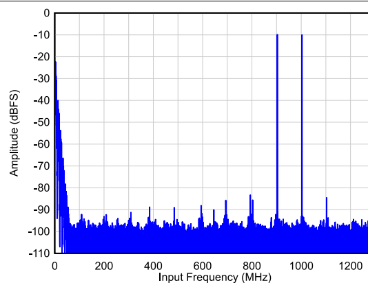
FIG 6-24. Two Tone FFT at F_{IN} = 900/1000 MHz
