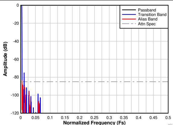
7-35. Complex Decimation by 128 Filter Response
