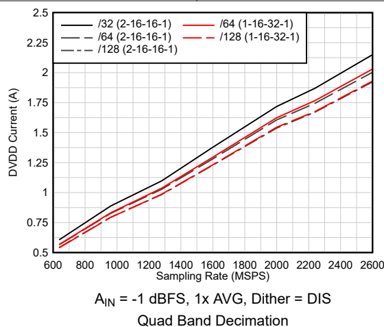
FIG 6-55. Current vs Sampling Rate vs Decimation
