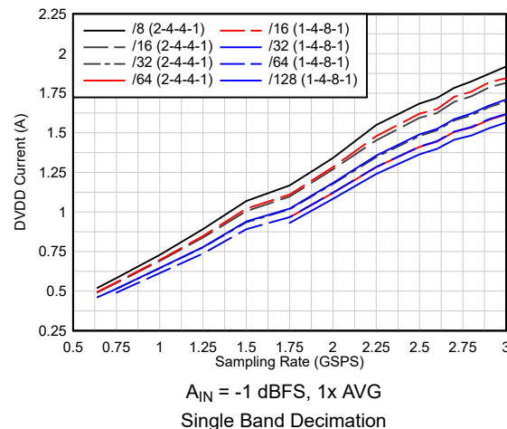
6-105. Current vs Sampling Rate vs Complex Decimation
