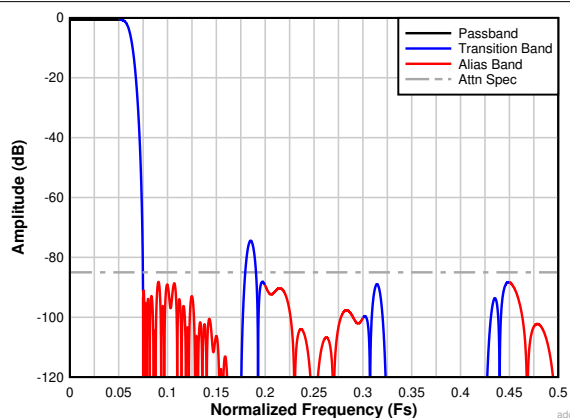
7-26. Complex Decimation by 8 Filter Response
