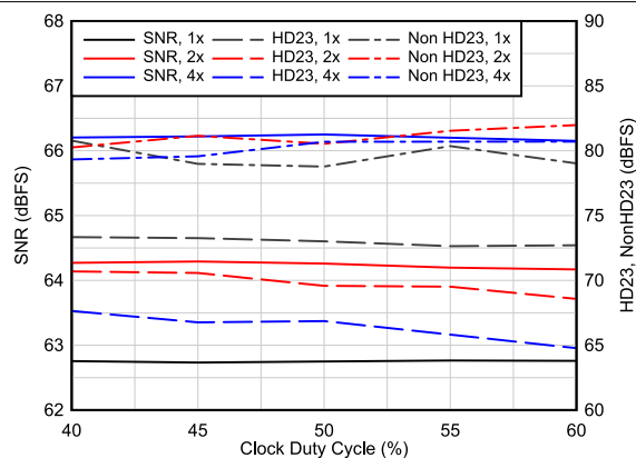
F_{IN} = 900 \text{ MHz} , A_{IN} = -1 \text{ dBFS} , Dither = DIS Figure 6-41. AC Performance vs Clock Duty Cycle
