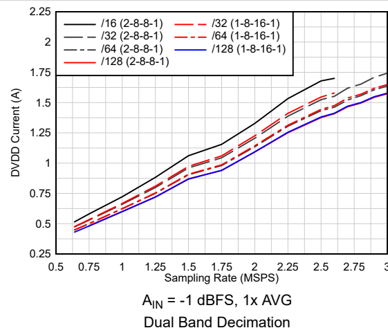
6-107. Current vs Sampling Rate vs Complex Decimation
