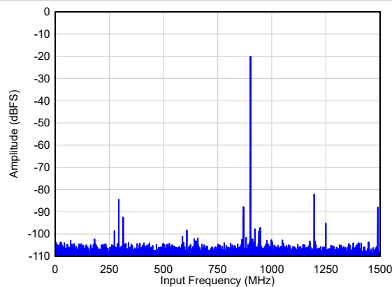
FIG 6-74. Single Tone FFT at F_{IN} = 900 MHz
