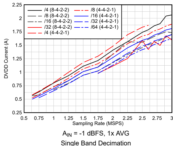
6-104. Current vs Sampling Rate vs Complex Decimation
