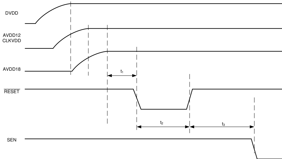
図 8-4. Initialization of Serial Registers After Power-Up
