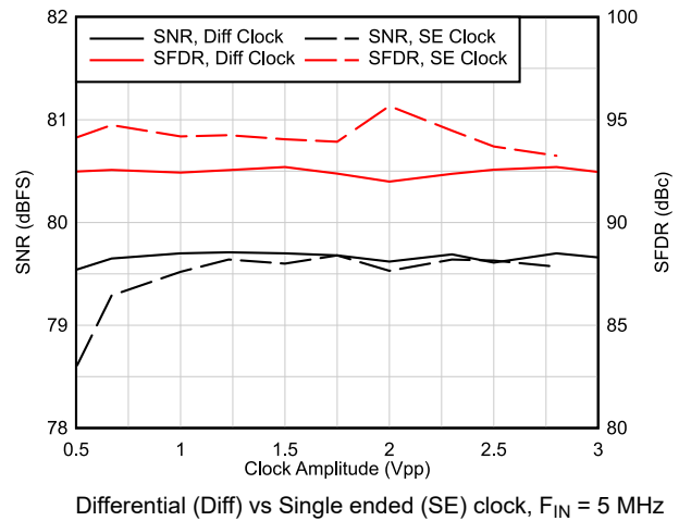
6-52. AC Performance vs Clock Amplitude
