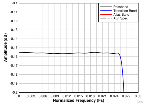
8-32. Decimation by 16 complex passband ripple response
