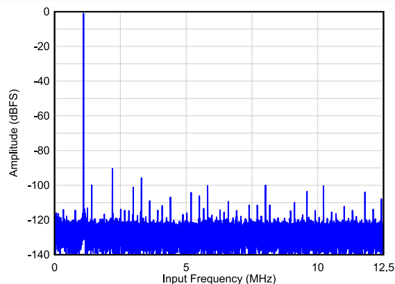
FIG 6-18. Single Tone FFT at F_{IN} = 1.1\text{ MHz}
