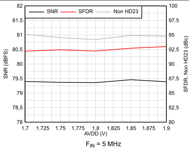
6-53. AC Performance vs AVDD
