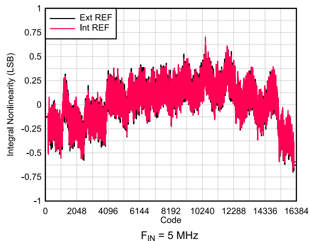
FIG 6-55. INL vs Code
