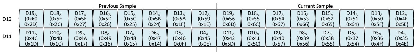
8-46. Example: 2-wire output mapping
