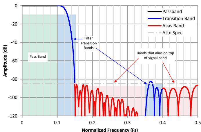
図 8-24. Interpretation of the Decimation Filter Plots
