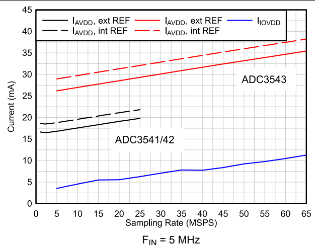
FIG 6-60. Current vs Sampling Rate
