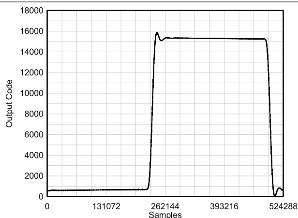
Figure 6-14. Pulse Response
