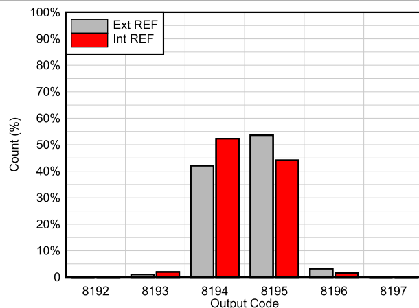
FIG 6-57. DC Histogram
