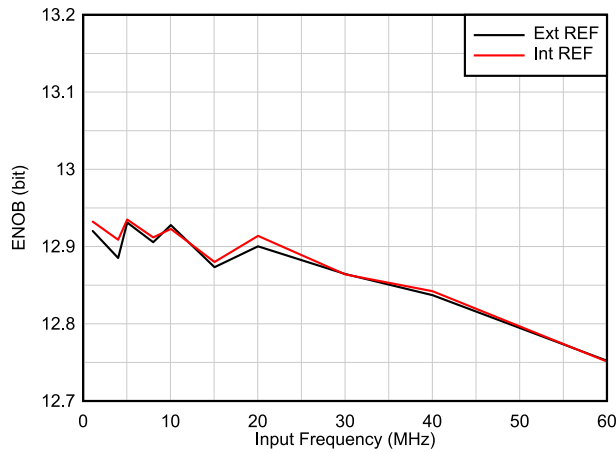
6-49. ENOB vs Input Frequency
