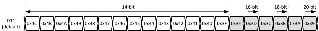
8-47. 1-wire output bit mapping
