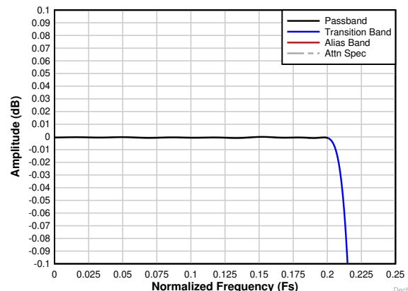
8-26. Decimation by 2 complex passband ripple response
