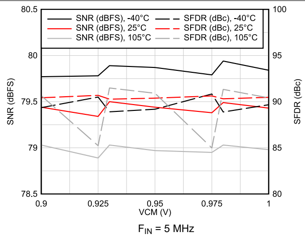
6-54. AC Performance vs VCM vs Temperature
