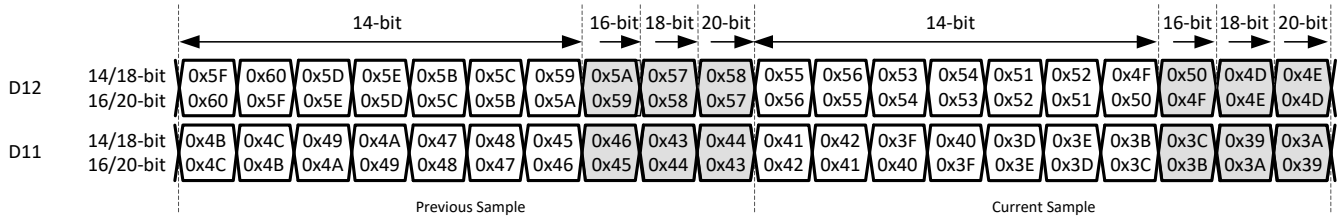
8-45. 2-wire output bit mapper
