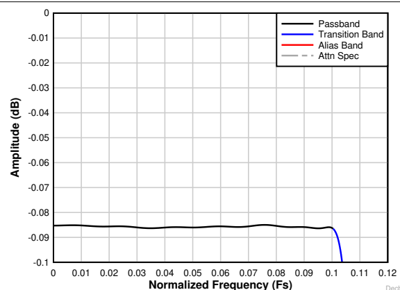
8-28. Decimation by 4 complex passband ripple response
