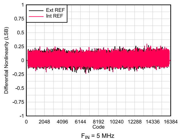
FIG 6-56. DNL vs Code
