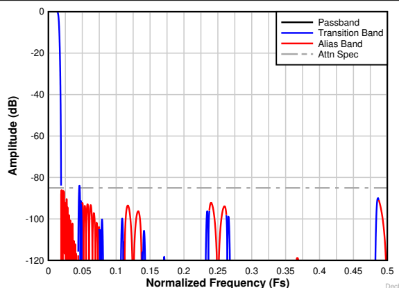
8-33. Decimation by 32 complex frequency response
