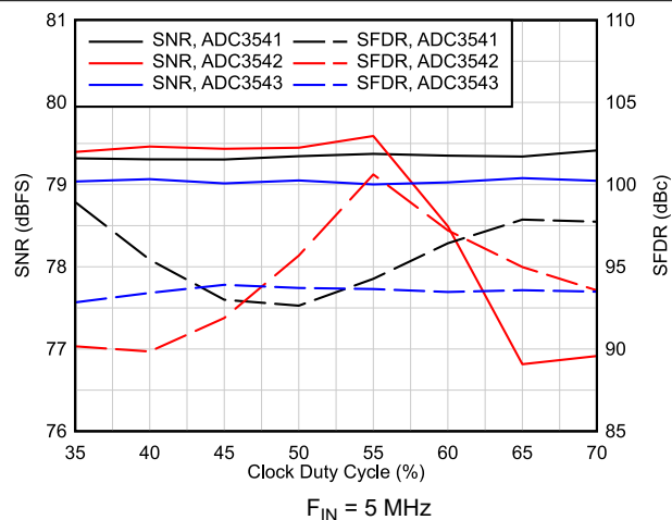
FIG 6-59. AC Performance vs Clock Duty Cycle
