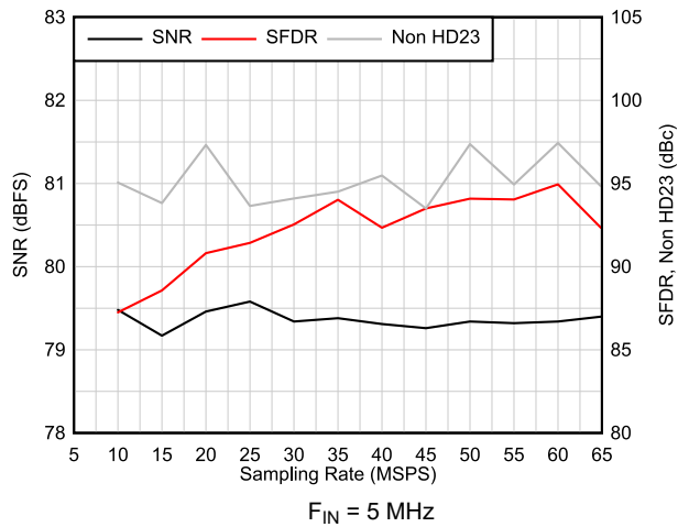
6-51. AC Performance vs Sampling Rate
