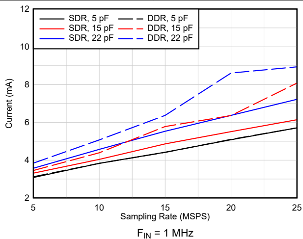
Figure 6-17. I OVDD Current vs Output Load
