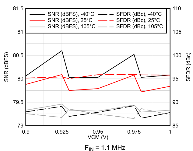
6-31. AC Performance vs VCM vs Temperature
