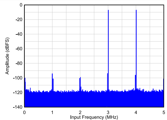
FIG 6-2. Two Tone FFT at F_{IN} = 3,4\text{ MHz}
