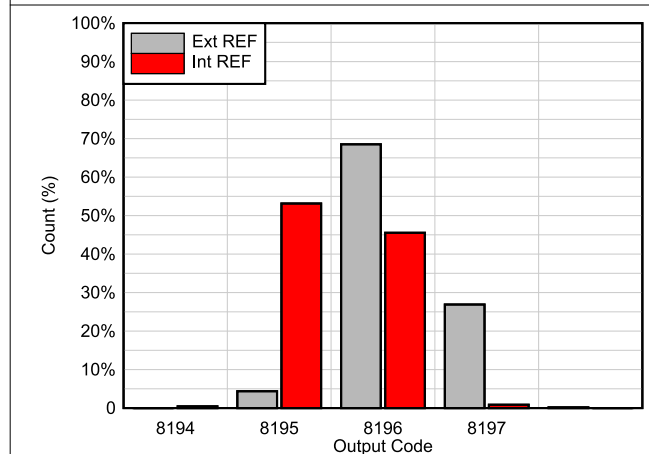
6-34. DC Histogram
