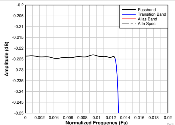
8-34. Decimation by 32 complex passband ripple response
