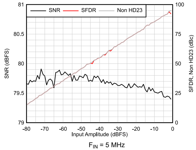
6-50. AC Performance vs Input Amplitude
