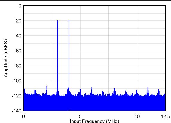
FIG 6-23. Two Tone FFT at F_{IN} = 3, 4\text{ MHz}
