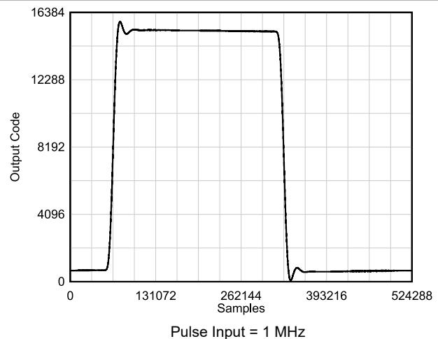
FIG 6-58. Pulse Response
