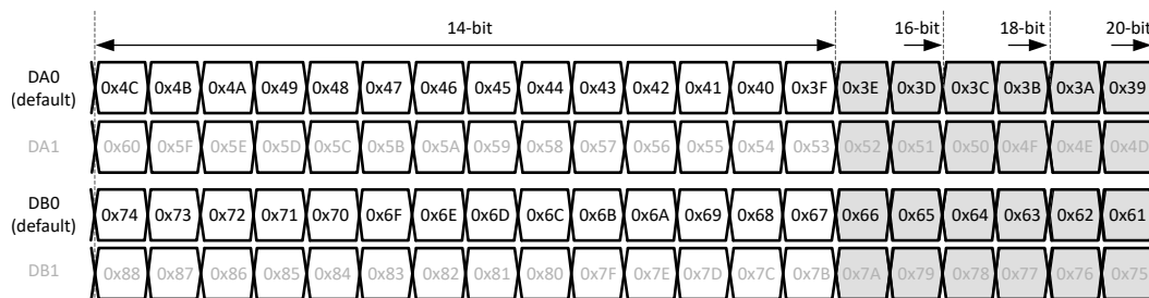
Figure 8-47. 1-wire output bit mapping
