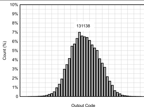
FIG 6-61. DC Histogram
