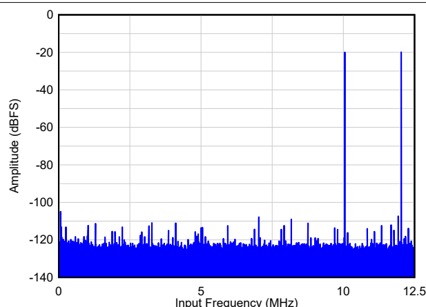
A_{IN} = -20 dBFS/line, IMD3 = 88 dBc 6-26. Two Tone FFT at F_{IN} = 10/12 MHz
