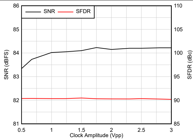
F_{IN} = 1.1 MHz 6-31. AC Performance vs Clock Amplitude
