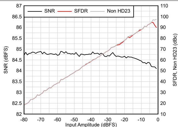
F_{IN} = 1.1 MHz 6-29. AC Performance vs Input Amplitude
