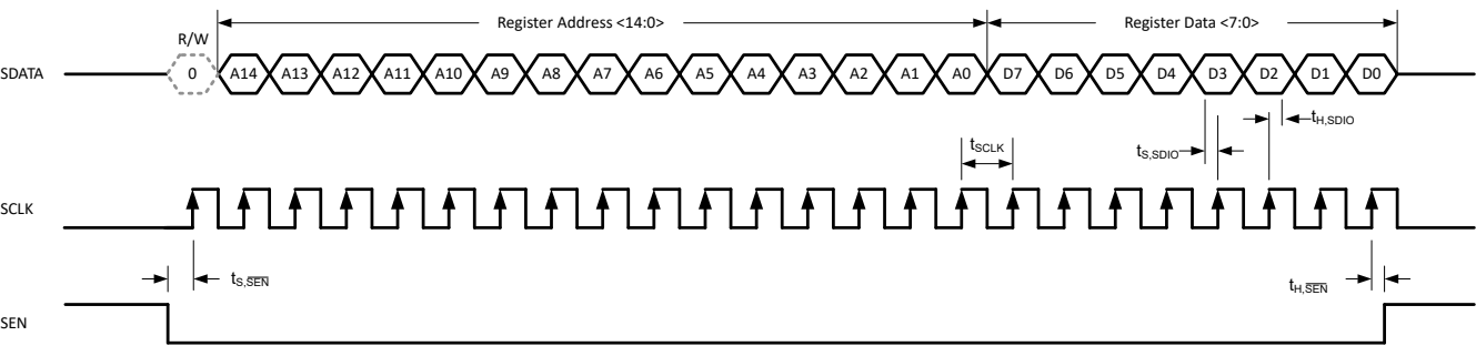
図 6-33. Serial Register Write Timing Diagram
