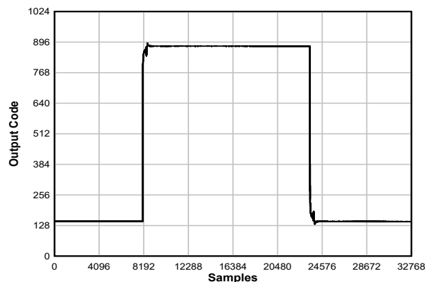
Figure 5-62. Pulse Response
