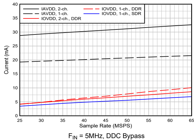
FIG 5-40. Current vs Sampling Rate
