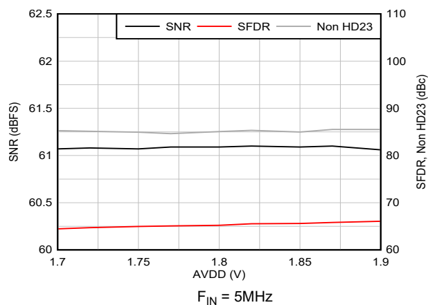
Figure 5-34. AC Performance vs AVDD
