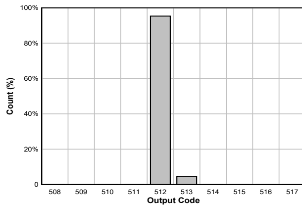
FIG 5-38. DC Offset Histogram
