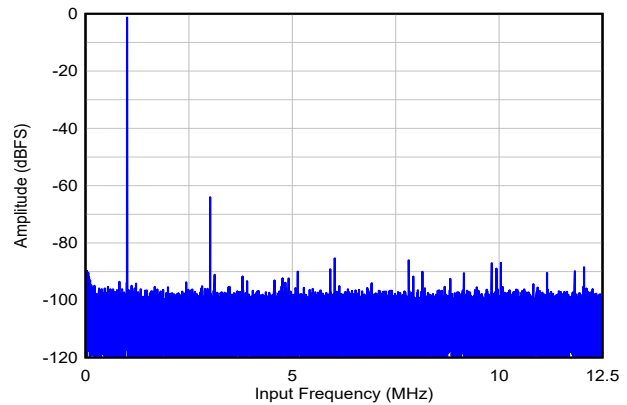
図 5-6. Single Tone FFT at F_{IN} = 1\text{MHz} , Single-ended Input
