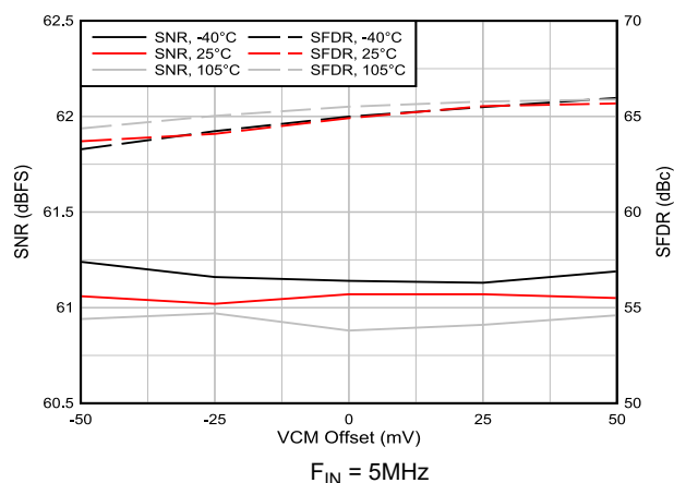
Figure 5-35. AC Performance vs VCM vs Temperature
