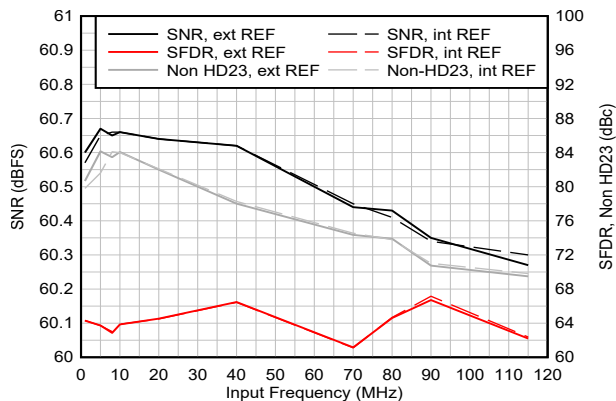
図 5-53. AC Performance vs Input Frequency
