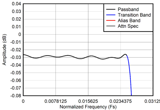
6-19. Decimation by 16 passband ripple response
