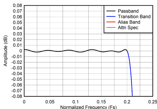
図 6-13. Decimation by 2 passband ripple response
