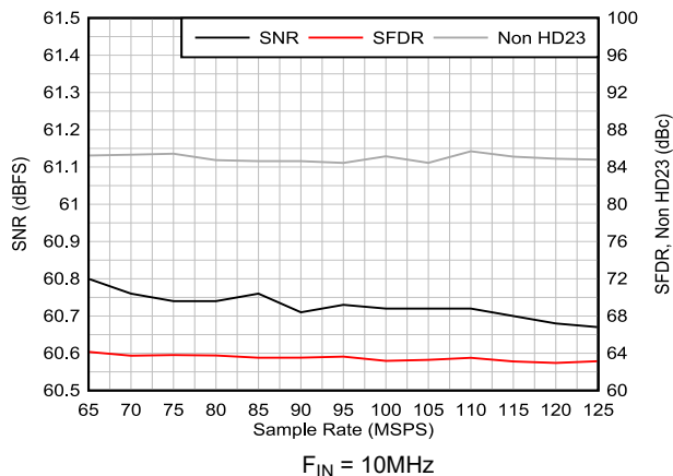
図 5-55. AC Performance vs Sampling Rate
