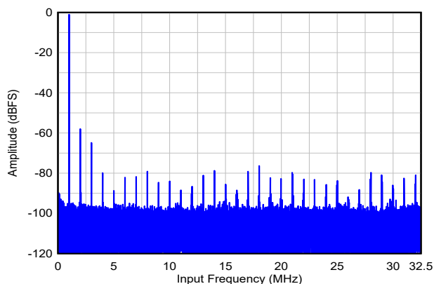
図 5-25. Single Tone FFT at F_{IN} = 1\text{MHz} , Single-ended input
