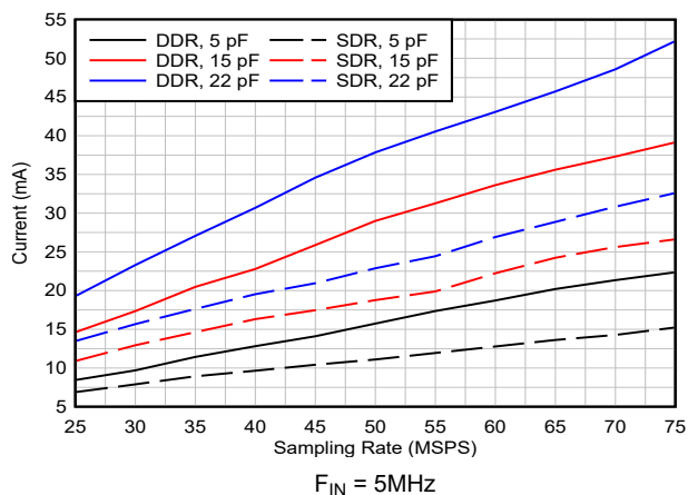
图 5-43. I_{OVDD} Current vs Load Capacitance
