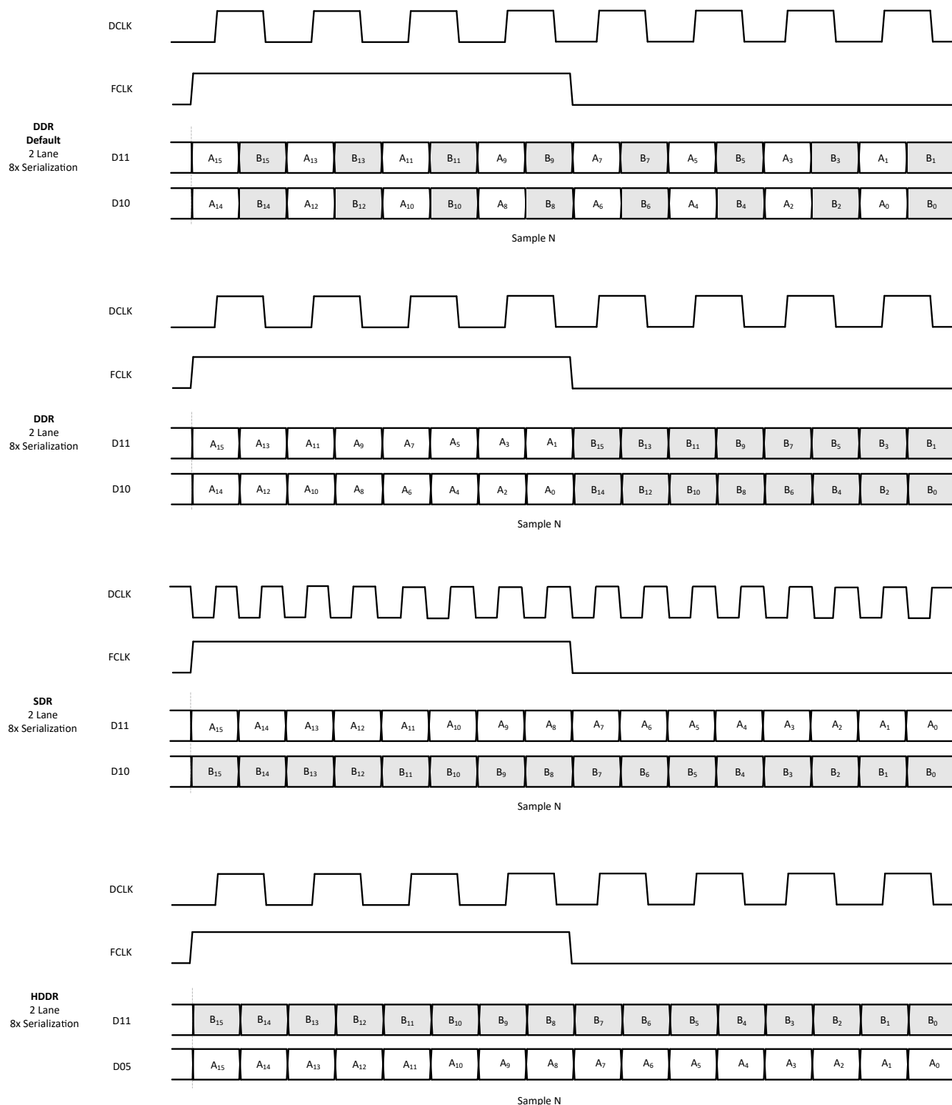
図 6-23. 16 Bit, 2 Lanes, 8x Serialization
