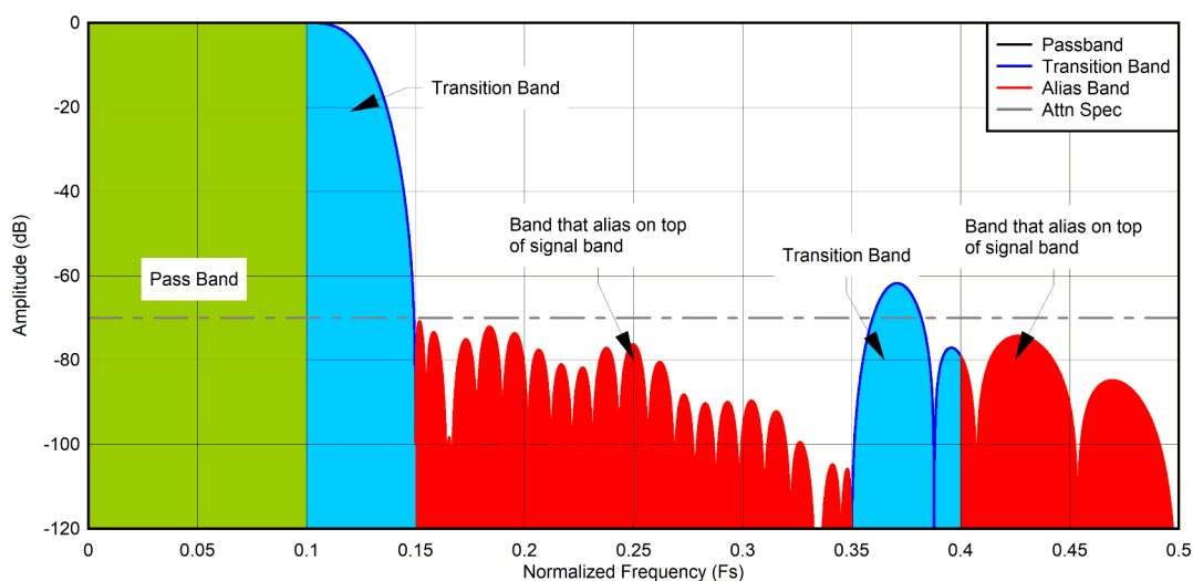
図 6-11. Interpretation of the Decimation Filter Plots
