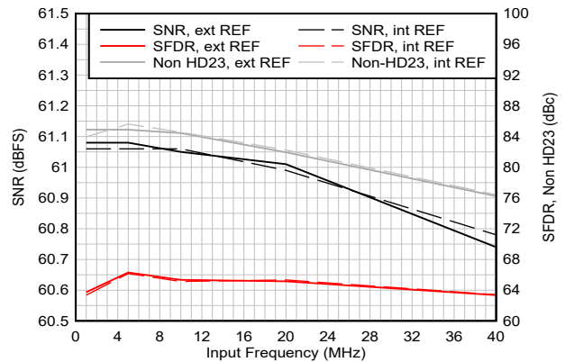
図 5-10. AC Performance vs Input Frequency
