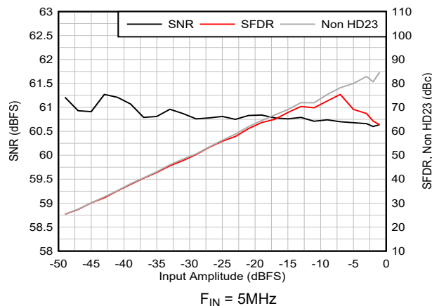
図 5-54. AC Performance vs Input Amplitude
