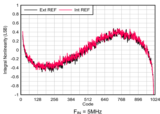
Figure 5-16. INL vs ADC Code
