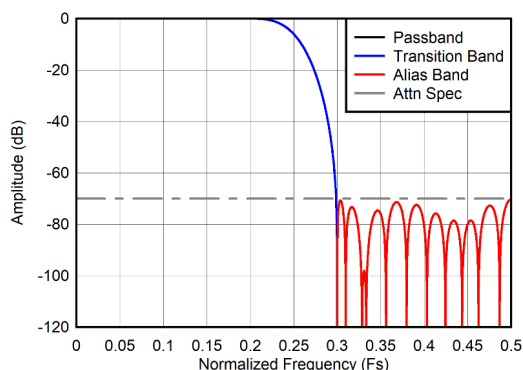
図 6-12. Decimation by 2 frequency response
