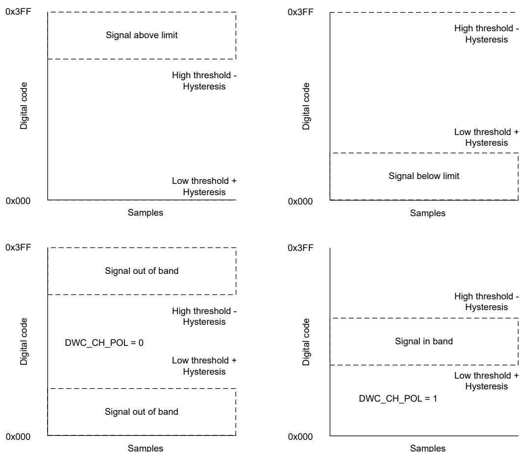
図 6-26. Digital Comparator Event Monitoring
