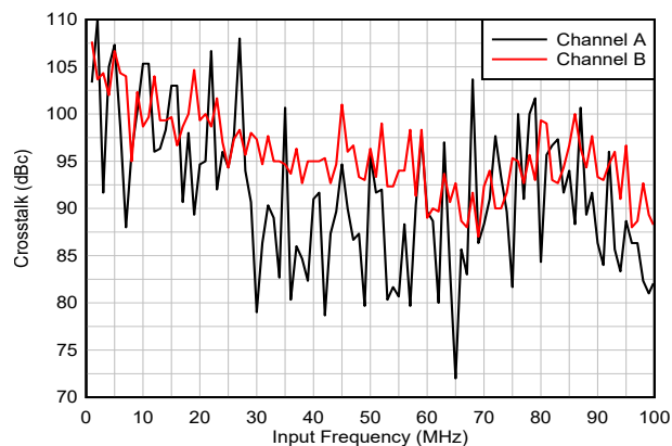
Figure 5-33. Crosstalk vs Input Frequency
