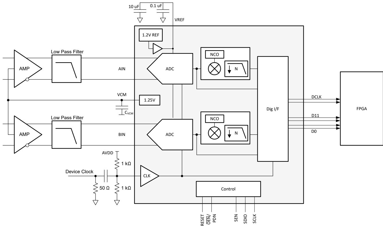
図 7-1. Typical configuration for a spectrum analyzer with DC support
