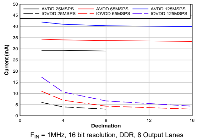
FIG 5-41. Current vs Decimation
