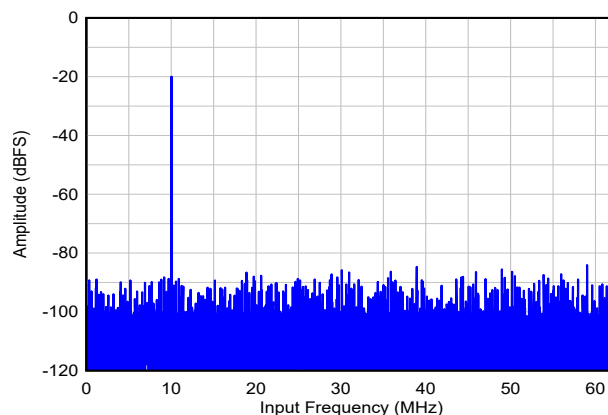
図 5-45. Single Tone FFT at F_{IN} = 10\text{MHz} , A_{IN} = -20\text{dBFS}
