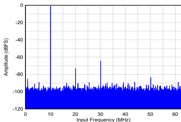
図 5-44. Single Tone FFT at F_{IN} = 10\text{MHz}
