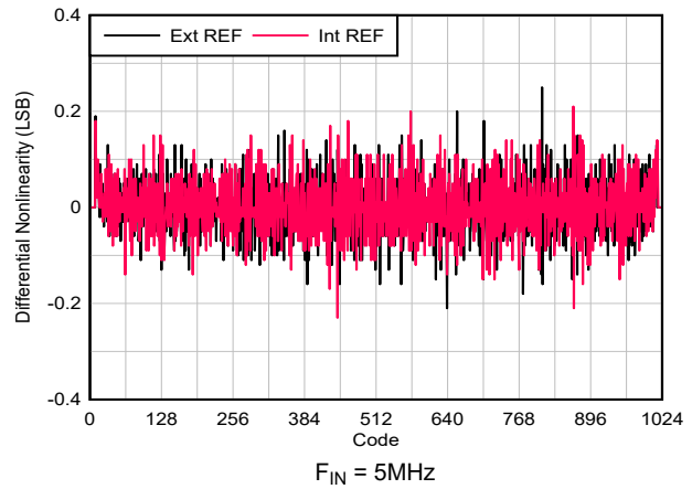
FIG 5-37. DNL vs ADC Code
