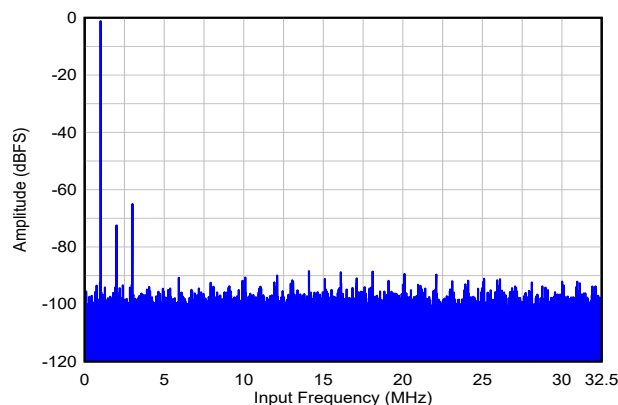
図 5-24. Single Tone FFT at F_{IN} = 1\text{MHz}
