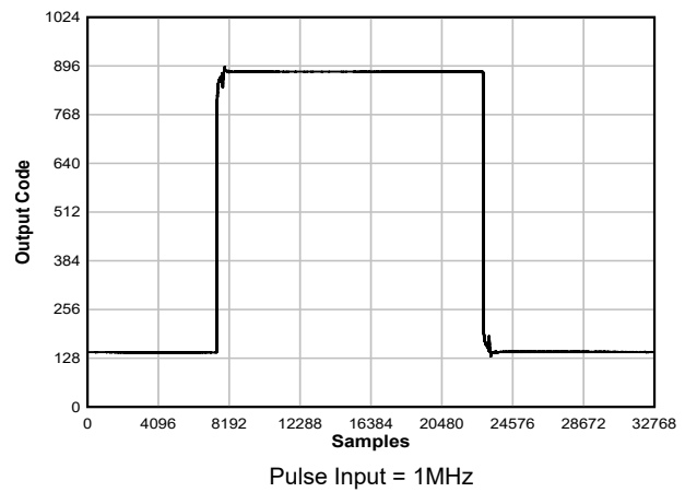
FIG 5-39. Pulse Response
