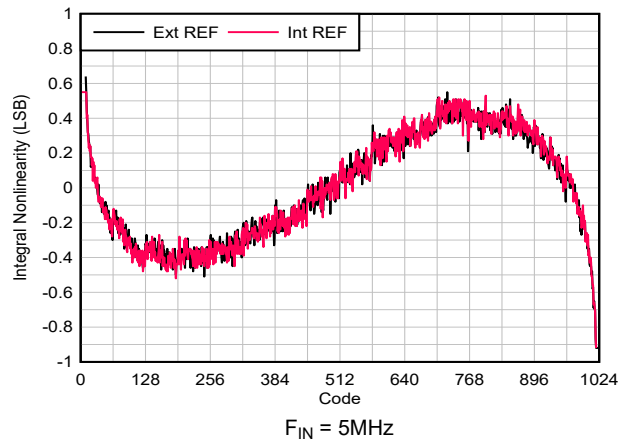
FIG 5-36. INL vs ADC Code
