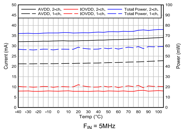
图 5-42. Current vs Temperature
