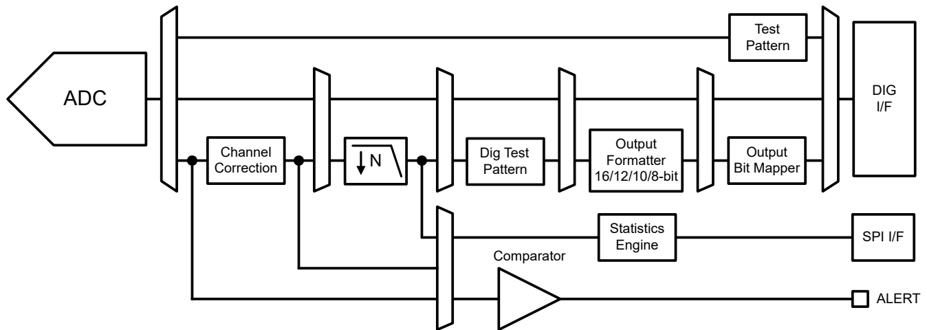
図 6-1. Digital features block diagram
