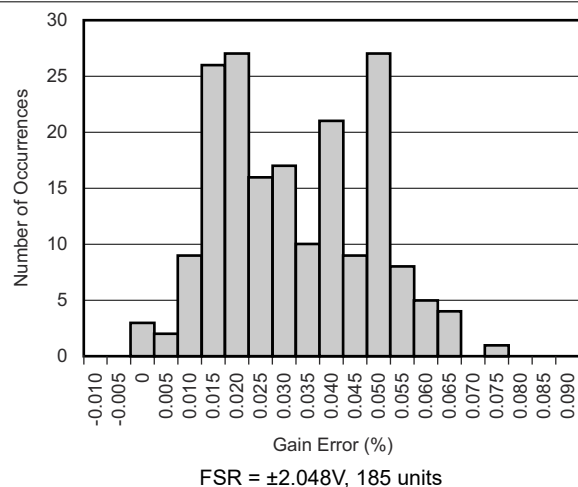
5-17. Gain Error Histogram
