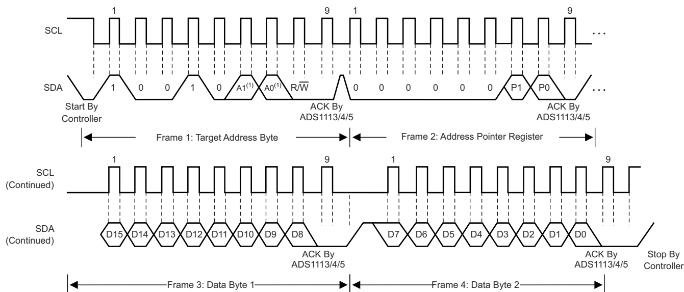
図 7-10. Timing Diagram for Writing to the ADS111x
