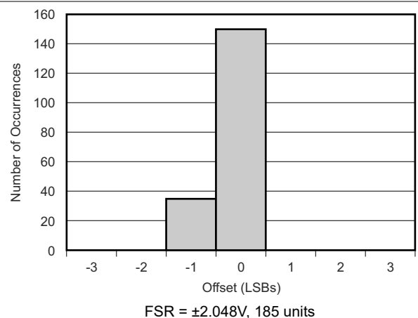
5-18. Offset Histogram
