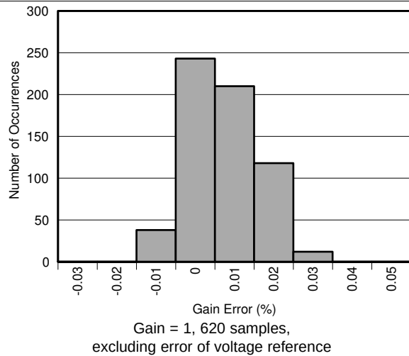
FIG 10. Gain Error Histogram
