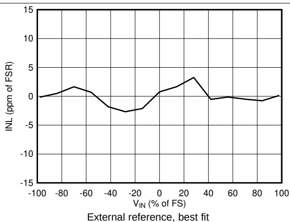
FIG 6. INL vs Differential Input Voltage
