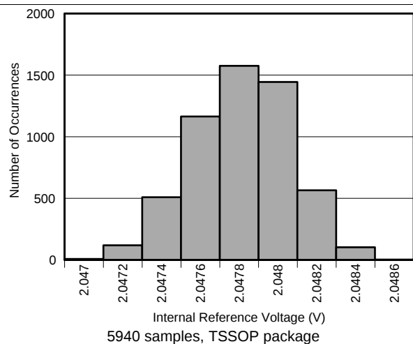
Figure 26. Internal Reference Voltage Histogram
