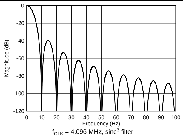
图 70. Sinc 3 Filter Frequency Response, Data Rate = 10 SPS
