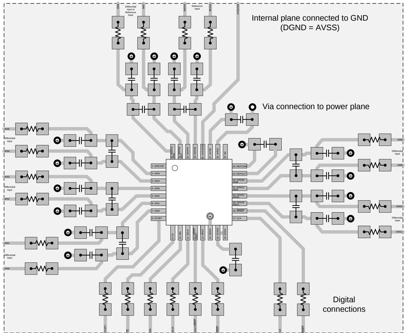
✎ 121. ADS114S0x Layout Example
