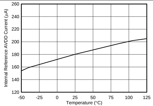
FIG 45. Internal Reference AVDD Current vs Temperature
