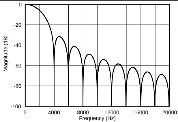
図 67. Low-Latency Filter Frequency Response, Data Rate = 2 kSPS
