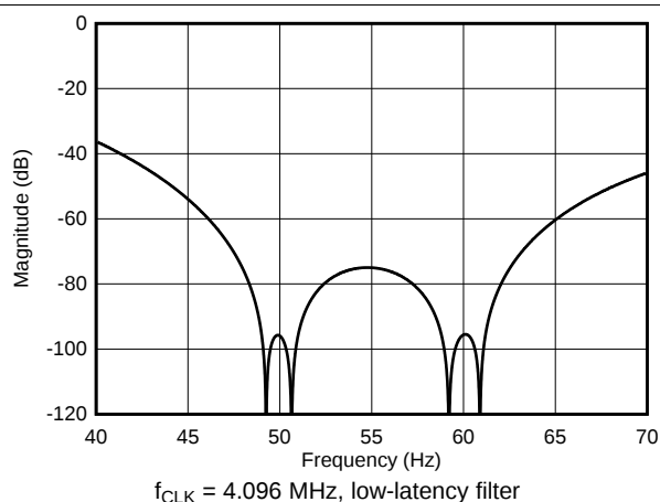
Figure 59. Low-Latency Filter Frequency Response, Data Rate = 20 SPS, Zoomed to 50 Hz and 60 Hz
