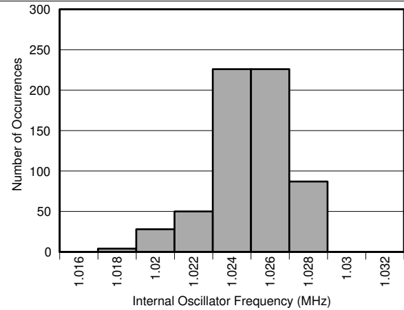
FIG 17. Internal Oscillator Frequency Histogram
