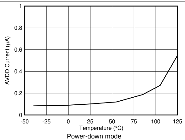
FIG 21. Analog Supply Current vs Temperature
