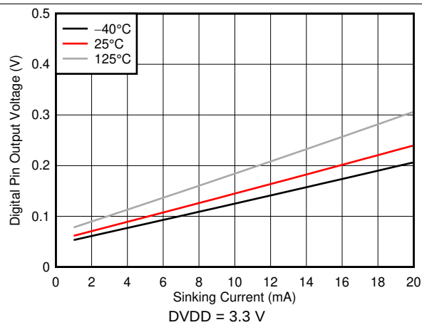
FIG 20. Digital Pin Output Voltage vs Sinking Current
