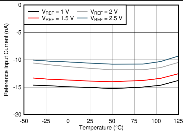
FIG 16. External Reference Input Current vs Temperature
