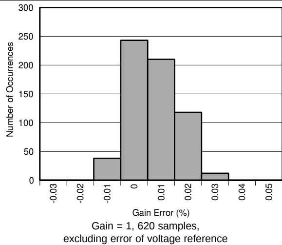
FIG 10. Gain Error Histogram
