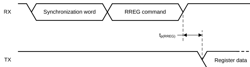
✎ 5. Register Read Switching Characteristics
