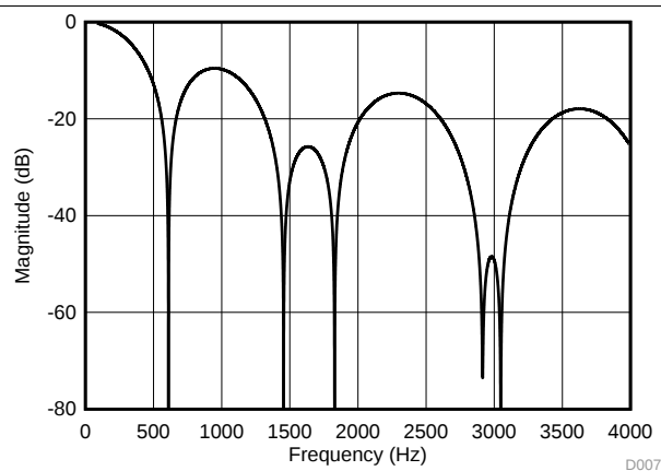
FIG 54. Filter Response (Normal Mode, DR = 600 SPS)
