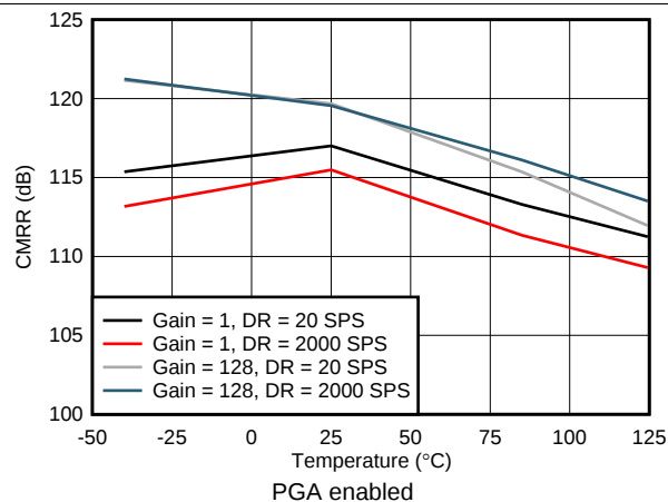
25. DC CMRR vs Temperature
