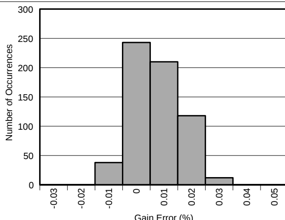
FIG 19. Gain Error Histogram
