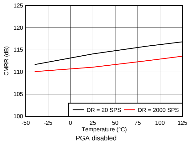
24. DC CMRR vs Temperature
