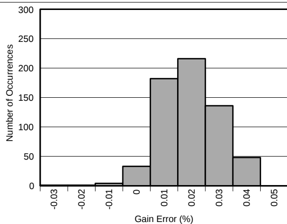
FIG 19. Gain Error Histogram
