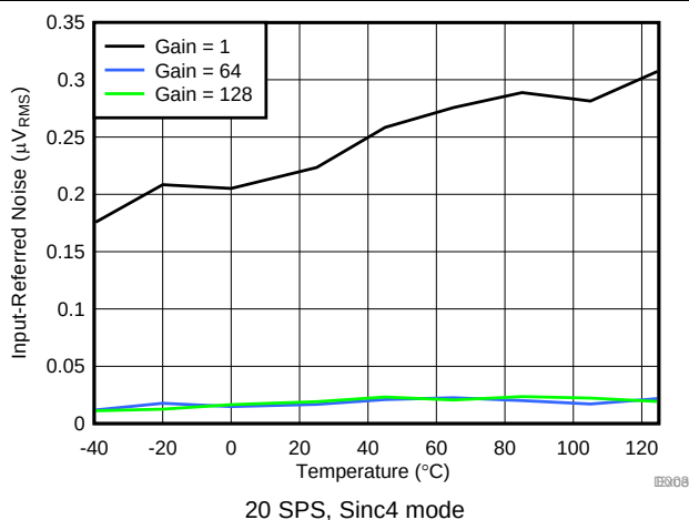
FIG 17. Noise vs Temperature
