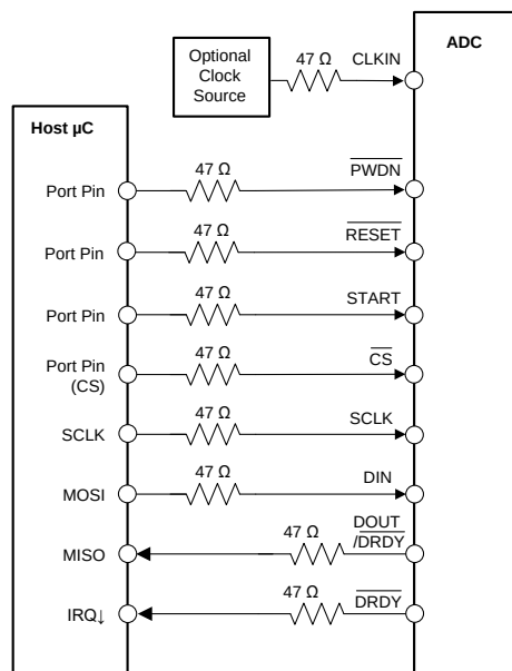
83. Serial Interface and Digital I/O Connections
