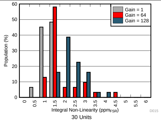
图 24. Integral Non-Linearity Distribution
