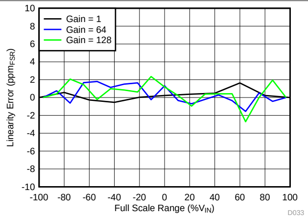
图 22. Integral Non-Linearity vs V_{IN}
