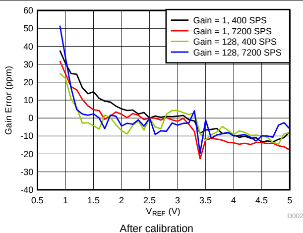
FIG 16. Gain vs Reference Voltage
