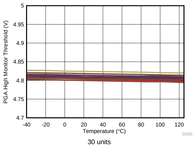
FIG 36. PGA High Monitor Threshold vs Temperature
