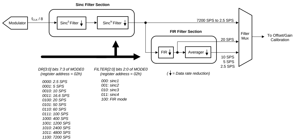
Figure 48. Digital Filter Block Diagram
