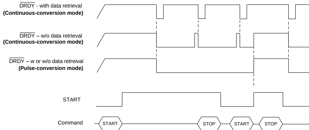
Figure 61. \overline{\text{DRDY}} Operation
