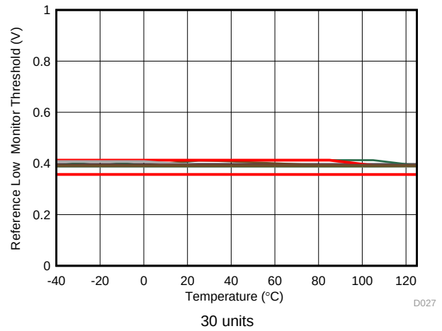
FIG 34. Reference Low Monitor Threshold vs Temperature
