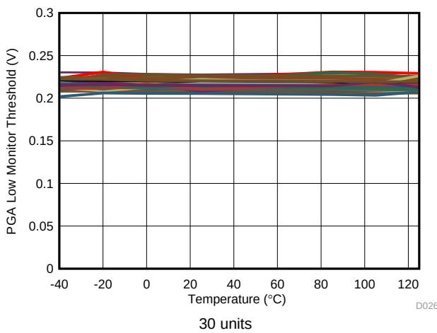
FIG 35. PGA Low Monitor Threshold vs Temperature
