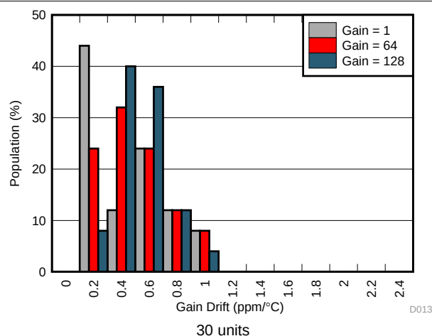
FIG 15. Gain Drift Distribution
