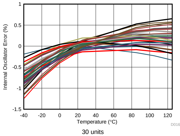
FIG 33. Internal Oscillator Frequency vs Temperature
