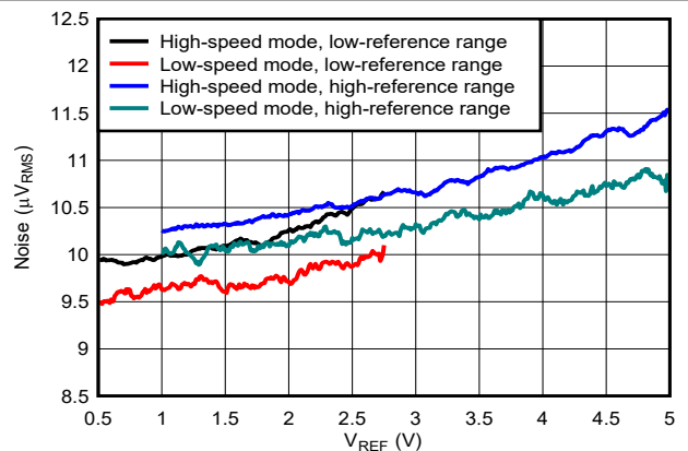
Shorted input, wideband filter, OSR = 32
