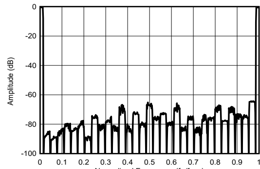
Figure 8-11. Wideband Filter Stop-Band Attenuation
