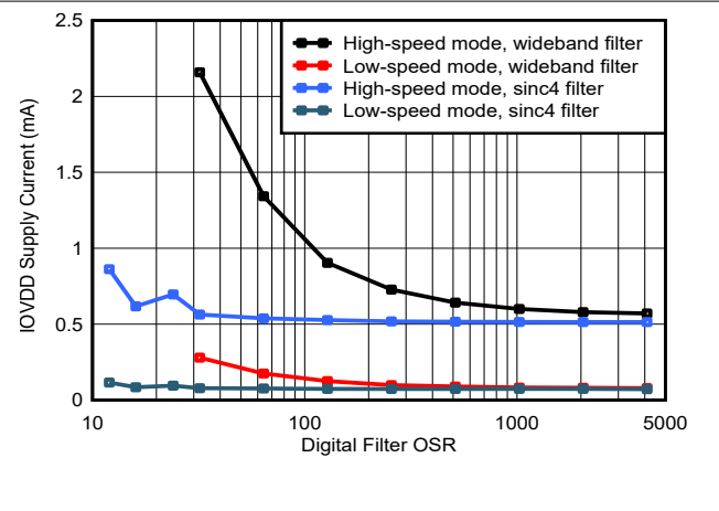
6-63. Power-Supply Current vs Oversampling Ratio
