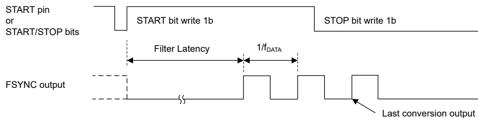
図 7-27. Start/Stop Control Mode
