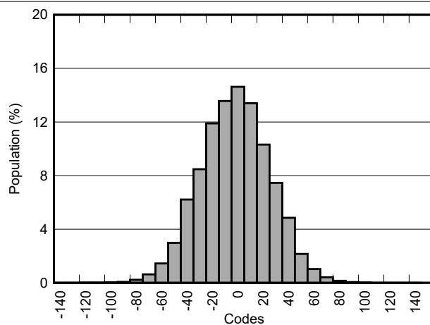
图 5-17. High-Speed Mode, Shorted FFT
