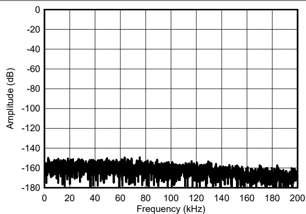
图 5-17. High-Speed Mode, Shorted FFT
