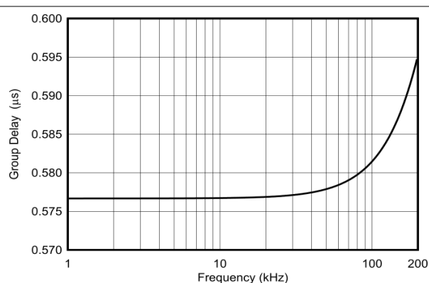
☒ 9-3. Antialias Filter Group Delay
