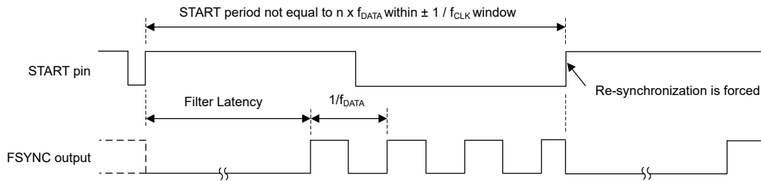
図 7-26. Synchronized Control Mode
