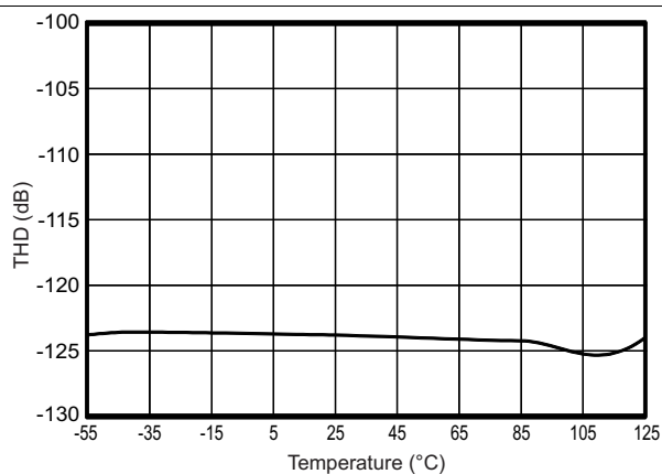
Figure 9. THD (G = 8) vs Temperature
