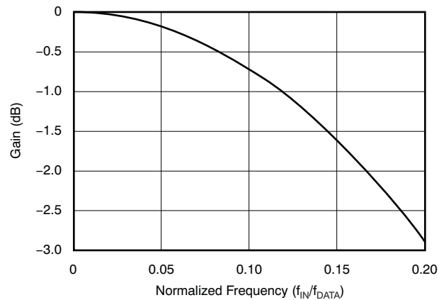
Figure 38. Sinc Filter Roll-Off
