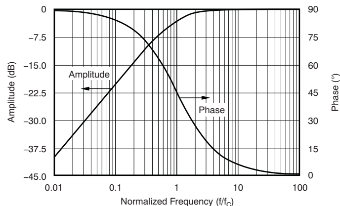
Figure 52. HPF Amplitude and Phase Response
