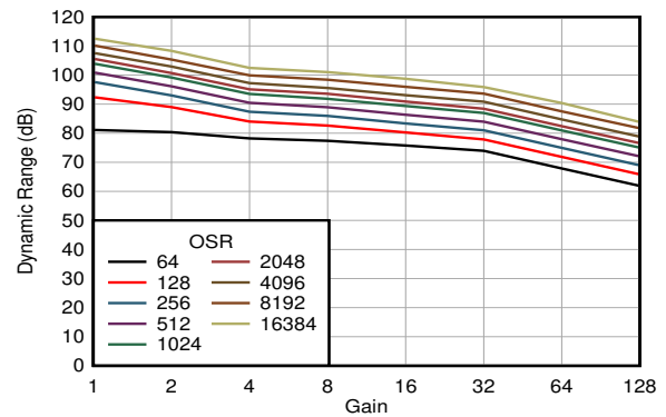
FIG 6-23. Dynamic Range at 4 kSPS vs Gain
