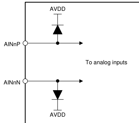
FIG 8-1. Input ESD Protection Circuitry
