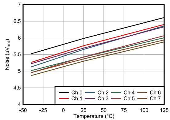
6-17. Noise vs Temperature
