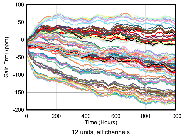
FIG 6-11. Long-Term Gain Drift (WQFN Package)
