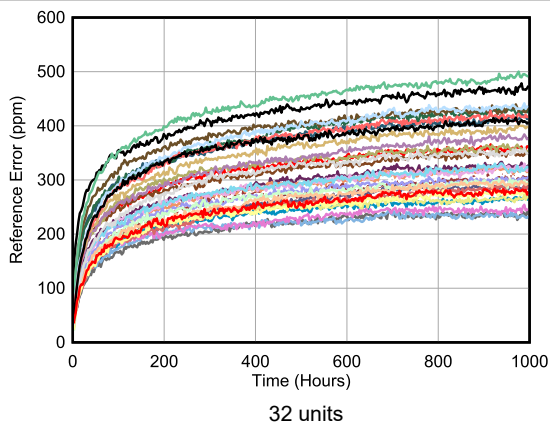
FIG 6-26. Long-Term Reference Drift (TQFP Package)
