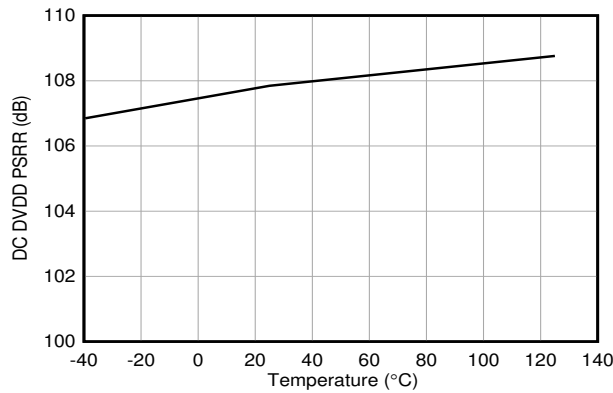
6-16. DC DVDD PSRR vs Temperature
