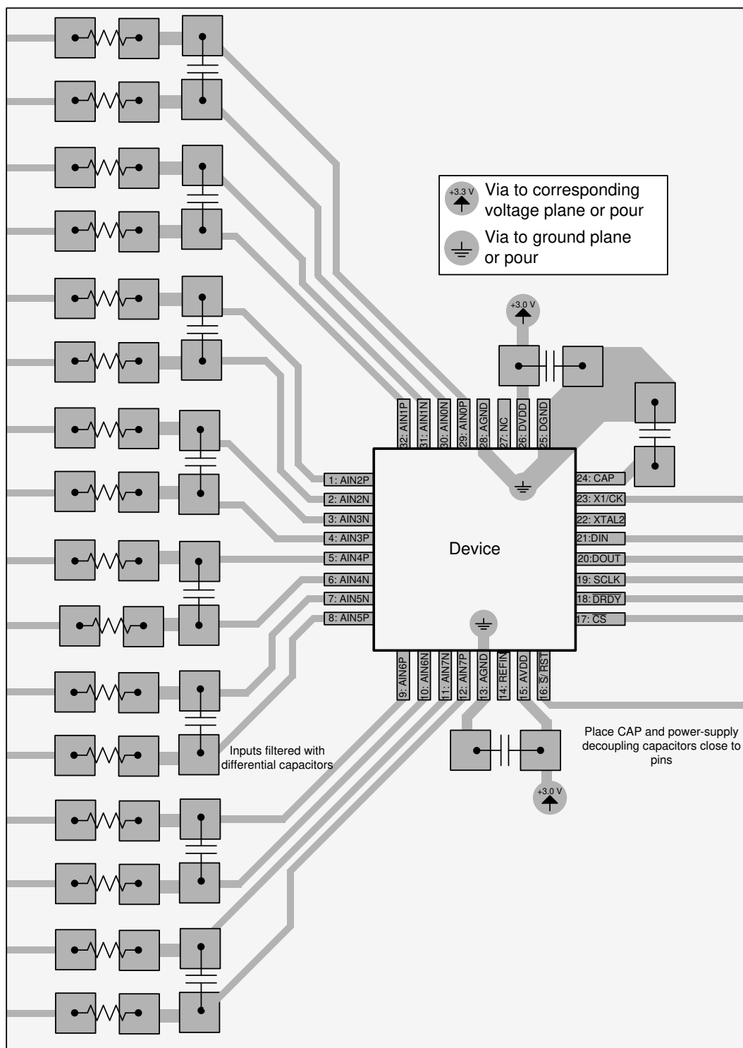
Figure 11-1. Layout Example
