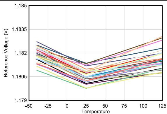
FIG 6-29. Internal Reference Voltage Temperature Drift
