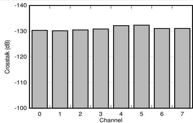
FIG 6-23. Crosstalk vs Channel
