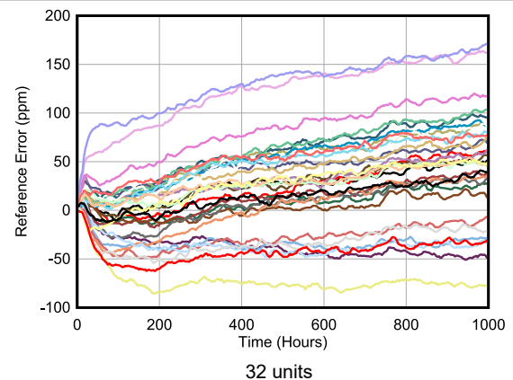
FIG 6-27. Long-Term Reference Drift (WQFN Package)
