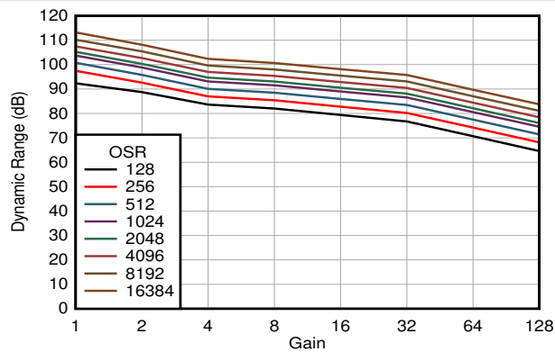
FIG 6-22. Dynamic Range vs Gain Across OSR
