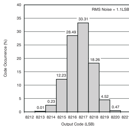
Figure 7-69. Output Noise Histogram (With Inputs Shorted to VCM)
