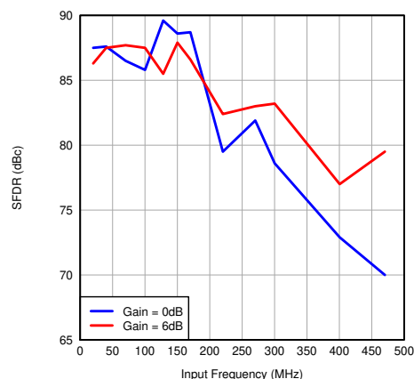
7-91. SFDR vs Input Frequency
