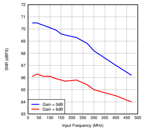
7-75. SNR vs Input Frequency
