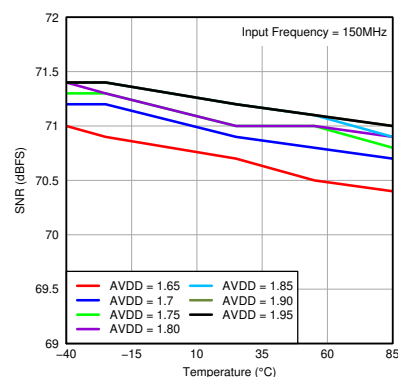
7-21. SNR vs Temperature and AVDD Supply
