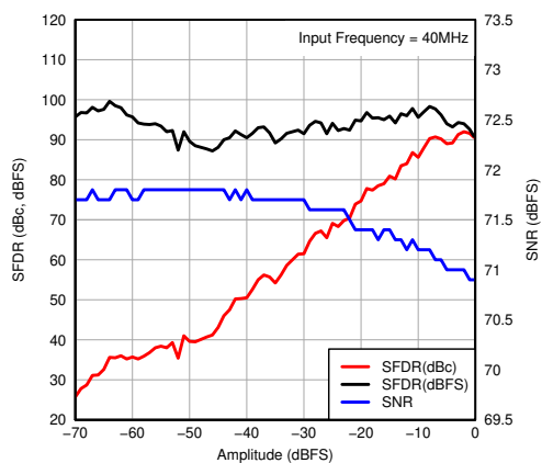
7-114. Performance vs Input Amplitude
