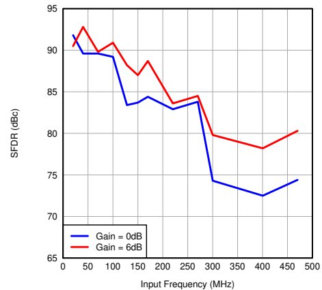
7-109. SFDR vs Input Frequency
