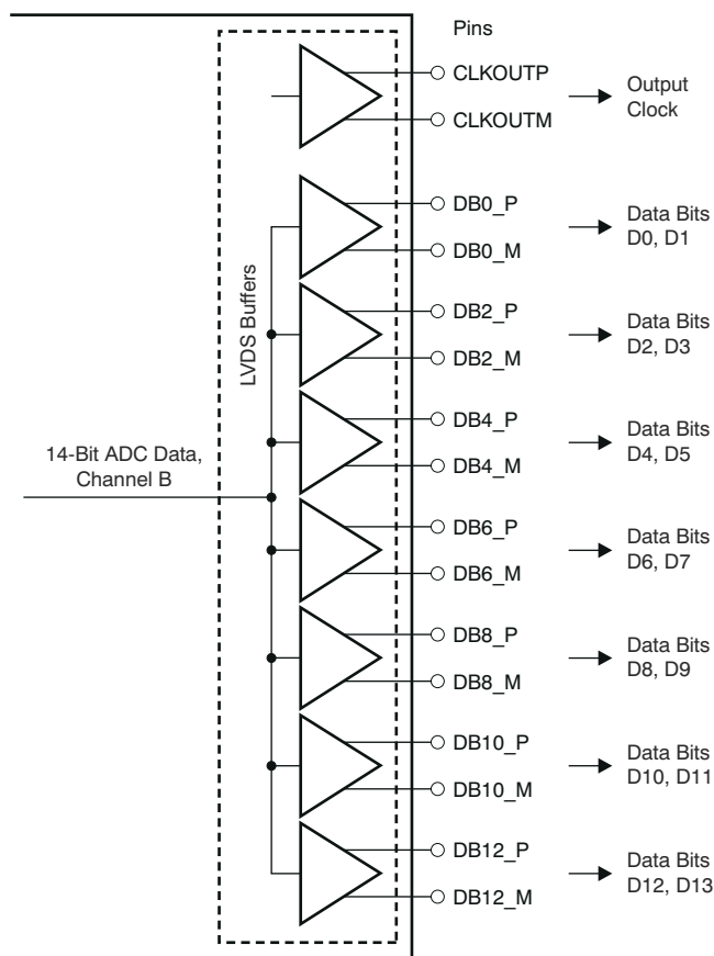
8-20. LVDS Interface
