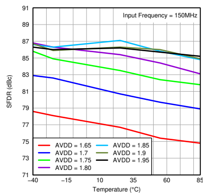
7-41. SFDR vs Temperature and AVDD Supply
