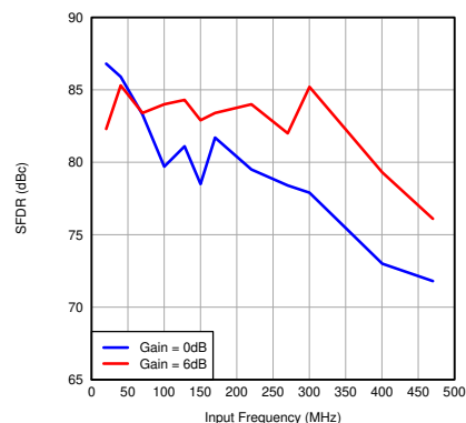
7-11. SFDR vs Input Frequency
