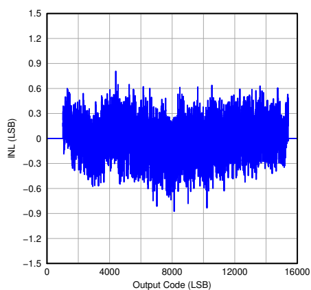
Figure 7-68. Integrated Nonlinearity
