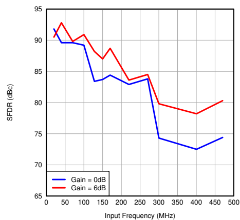
7-53. SFDR vs Input Frequency
